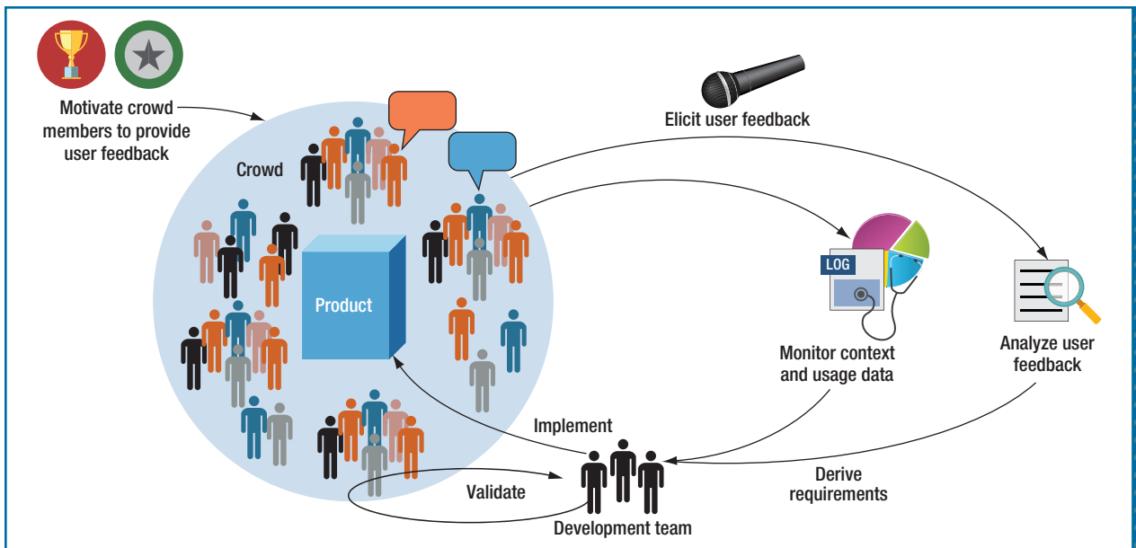
FIGURE 1. The relationships among the aspects of crowd-based requirements engineering (CrowdRE). CrowdRE strives to mobilize as many crowd members as possible to communicate and discuss their needs regarding the evolution of existing software products.
