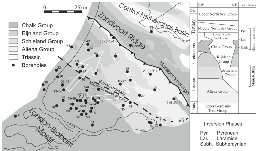
Fig. 10 General pattern of erosion in the West Netherlands Basin (for data see Table 1). Well numbers are the same as in Table 1. Background map represents the pre-Tertiary outcrop pattern. White arrows indicate the direction of increasing erosion
