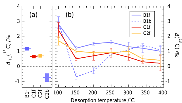
Figure 6. \Delta(^{13}\text{C}) values of alpha-pinene SOA filter samples. Full lines represent front filters, and dashed lines back filters. Error bars denote 1- \sigma standard deviations and are propagated; they vary with loading. (a) TC analysis of selected filters (see x axis). (b) Thermal desorption analysis of filter material.
