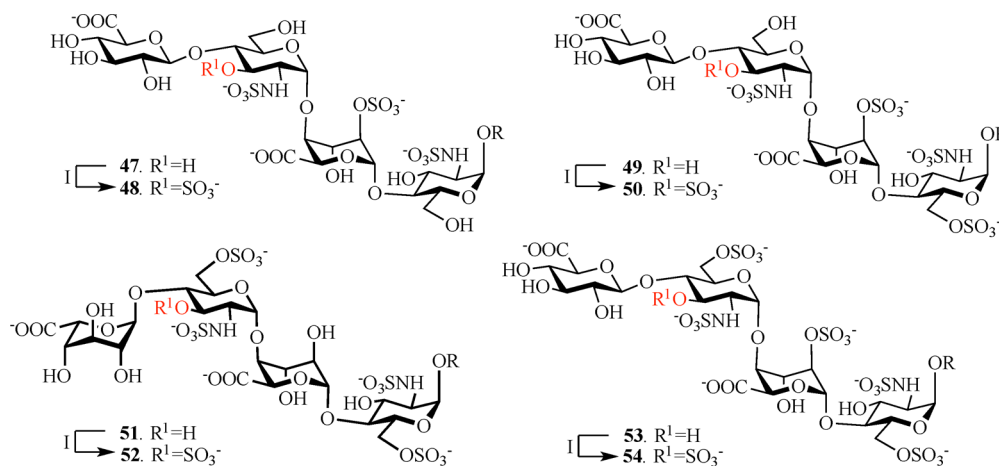
Scheme 2. Tetrasaccharide Substrates for 3-OST1 and Their Modified Products a
