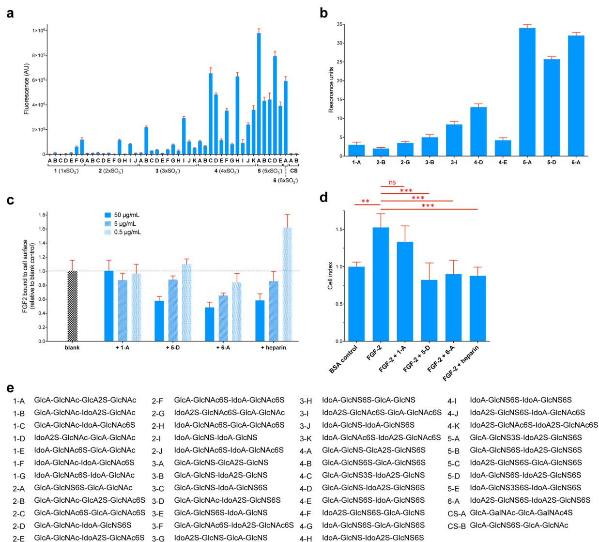
Figure 2. Binding of synthetic heparan sulfate oligosaccharides to FGF-2. (a) Binding of FGF-2 (0.5 µg/mL) to the HS oligosaccharide microarray at 1 mM ( n = 6 ). (b) SPR binding of immobilized FGF-2 to various tetrasaccharides (100 µM) used as analytes. (c) Inhibition of FGF-2 binding to mouse endothelium cell surface by various tetrasaccharides and heparin measured in real time by an xCELLigence RTCA DP system. (d) Inhibition of FGF-2 induced cell proliferation by various tetrasaccharides and heparin measured in real time by an xCELLigence RTCA DP system. Asterisks indicate statistically significant difference (** P < 0.01 , *** P < 0.001 ) and ns indicates no significant difference. Bar graphs in panels a-d represent the mean \pm SD. (e) Compound numbering and structures of the tetrasaccharide library.
