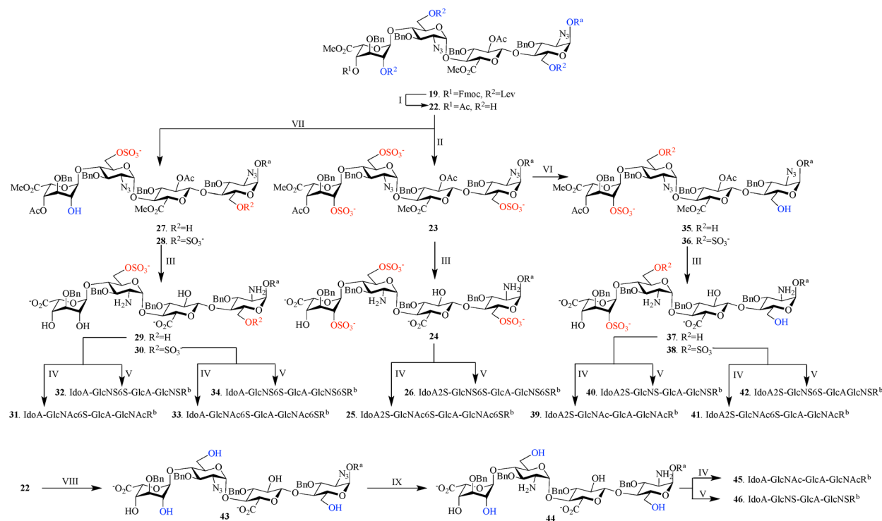
Scheme 1. Diversification of Tetrasaccharide 18 a
