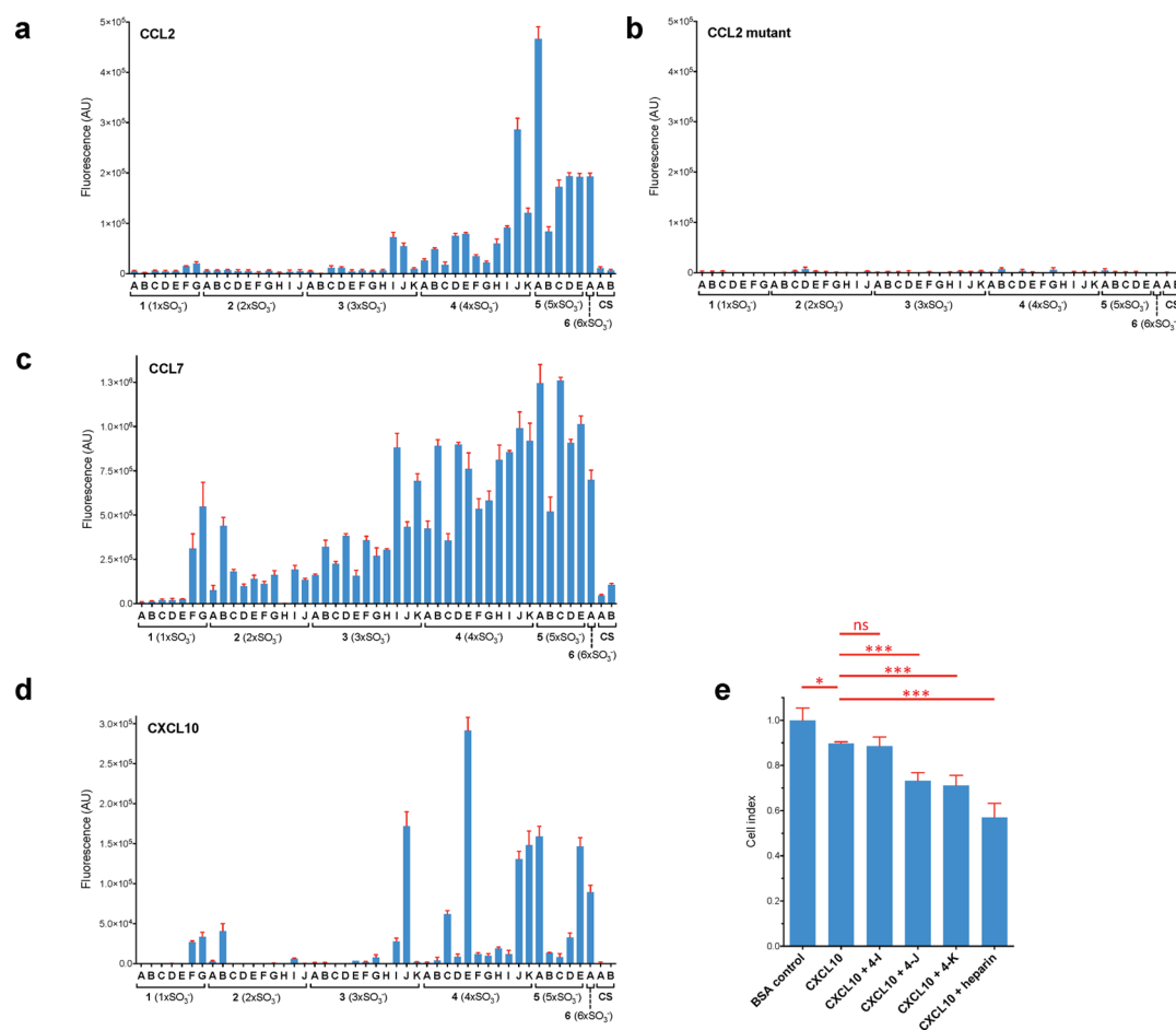
Figure 3. Binding of different HS-binding proteins to the HS oligosaccharide microarray and subsequent biological examination. Microarray results of synthetic heparin sulfate tetrasaccharide library at 1 mM with (a) CCL2 (0.5 \mu\text{g}/\text{mL} ); (b) CCL2 mutant R18AK19A (0.5 \mu\text{g}/\text{mL} ; shown at same scale as CCL2); (c) CCL7 (1 \mu\text{g}/\text{mL} ); and (d) CXCL10 (0.5 \mu\text{g}/\text{mL} ). (e) Effect of various tetrasaccharides on the inhibition of CXCL10 on cell proliferation. Asterisks indicate statistically significant difference (* P < 0.05 , *** P < 0.001 ) and ns indicates no significant difference. Bar graphs in panels a–e represent the mean \pm SD.
