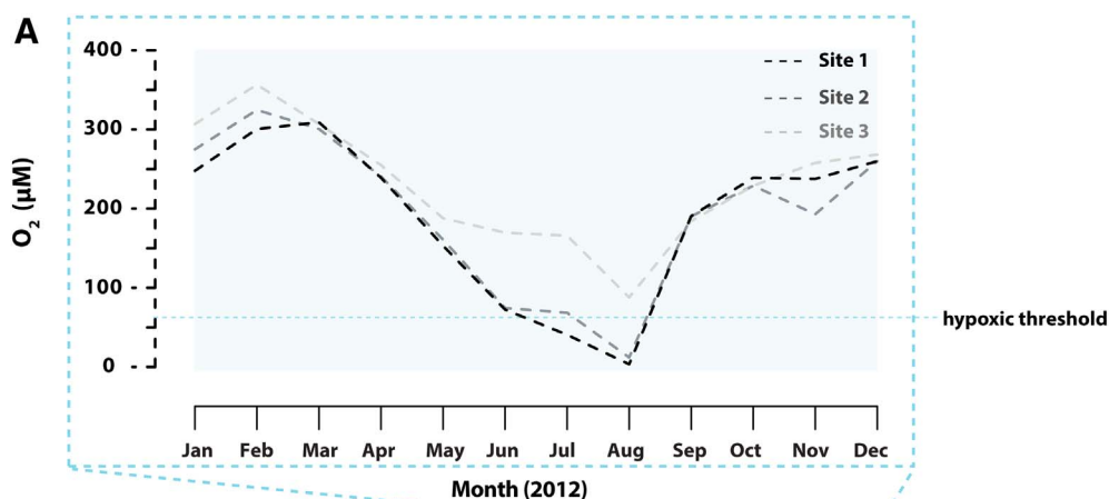
Fig. 2. (A) Monthly bottom-water oxygen concentrations (in \mu\text{M} ) at all three sites from January to December 2012. The horizontal line refers to the threshold for hypoxia ( \text{O}_2 = 62.5 \mu\text{M} ) (B) Periods of oxic, hypoxic and anoxic bottom-water conditions from 1999 to 2011 at site 1 (Ministry of Infrastructure and Environment (Wetsteyn, 2011)).
