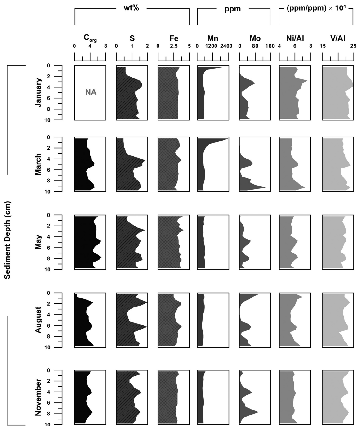
Fig. 5. Sediment profiles of C_{org} , total S, Fe, Mn, Mo, Ni/Al and V/Al for January, March, May, August and November 2012 at site 1. Nickel and vanadium are normalised to aluminium to account for the high background concentration in clays (Wedepohl, 1991). Sediment profiles of Mo/Al are provided in Fig. S4. Data are provided in Table S4.
