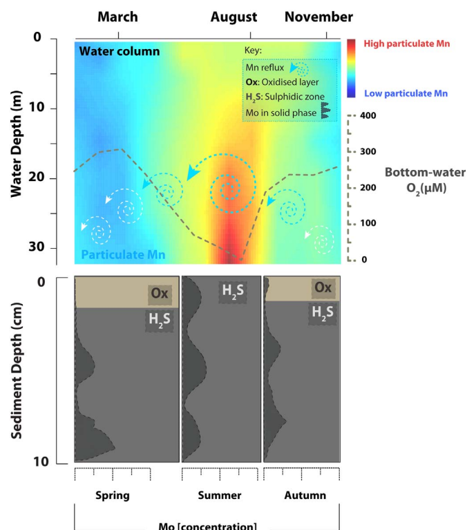
Fig. 11. Schematic of Mo and Mn dynamics in the sediment and water column at site 1 in spring, summer and late autumn. Upper panel: particulate Mn in the water column. Lower panel: schematic representation of sediment Mo profiles.
