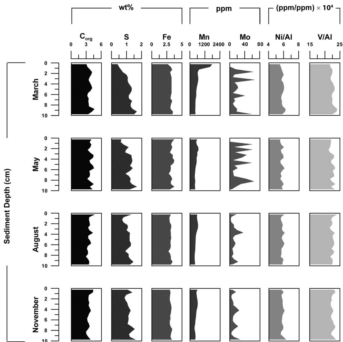
Fig. 6. Sediment profiles of C_{org} , total S, Fe, Mn, Mo, Ni/Al and V/Al for March, May, August and November 2012 at site 2. Note that site 2 was not sampled in January 2012. Data are provided in Table S4.
