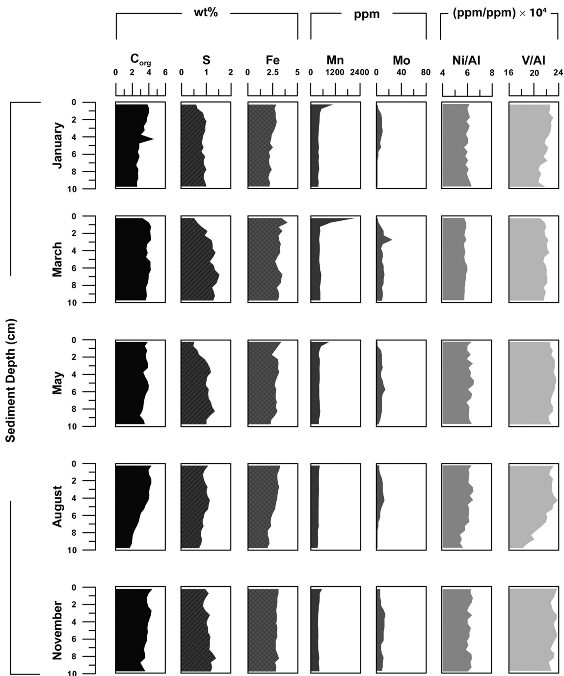
Fig. 7. Sediment profiles of C_{org} , total S, Fe, Mn, Mo, Ni/Al and V/Al for March, May, August and November 2012 at site 3. Data are provided in Table S4.
