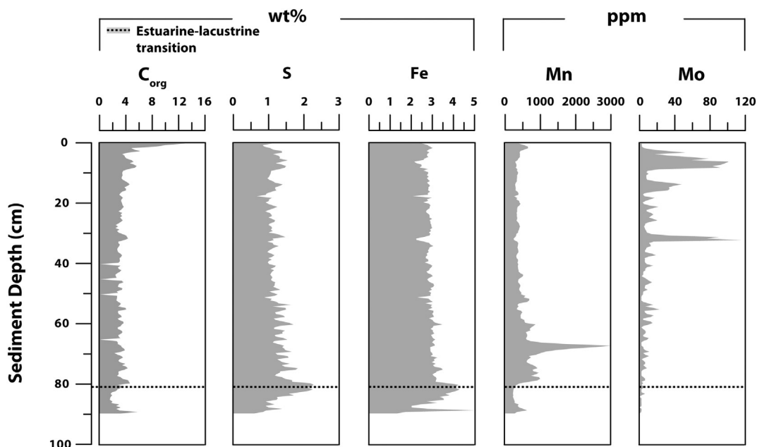
Fig. 9. Sediment profile of C_{\text{org}} , total S, Fe, Mn and Mo for the long core (90 cm) at site 1 for May 2012. The estuarine-lacustrine transition is indicated with a dotted line. Data are provided in Table S5.
