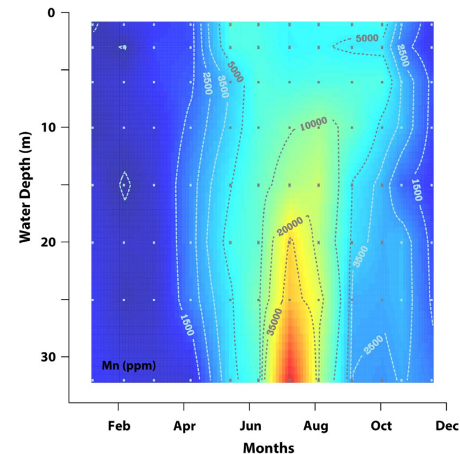
Fig. 3. Concentrations of total Mn in suspended matter (in ppm) at site 1 for 2012. Note that a similar pattern with depth and time is observed when Mn concentrations are expressed per volume of water; Fig. S3). Data are provided in Table S2.
