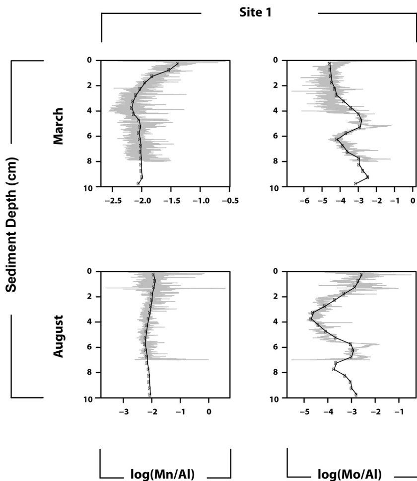
Fig. 8. Sediment profiles of \log(\text{Mn}/\text{Al}) and \log(\text{Mo}/\text{Al}) for March and August 2012 at site 1 as obtained with LA-ICP-MS (grey lines) and discrete sampling followed by total elemental analysis (black lines and dots). Data are provided in Tables S6 and S7.
