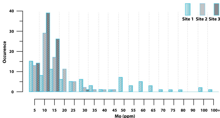
Fig. 10. Number of samples with Mo concentrations (ppm) in different concentration ranges at sites 1–3 (after Scott and Lyons, 2012). Where sulphide is present but restricted to the pore waters, sediment Mo concentrations do not typically exceed 25 ppm. Conversely, in euxinic environments where hydrogen sulphide is present in the water column throughout the year, and dissolved Mo is abundant due to effective exchange with the open ocean, enrichments display a much wider range with concentrations consistently > 100 ppm (Scott and Lyons, 2012).
