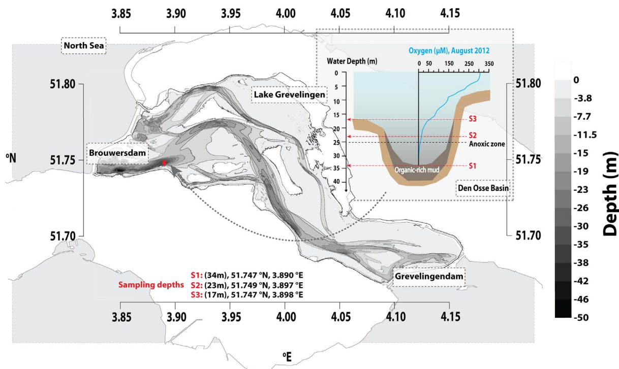
Fig. 1. Location of the Den Osse basin at the south-western edge of Lake Grevelingen. Sediment samples were collected from three sites (S1–S3) along a water depth gradient from January to December 2012 (inset). The water column oxygen concentration as a function of water depth for site 1 is plotted for the most anoxic period of the sampling year, August 2012.
