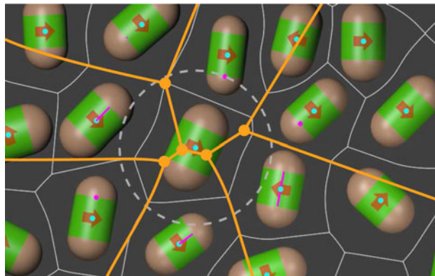
Fig. 6. Example of a local Generalized Voronoi Diagram (GVD), with points of maximal local clearance, in orange. The GVD of the crowd is shown in white. The features that define the local GVD are shown in magenta. The dashed circle shows the clearance of the agent.
