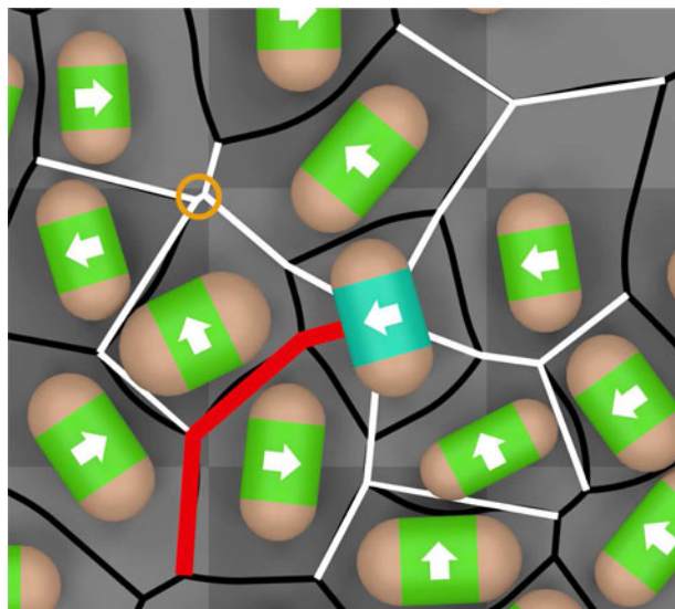
Fig. 5. Candidate paths in white lines, with the best-scoring path as a thick, red line. The circled edge was shorter than H_\epsilon . The paths are extended to the agent position. The goal position is bottom left outside the frame. Note that the paths along curved Voronoi edges are just drawn as straight line segments for simplicity.
