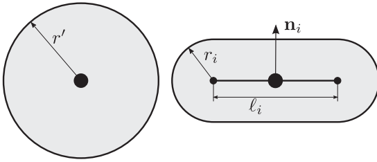
Fig. 2. Two types of crowd agent representation. On the left a common crowd agent: a point with a radius. On the right our crowd agent: a line segment with a radius.
