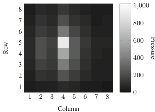
Fig. 4 Crosstalk visualization showing the sensor data of a single frame, a pencil was pressed down on the sensor grid (light pressure point) effecting the pressure level of adjacent channels
