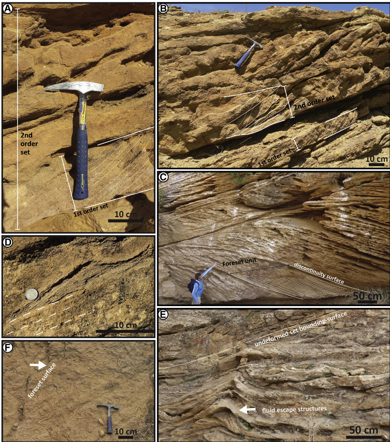
Fig. 9. (A) Relationship between different orders of cross-stratification at Ben Allou. First-order sets are small dunes prograding down the lee-side of larger dunes (2nd order sets). (B) West-migrating, medium thickness, simple cross-bedding with tabular geometry at Ben Allou A, SI-1a. (C) West-migrating, medium to large, compound cross-bedding at Ben Allou B, SI-1a. (D) Well-preserved dune over-riding a larger dune. (E) Fluid-escape structures occur in cross-sets and are capped by undeformed set-boundaries. (F) Planolites burrowing the surface of a foreset.
