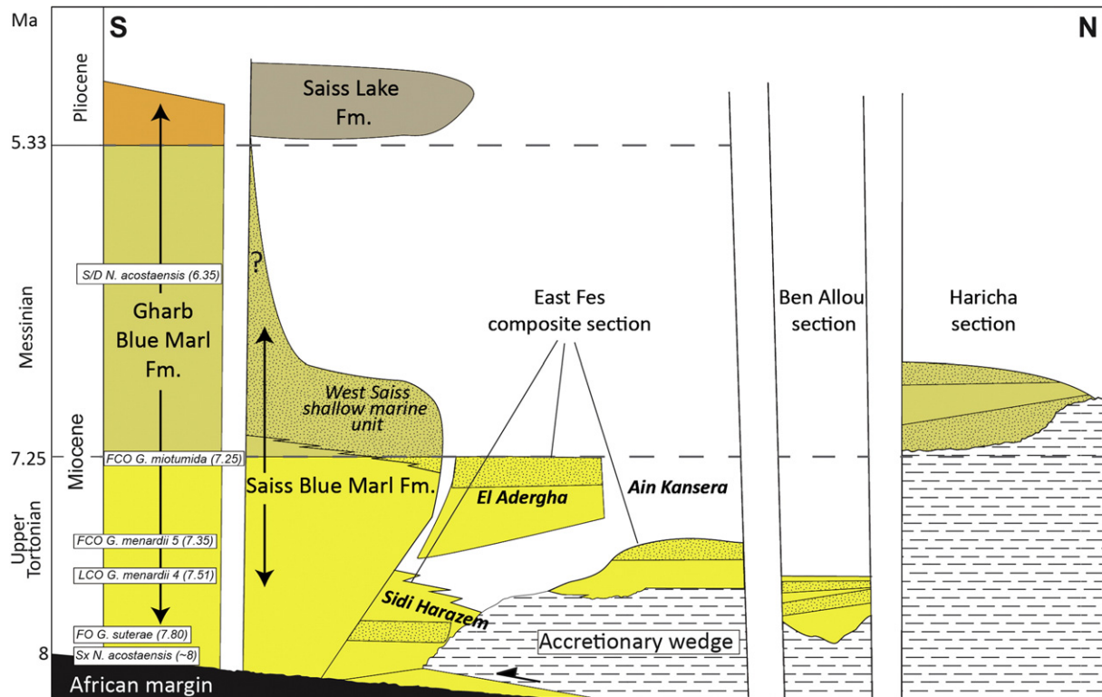
Fig. 3. Correlation diagram between the studied sections and the classic Gharb-Saiss stratigraphy. The 5 studied sections (Sidi Harazem, El Adergha, Ain Kansera, Ben Allou, and Haricha) are dated with biostratigraphy. Bioevents (left column): Sx = onset dominant sinistral; FO = first occurrence; LCO = last common occurrence; FCO = first common occurrence; S/D = coiling change from predominantly sinistral to dextral (after Lourens et al., 2004; Hilgen et al., 2012). Dotted fills depict the sand-rich parts, whereas simple colour fill broadly represents other lithologies (e.g., marlstone, limestone).
