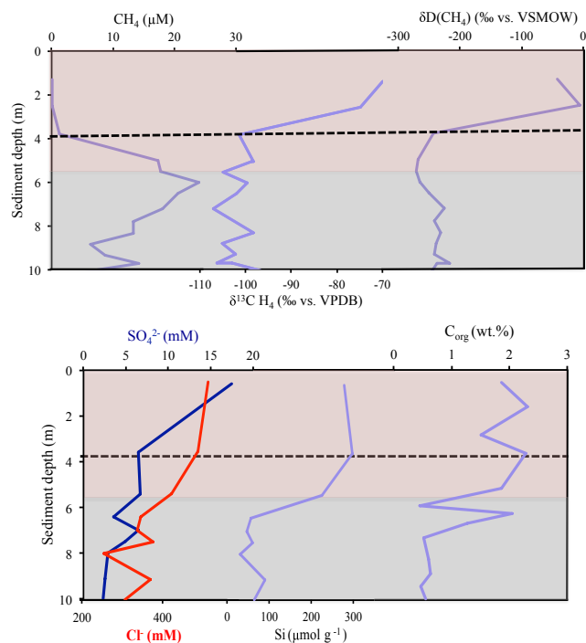
Figure 5. Close-up of the CH 4 concentration, stable isotope and other biogeochemical data of the surface of the non-ebullition sediment core ID-11, from the Buor-Khaya Bay. Red shaded area corresponds to the marine sediment deposited during the Holocene transgression and the grey shaded area corresponds to the thawed permafrost layer. The black dotted line corresponds to the depth where CH 4 oxidation starts to occur.
