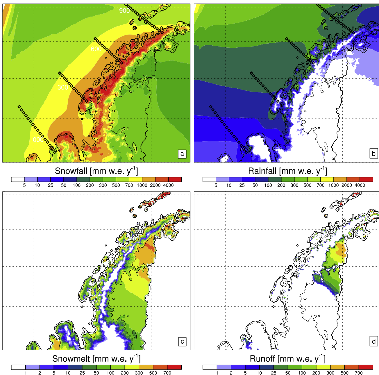
Fig. 2. Climatological (1979–2014) freshwater fluxes from RACMO2.3: snowfall (a), rainfall (b), snowmelt (c) and meltwater runoff (d) in mm w. e. y^{-1} . Note the different scales in a,b compared to c,d. Also shown in a,b are the Pal-LTER transects as used in this study.
