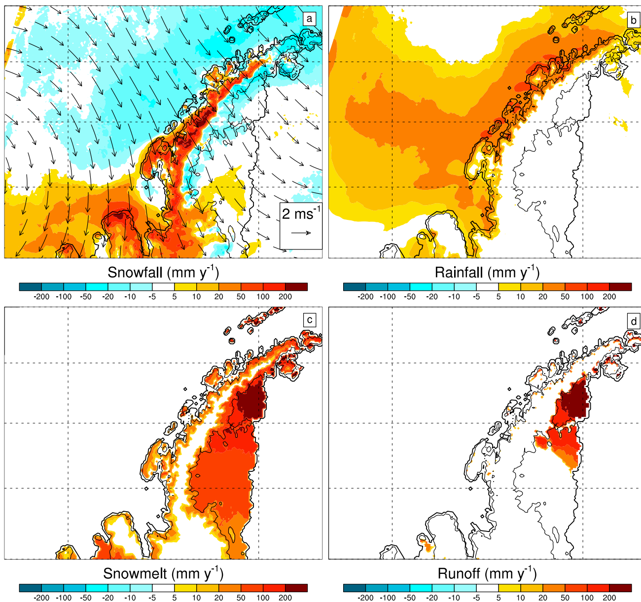
Fig. 5. Difference of the SAM+/ENSO+ composite with the climatology (1979–2014) of the summer months (Dec., Jan., Feb.) freshwater components snowfall (a), rainfall (b), snowmelt (c) and meltwater runoff (d), in mm w. e. y -1 for 1979–2014. In a) 500 hPa wind speed difference vectors are also shown. Details are found in Section 2.2.
