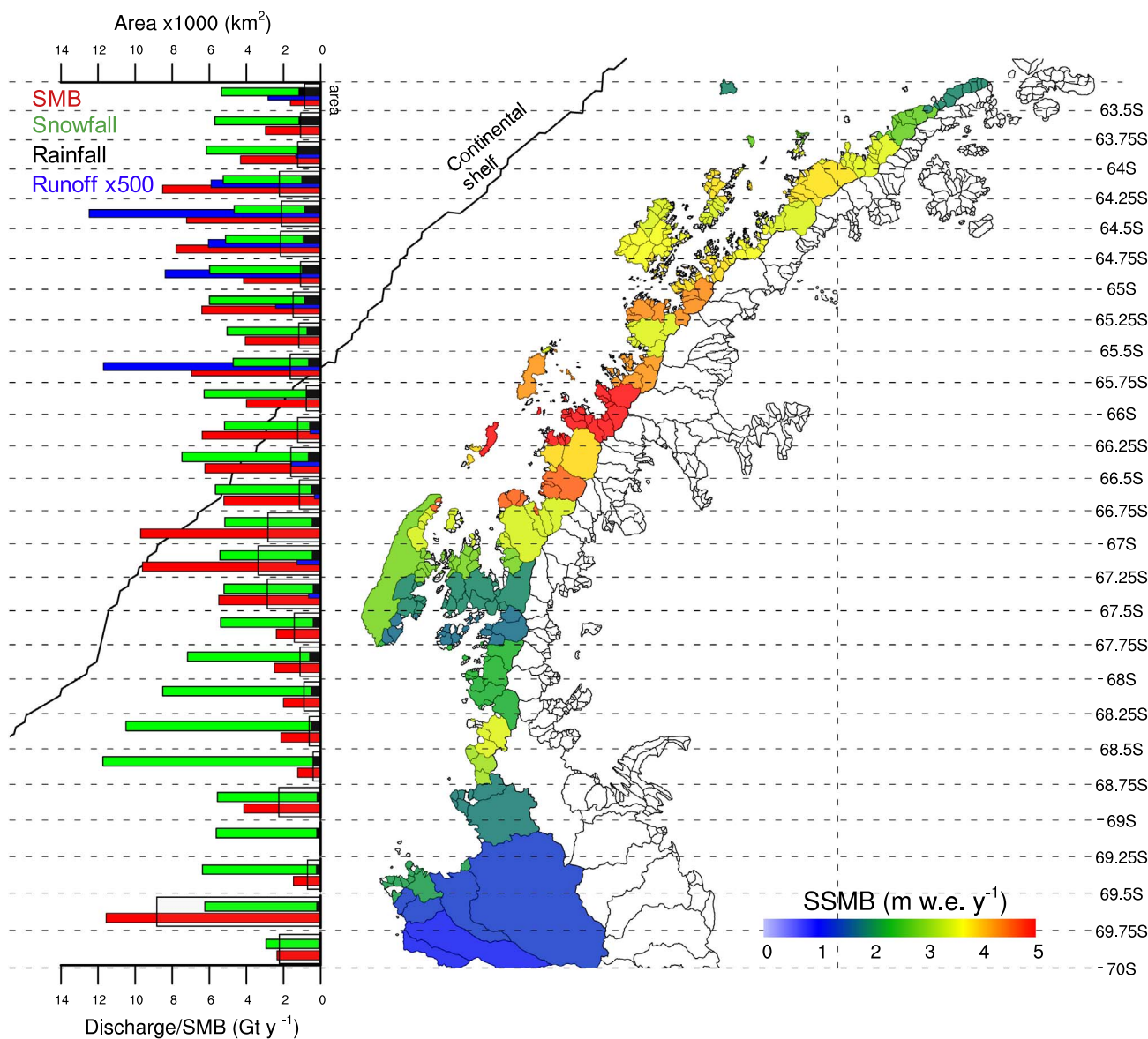
Fig. 6. Specific (area averaged) surface mass balance (SSMB; m w. e. y^{-1} ; colours), basin integrated SMB ( Gt y^{-1} ; red bars), meltwater runoff ( 500-Gt y^{-1} ; blue bars), ocean integrated snowfall/rainfall ( Gt y^{-1} ; green/black bars) and area ( 1000 km^2 ; black boxes) binned into 27 latitudinal intervals ( 0.25^\circ ). Only WAP basins larger than the area of one gridbox are used. Basin definitions are based on Cook et al. (2014). For each basin, the average latitude is calculated, which is used to determine to which bin the basin belongs. Ocean basins are based on all gridboxes up to the continental shelf (black line; see Fig. 1). (For interpretation of the references to color in this figure legend, the reader is referred to the web version of this article.)
