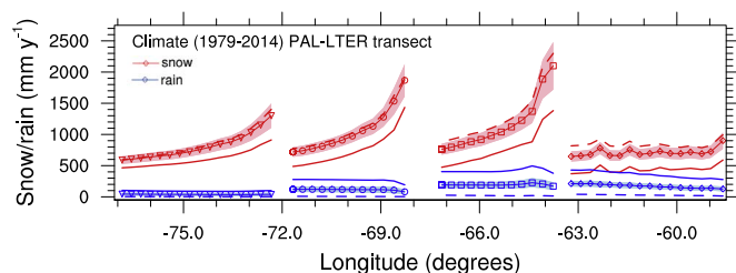
Fig. 3. Climatological (1979–2014) snowfall (red) and rainfall (blue) ( \text{mm w. e. y}^{-1} ) across Pal-LTER transects (see Figs. 1 and 2) 900 (diamonds), 600 (squares), 300 (circles) and 000 (triangles). Shading denotes interannual variability (one standard deviation). The dashed lines denote the winter (Jun., Jul., Aug.) averages, the solid (unmarked) lines the summer (Dec., Jan., Feb.) averages. Each of the transects is extrapolated so as to include two land points. (For interpretation of the references to color in this figure legend, the reader is referred to the web version of this article.)
