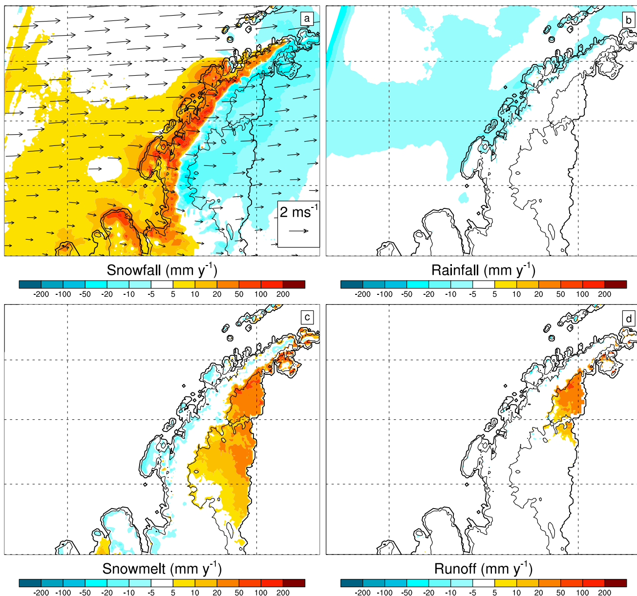
Fig. 4. Difference of the SAM + /ENSO - composite with the climatology (1979–2014) of the summer months (Dec., Jan., Feb.) freshwater components snowfall (a), rainfall (b), snowmelt (c) and meltwater runoff (d), in mm w. e. y -1 for 1979–2014. In (a) 500 hPa wind speed difference vectors are also shown. Details are found in Section 2.2.
