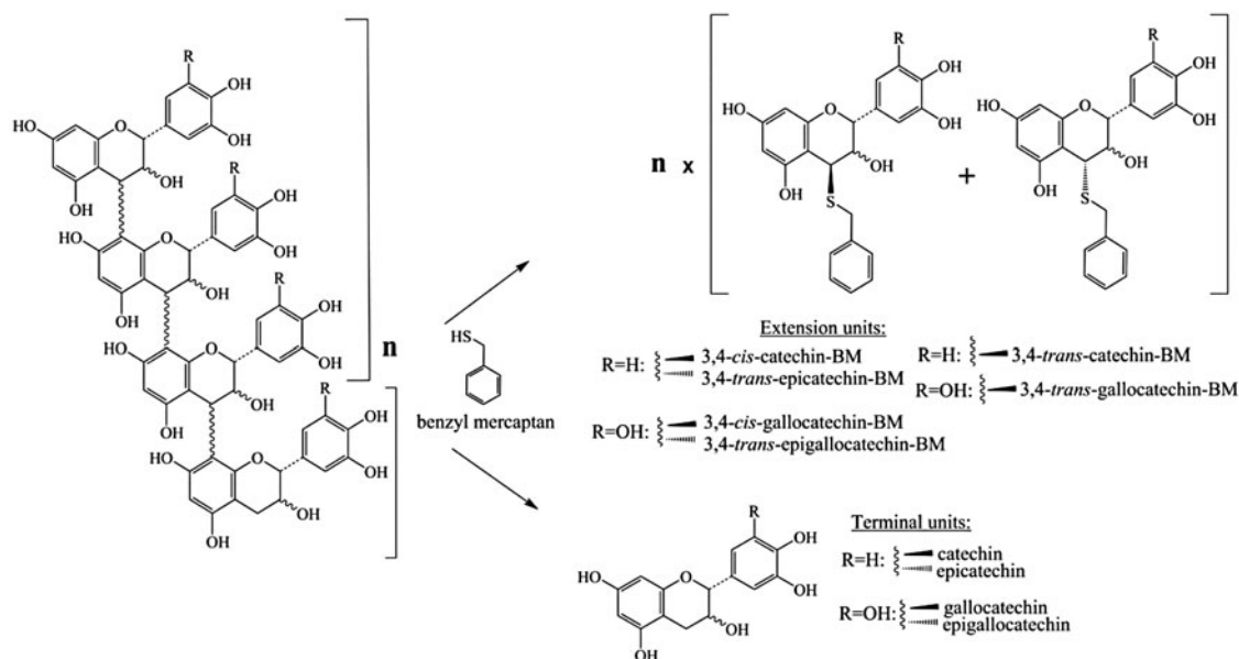
Fig. 1. Thiolytic degradation of condensed tannin polymers. Extension subunits are released as flavan-3-ol benzyl mercaptan (BM) adducts, terminal subunits are released as the free flavan-3-ols (Gea et al. 2011).
