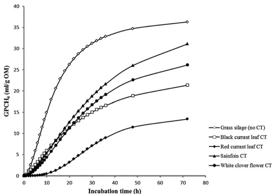
Fig. 3. Methane production profiles of grass silage with four condensed tannins extracts without polyethylene glycol (-PEG) (proportion of prodelphinidins, PD > 60 ).
