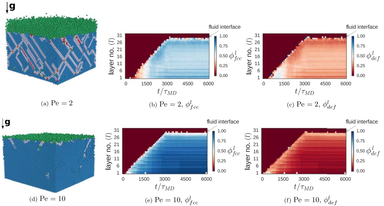
FIG. 2. ((a) and (d)) Side view of the final configurations at t/\tau_{MD} = 6000 of hard spheres sedimenting on an fcc (100) template with lattice spacing a = 1.004\sigma for Pe = 2 and 10 , respectively. The spheres in the snapshots are colored as follows: red: fcc (111), yellow: hcp, blue: fcc (100), lilac stacking fault, or another crystal structure, green: disordered. ((b) and (e)) Fraction of fcc particles \phi_{fcc}^l as denoted by the color bar, calculated over the total number of crystalline particles in each layer, showing the crystallization of each layer with time. ((c) and (f)) Fraction of particles belonging to a fault/defect \phi_{def}^l as denoted by the color bar, calculated over the total number of crystalline particles in each layer, plotted for each layer over time. The dark red region to the left of the four plots represents the absence of crystalline particles in the layer, i.e., a fluid layer. The initial packing fraction \eta_i = 0.02 .
