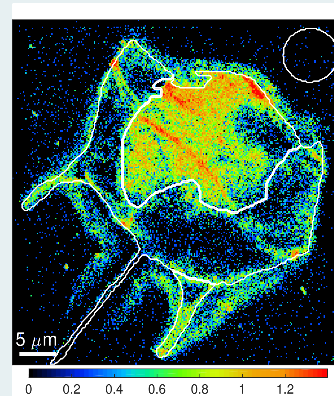
Figure 4 - \log(^{31}\text{P})
