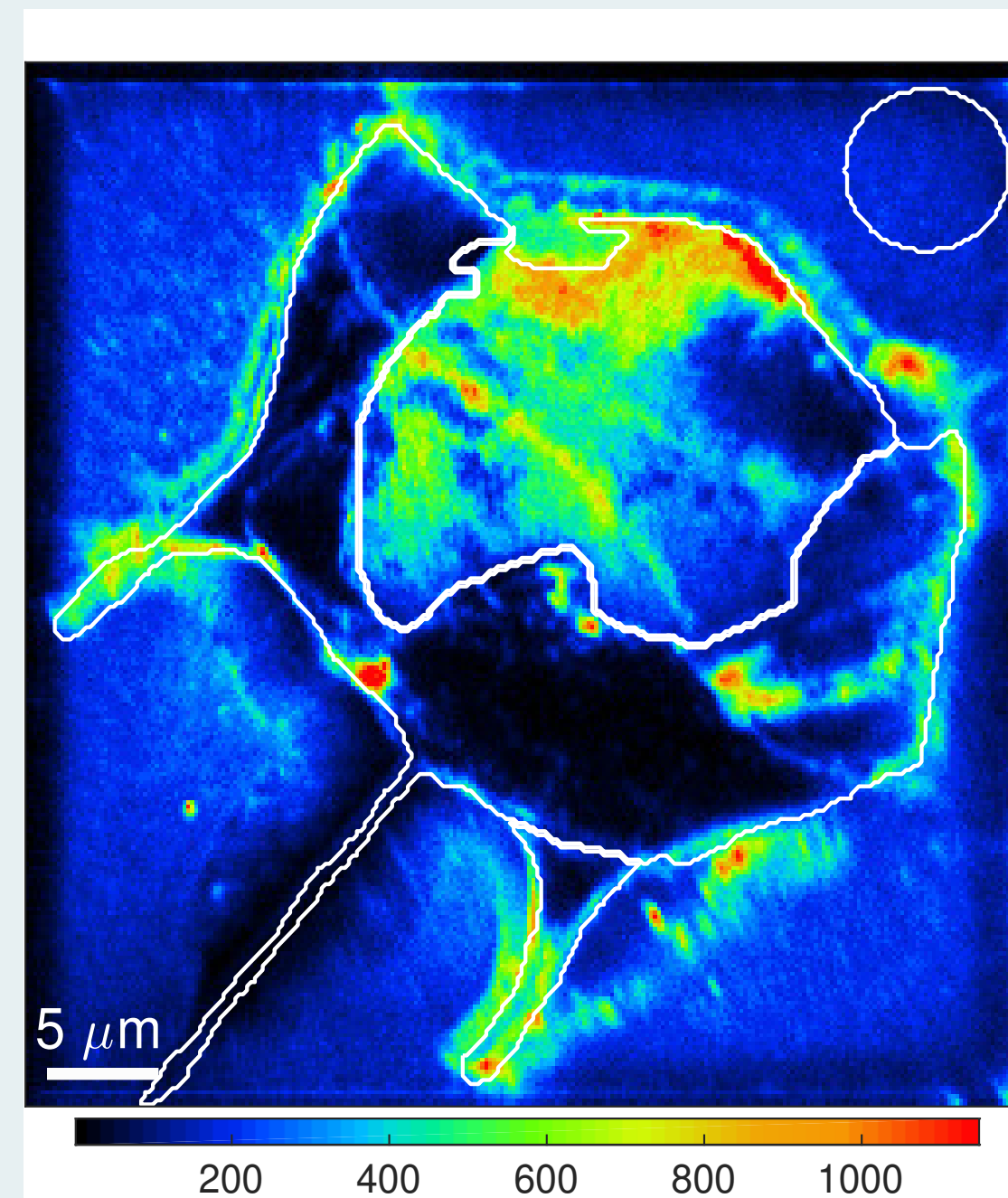
Figure 3 - ^{12}\text{C}^{14}\text{N}
