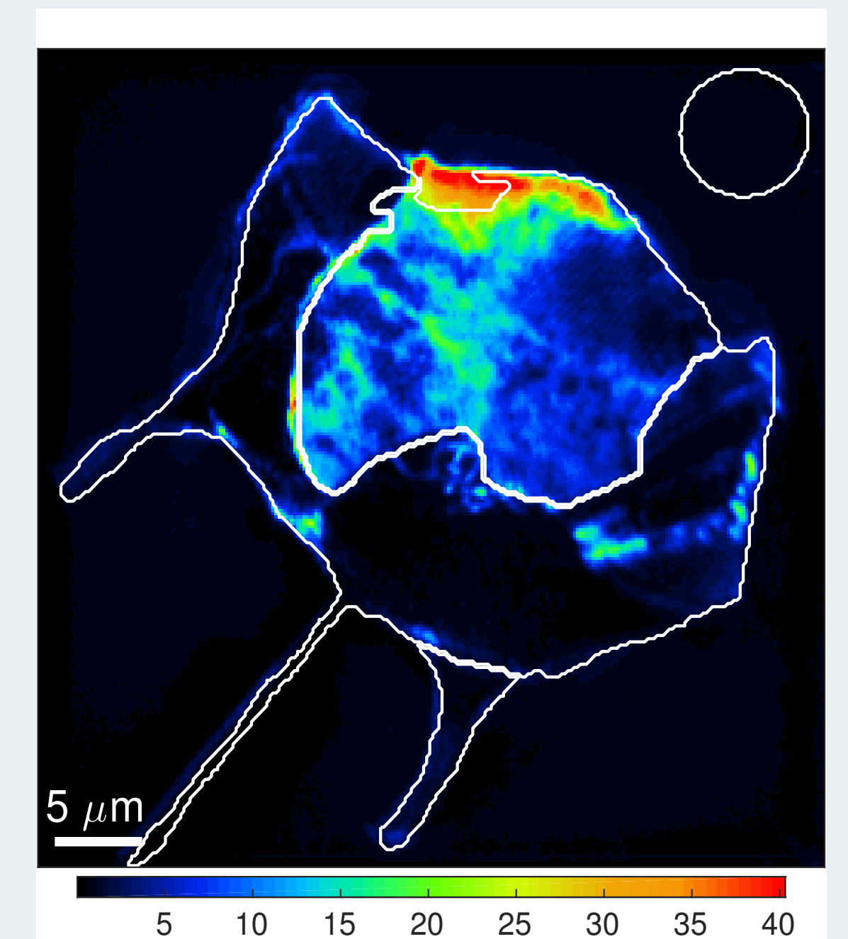
Figure 5 - ^{32}\text{S}
