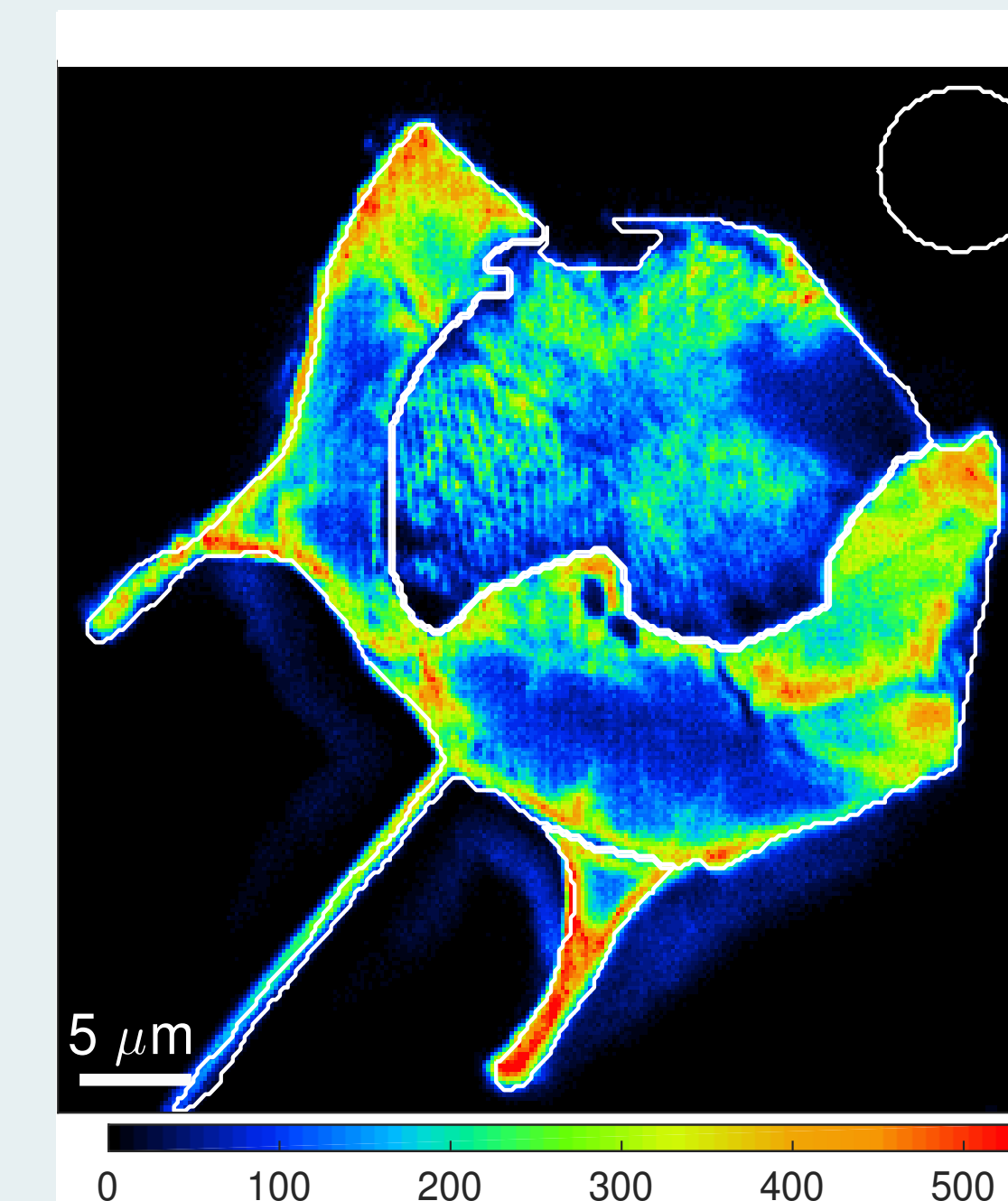
Figure 2 - ^{28}\text{Si}
