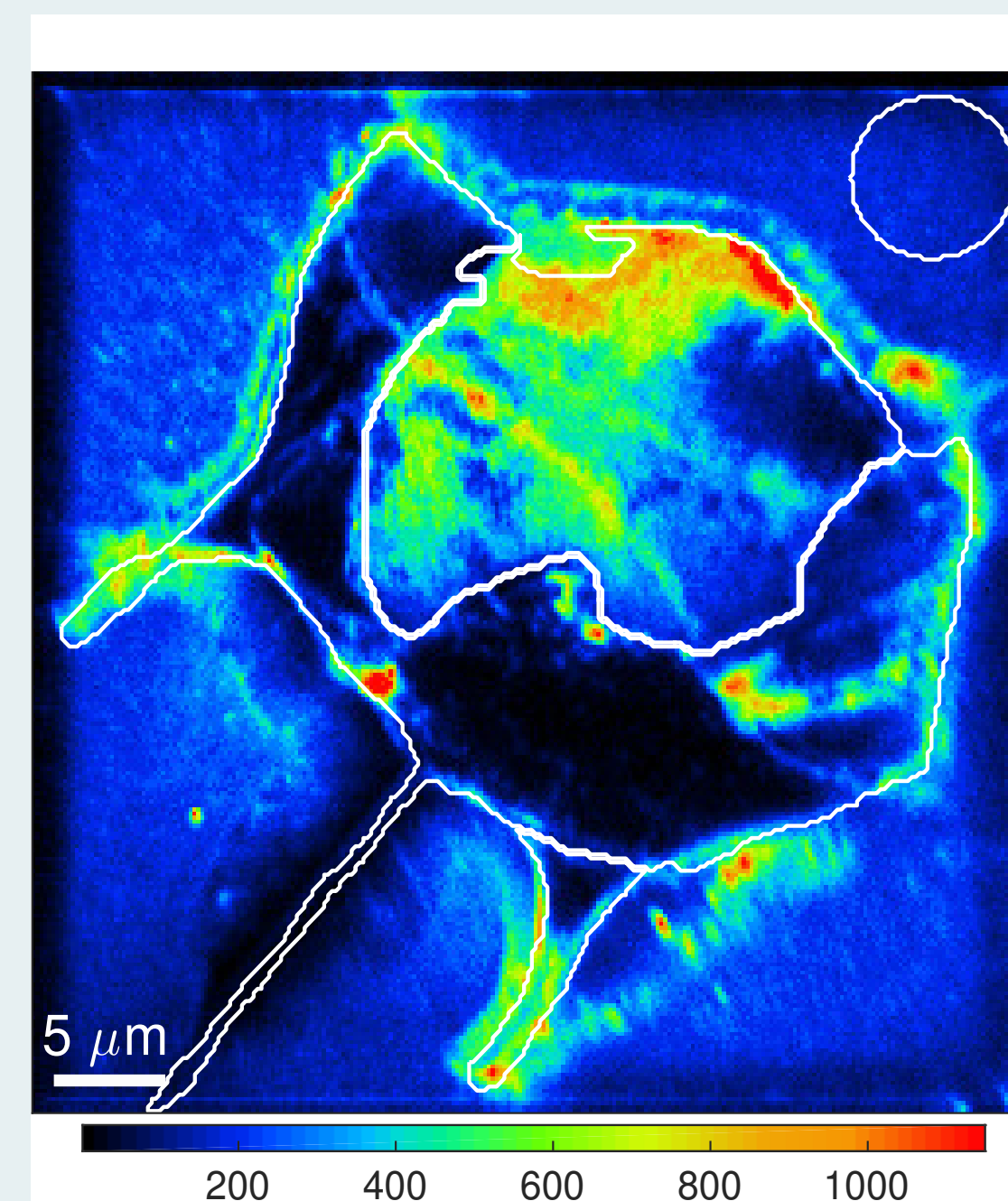
Figure 3 - ^{12}\text{C}^{14}\text{N}
