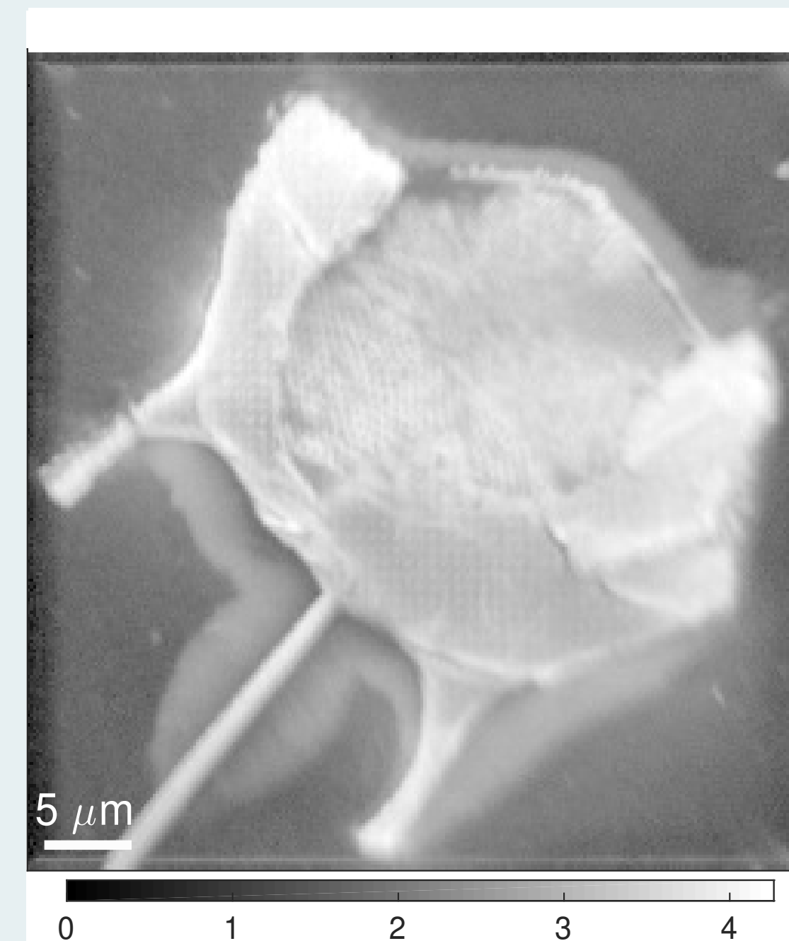
Figure 1 - \log(^{16}\text{O})
