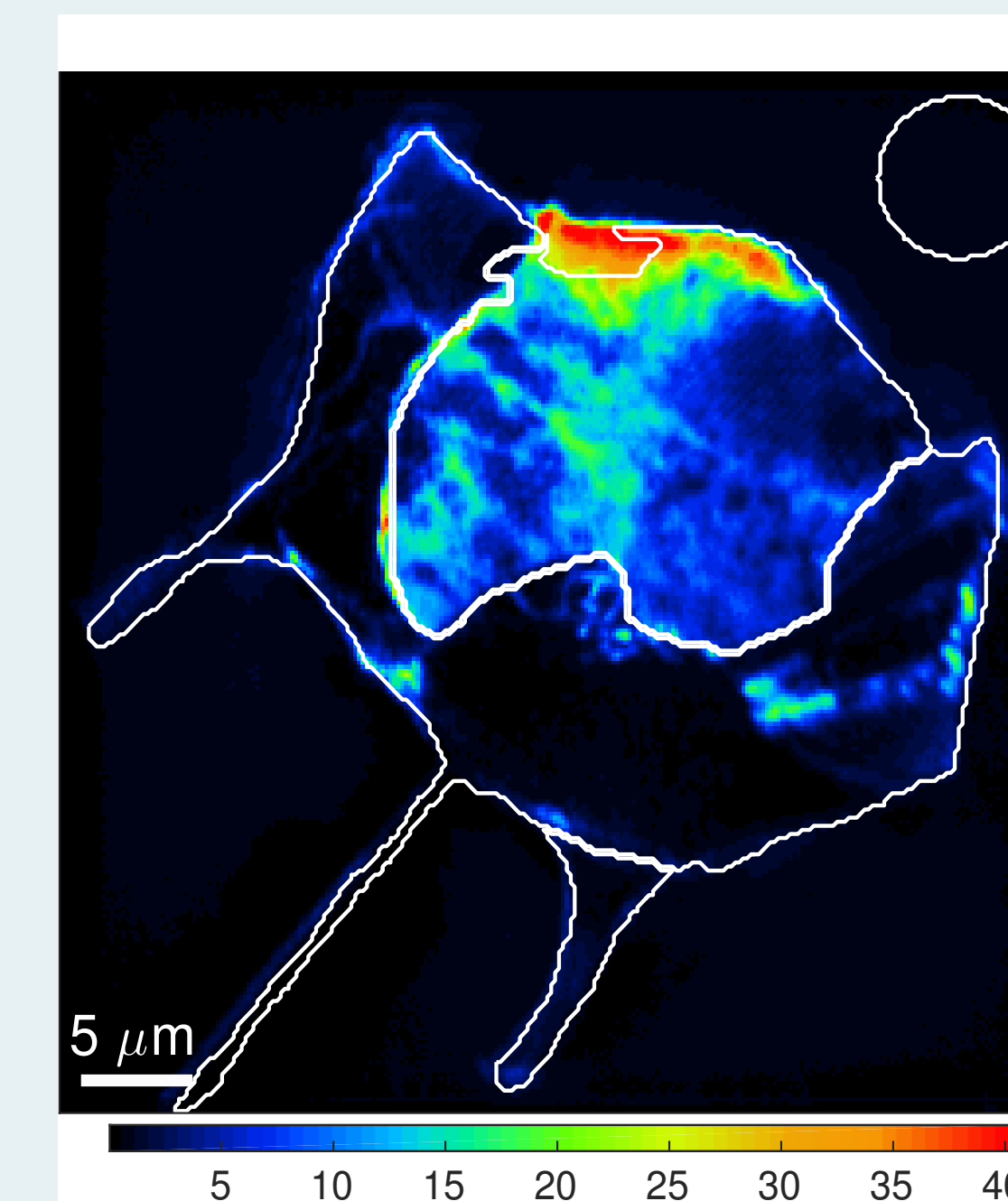
Figure 5 - ^{32}\text{S}
