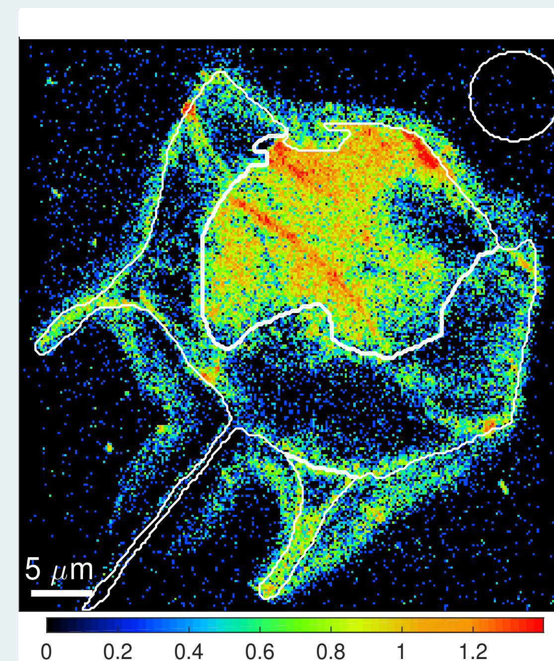
Figure 4 - \log(^{31}\text{P})
