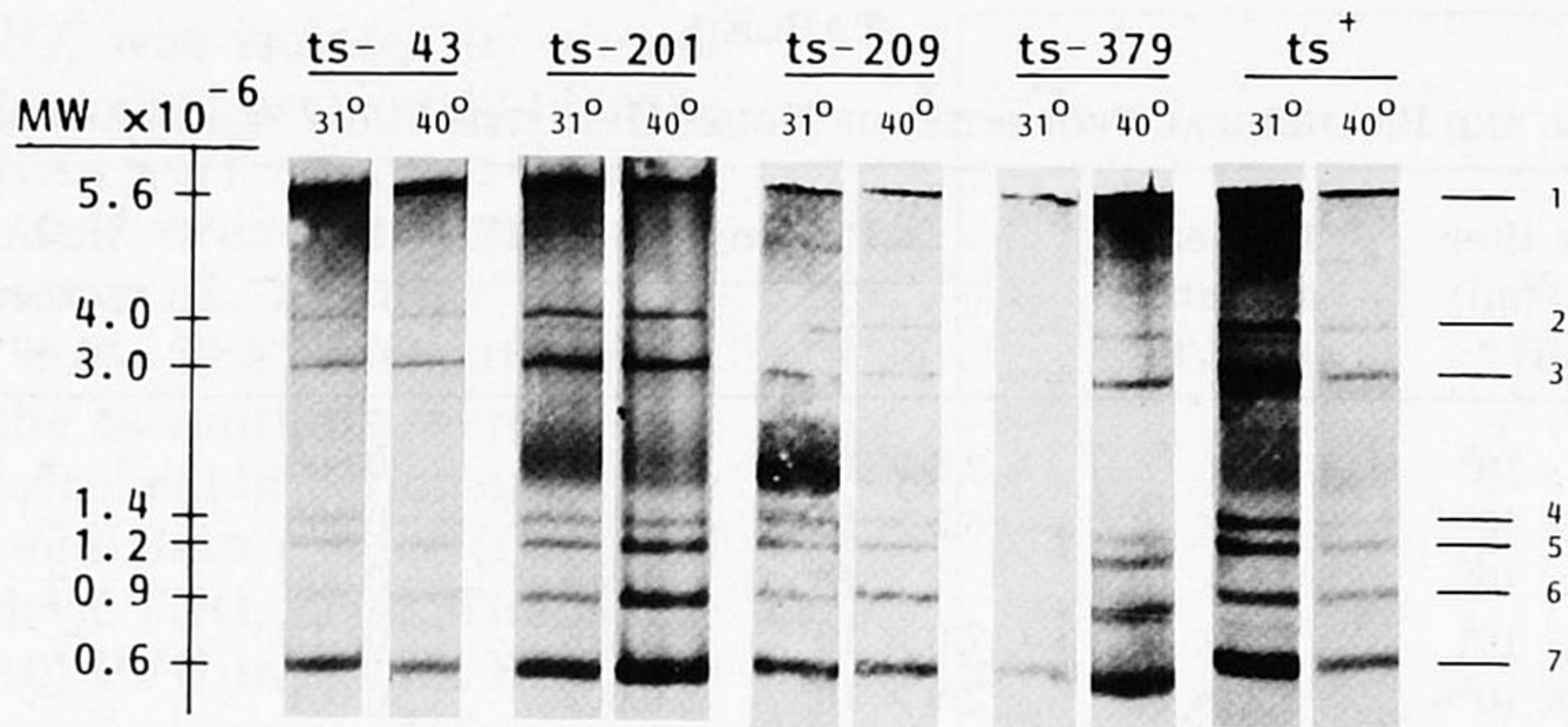
FIG. 2. Analysis by agarose gel electrophoresis of virus-specific RNAs extracted from Sac(-) cells infected with wild type MHV-A59 ( ts^+ ) or RNA + ts mutants grown at 31° and 40°. Gels were loaded with equal amounts (50,000 cpm) of radioactivity of the virus-specific RNAs synthesized at 31°, which were compared with RNA extracted from an equal number of cells incubated at 40°. Fluorographs were exposed for 7 days.
