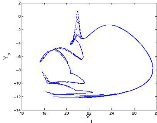
Fig. 5. A strange attractor at \gamma = 0.0892 , horizontal y , vertical \dot{y} ; from 4
