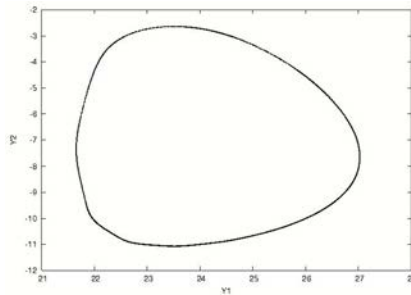
Fig. 3. Torus in projection of Poincaré-section (y, \dot{y}) at \gamma = 0.092 , b = -0.5 , \delta = 0.4 , \kappa = 0.1 , horizontal y \in [21, 28] , vertical \dot{y} \in [-12, -2] ; from 4
