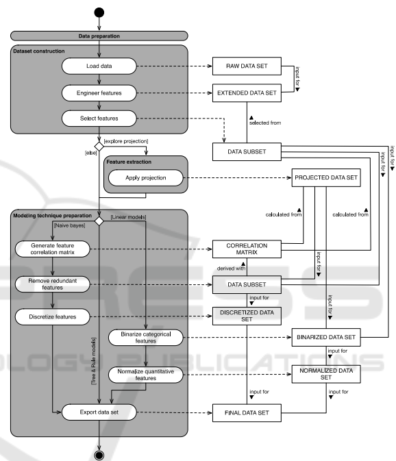
Figure 3: Data preparation method fragment.
