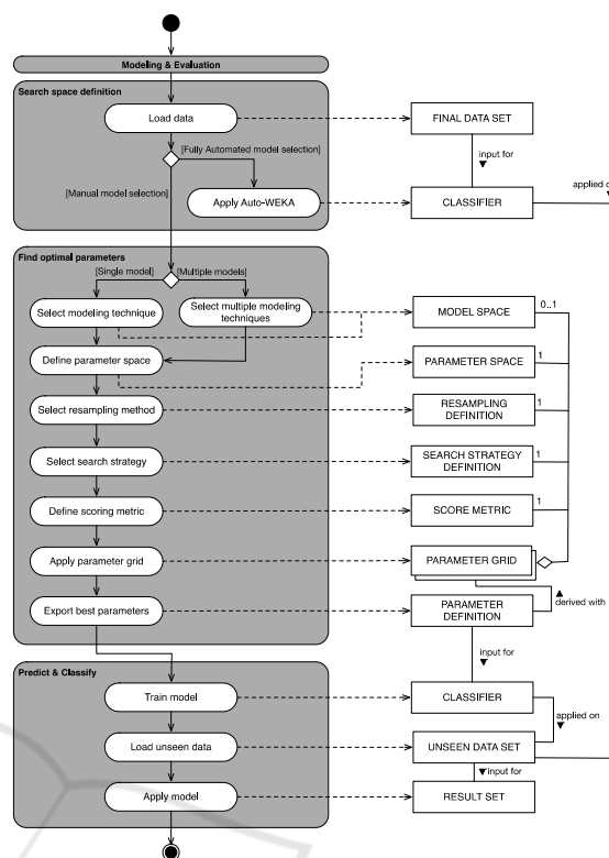
Figure 4: Modelling & evaluation method fragment.
