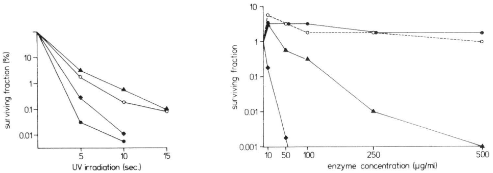
Fig. 2. Rates of virus inactivation by UV irradiation. UV inactivation of Berne virus (full circles; starting titre 10^{5.7} ), as compared with that of a togavirus (Semliki forest virus, triangles; 10^{7.0} ), a rhabdovirus (rabies virus, squares; 10^{7.1} ) and equine herpes virus 1 (empty circles; 10^{7.2} ) as a DNA virus representative.
