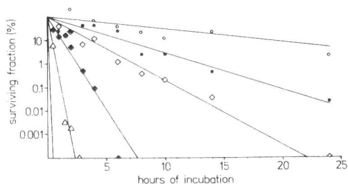
Fig. 1. Thermal inactivation of Berne virus. Loss of infectivity is linear at 31°C (open circles, correlation coefficient r = 0.949 ), 35°C (closed circles, r = 0.967 ), 39°C (open squares, r = 0.969 ), 43°C (closed squares, r = 0.982 ), 47°C (triangles, r = 0.983 ), 51°C and 55°C (no symbols). The untreated material had an infectivity titre of 10^{6.5} ID 50 units ml -1 ( \approx 100\% ).
