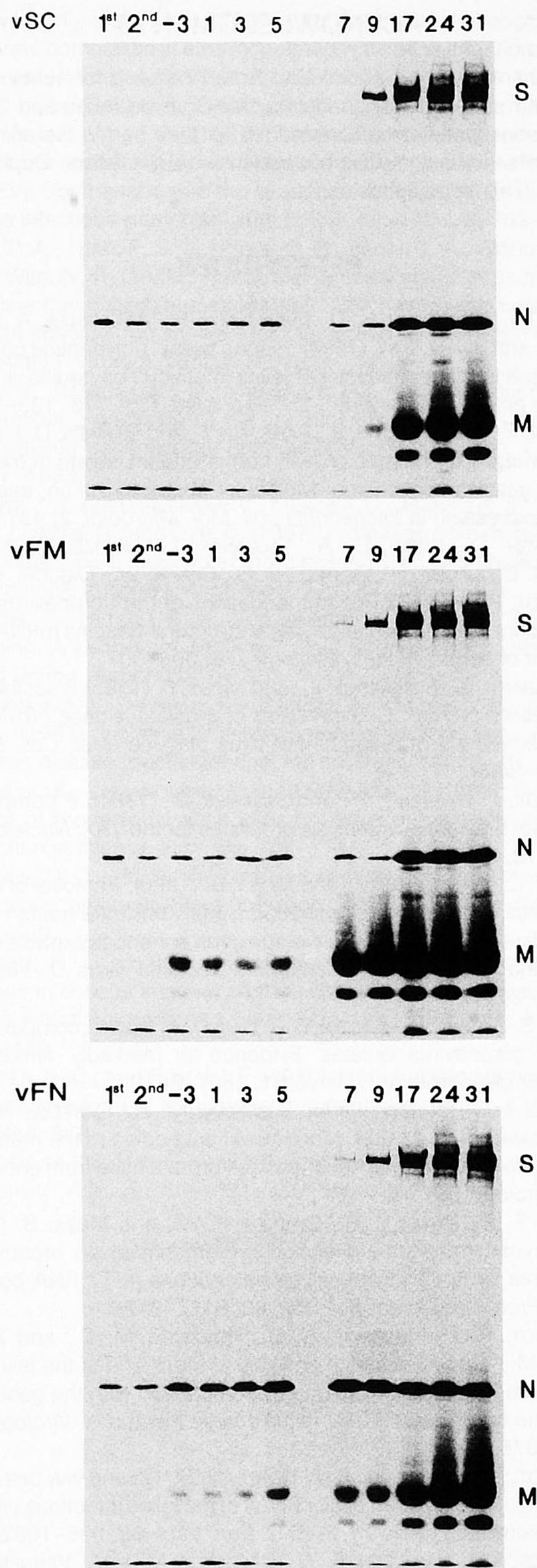
FIG. 6. SDS-PAGE analysis of RIP assays with pooled sera from experimentally infected kittens. FIPV-specific antibodies were detected using a lysate of metabolically labeled FIPV-infected fcwf-D cells as antigen source. Panels vSC, vFM, and vFN: pooled sera of eight kittens immunized with vSC, vFM, or vFN, respectively. The lanes marked 1st, 2nd, and -3 represent reactions at the day of the first and second immunization, and at 3 days before challenge. Subsequent numbers indicate the postchallenge day on which sera
