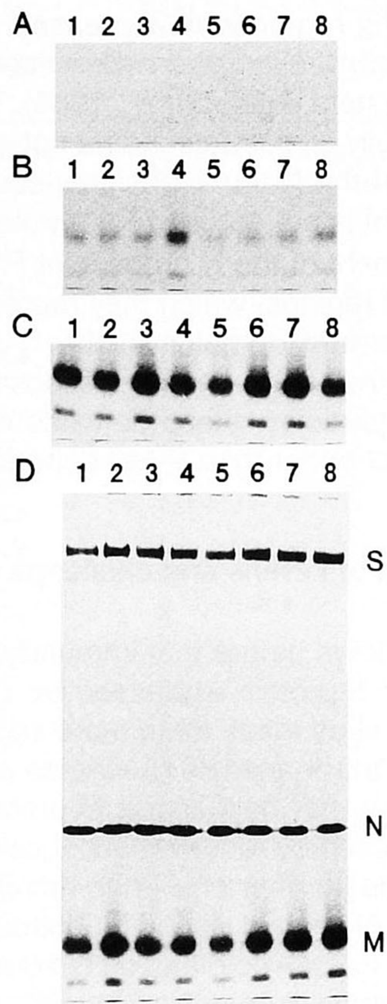
FIG. 7. SDS-PAGE analysis of RIP assays with individual sera of the vFM-immunized group. Kittens immunized with vFM were numbered from shortest to longest survival time after challenge; these were 21 days for 1 (89S), 23 days for 2 (89R) and 3 (M93), 36 days for 4 (M94), 41 days for 5 (M88), or more than 90 days for 6 (M87), 7 (721), and 8 (M79). Sera were from the day of the second immunization (A), from 3 days before challenge (B), and from 9 (C) and 17 (D) days after challenge; panels A through C represent only the lower portions of the gels containing the M protein bands. D illustrates the primary immune response against the S and N proteins. The structural proteins have been indicated.
