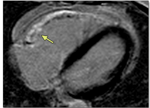
FIGURE 6 Phase-Sensitive Inversion Recovery Image After Administration of a Gadolinium Chelate by CMR in a 47-Year-Old Woman With ARVD/C
