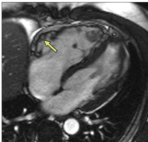
FIGURE 4 Four-Chamber Bright Blood Image by CMR of a 50-Year-Old Man With ARVD/C
