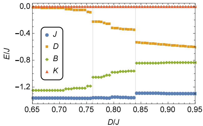
FIG. 3. The energy contributions E/J to the ground state of the interactions with coupling parameters J , D , B , and K are shown as a function of D/J at parameter values J = -1 , B = 3.2 , and K = 0 for a system of size L = 32 . The system undergoes two phase transitions at D/J = 0.76 and D/J = 0.84 between the spin-flop, 2q , and spiral phase, respectively. These are depicted as vertical gray lines. The discrete jumps in various energy contributions suggest first-order phase transitions.
