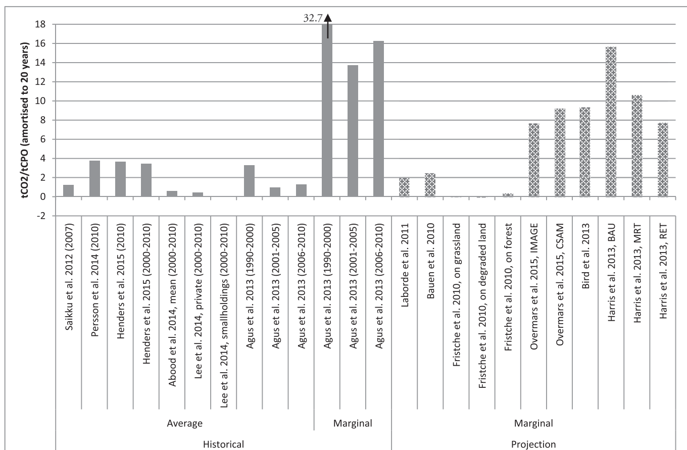
Fig. 2. Harmonised CSC-LUC values for Indonesian palm oil from selected studies.
