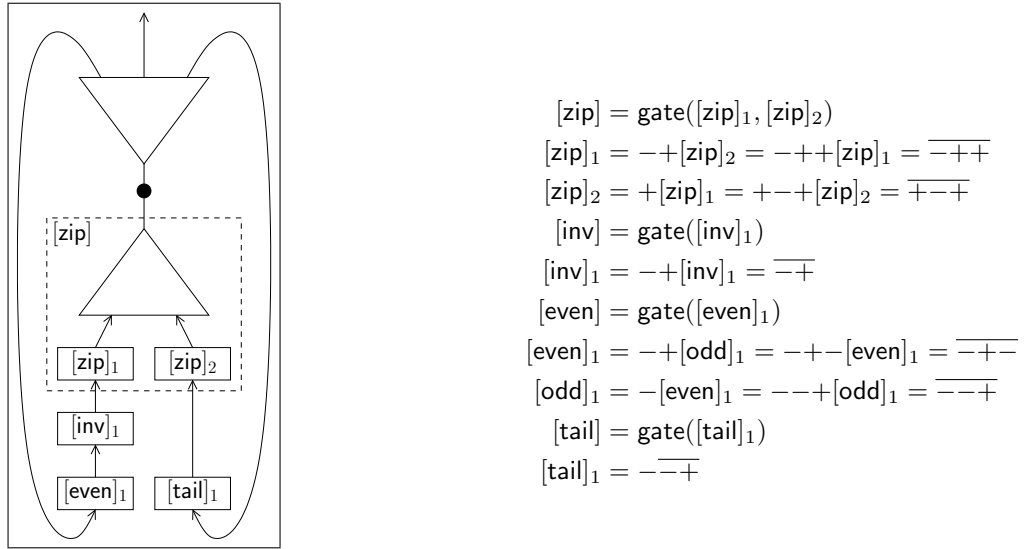
Figure 9: The net translation [M] = \mu M. \bullet([\text{zip}]([\text{inv}]([\text{even}](M)), [\text{tail}](M))) of M .
