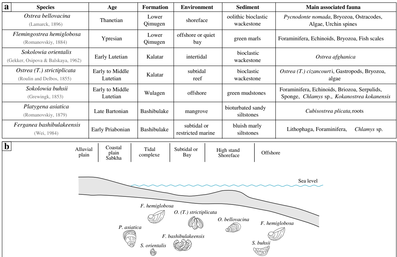
Fig. 2. a. Environment of the studied species: age, formation, depositional environment and associated fauna. b. Living position of species through the carbonate platform.
