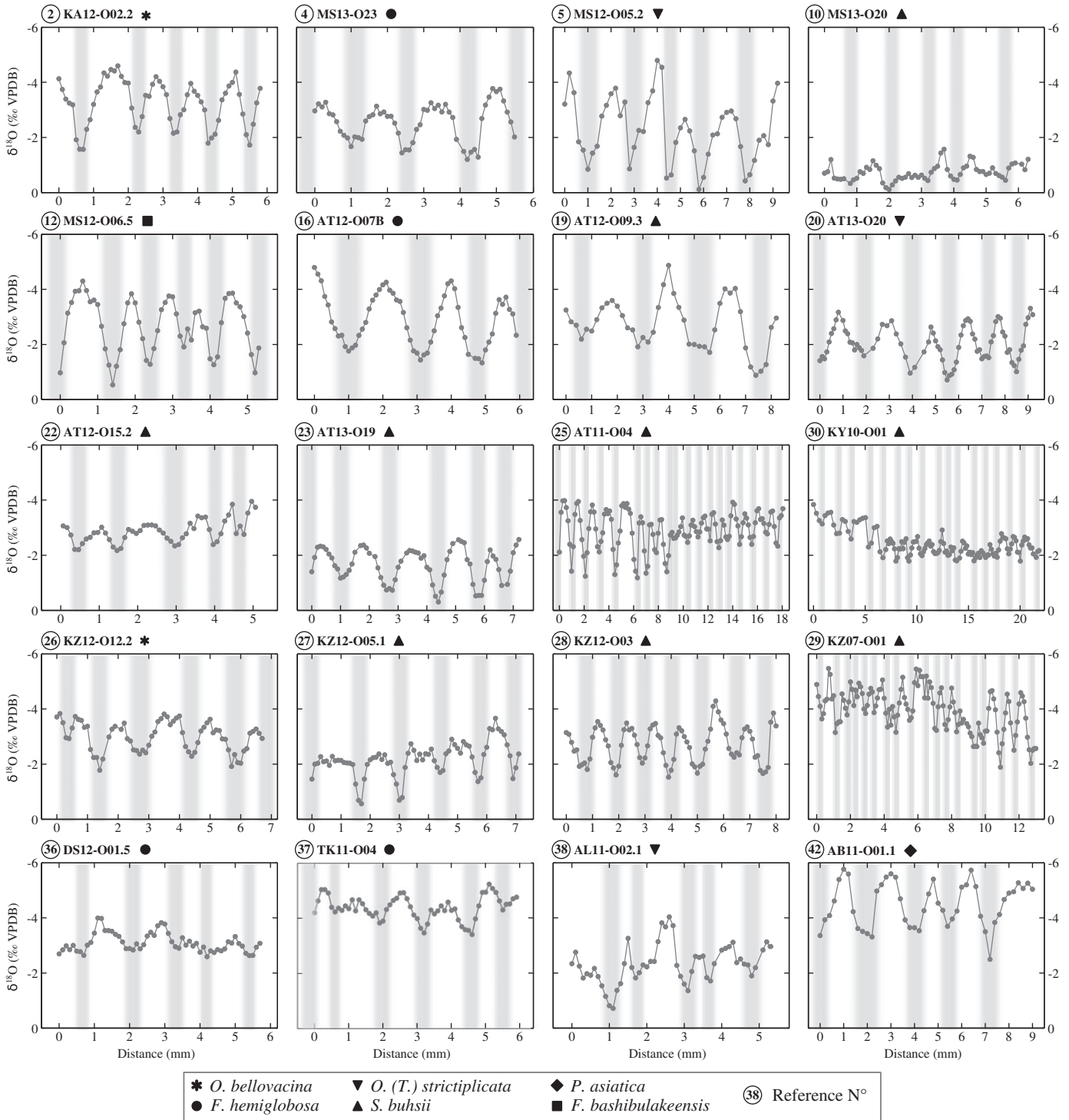
Fig. 5. Incremental stable oxygen ratio records ( \delta^{18}\text{O} ) in oyster shells. Horizontal axis indicates distance in millimetres starting from the first drilled micro-sample. Grey areas correspond to visible dark bands on the shells, white areas correspond to the light bands revealed by CL analyses.
