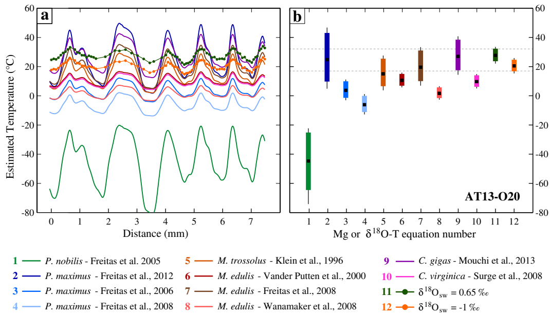
Fig. 10. a. Intra-annual temperatures (0.2 mm moving average) for the specimen AT13-O20 estimated using various Mg/Ca calibrations established on different species of calcitic bivalves (1 to 10, cf Table 1), or using \delta^{18}\text{O} calibration of Anderson and Arthur (1983) with a constant \delta^{18}\text{O}_{\text{sw}} of 0.65‰ according to modelled values for the study area in the Eocene (Tindall et al., 2010) (11), or of -1\text{‰} according to the value commonly used for the Eocene ice free world (12). b. Associated temperature range for each calibration.
