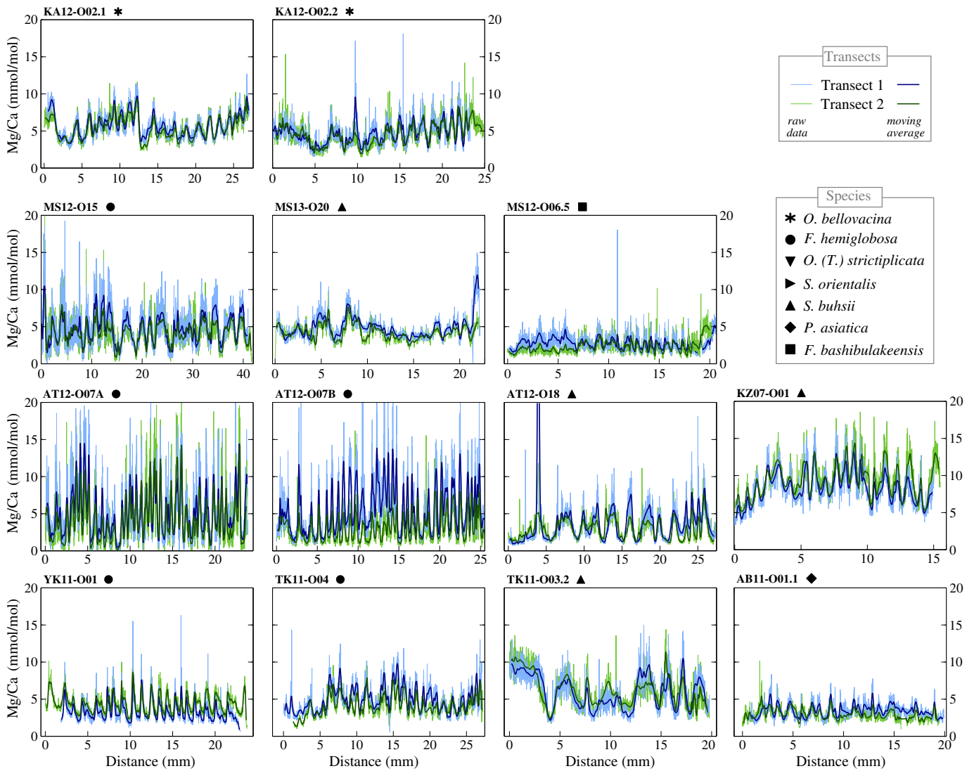
Fig. 7. Partly suitable Mg/Ca results across the oyster shell ligamental area showing only parts with well-expressed cyclicality and low intra-shell variability between parallel transects (Fig. 3). Analyses were performed following the growth direction with 0 mm corresponding to the most juvenile part analysed.
