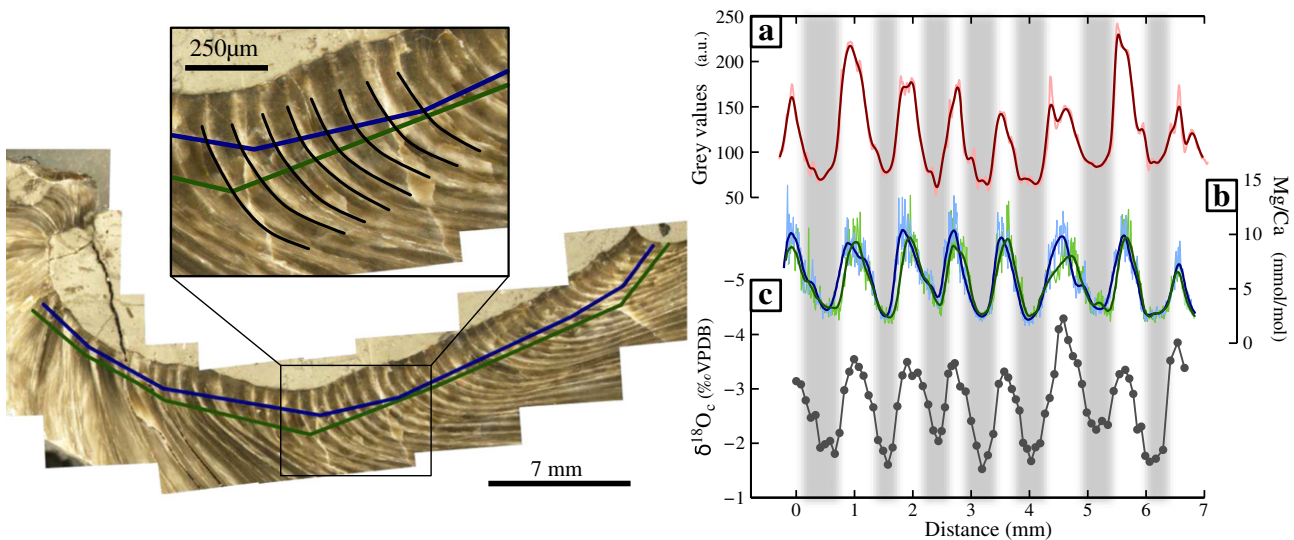
Fig. 4. Geochemical data for the specimen KZ12-O03 ( S. buhsii ): cathodoluminescence grey scale (light red: raw data, dark red: moving average) results, Mg/Ca ratio for two parallel transects yielding similar results (light blue or green: raw data, dark blue or green: moving average), Oxygen stable isotopes from the selected area. Grey areas correspond to light and dark layers as revealed by CL.
