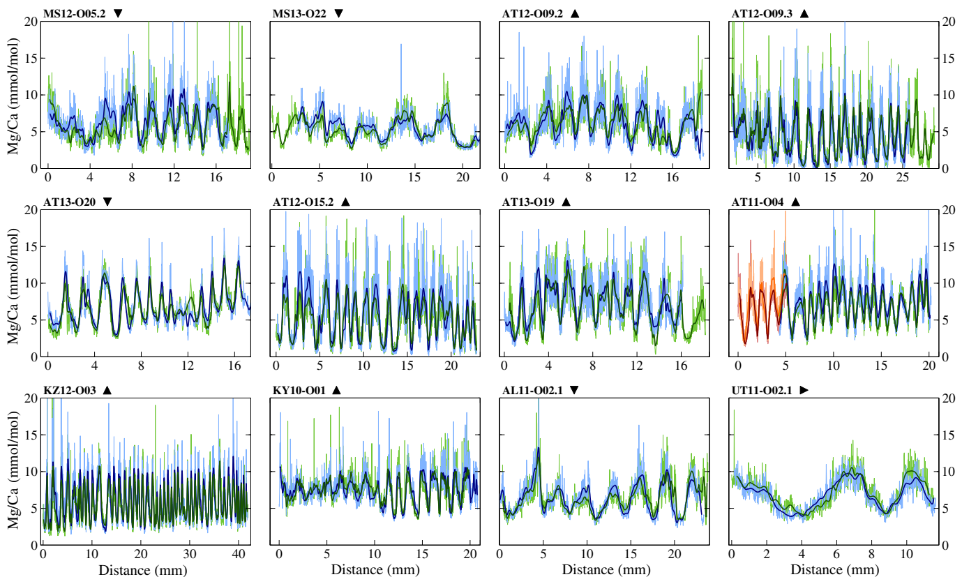
Fig. 6. Suitable Mg/Ca result across the oyster shell ligamental area showing both well-expressed cyclicity and low intra-shell variability between parallel transects (Fig. 3). Analyses were performed following the growth direction with 0 mm corresponding to the most juvenile part analysed. See Fig. 8 for explanatory legend of used symbols and patterns.
