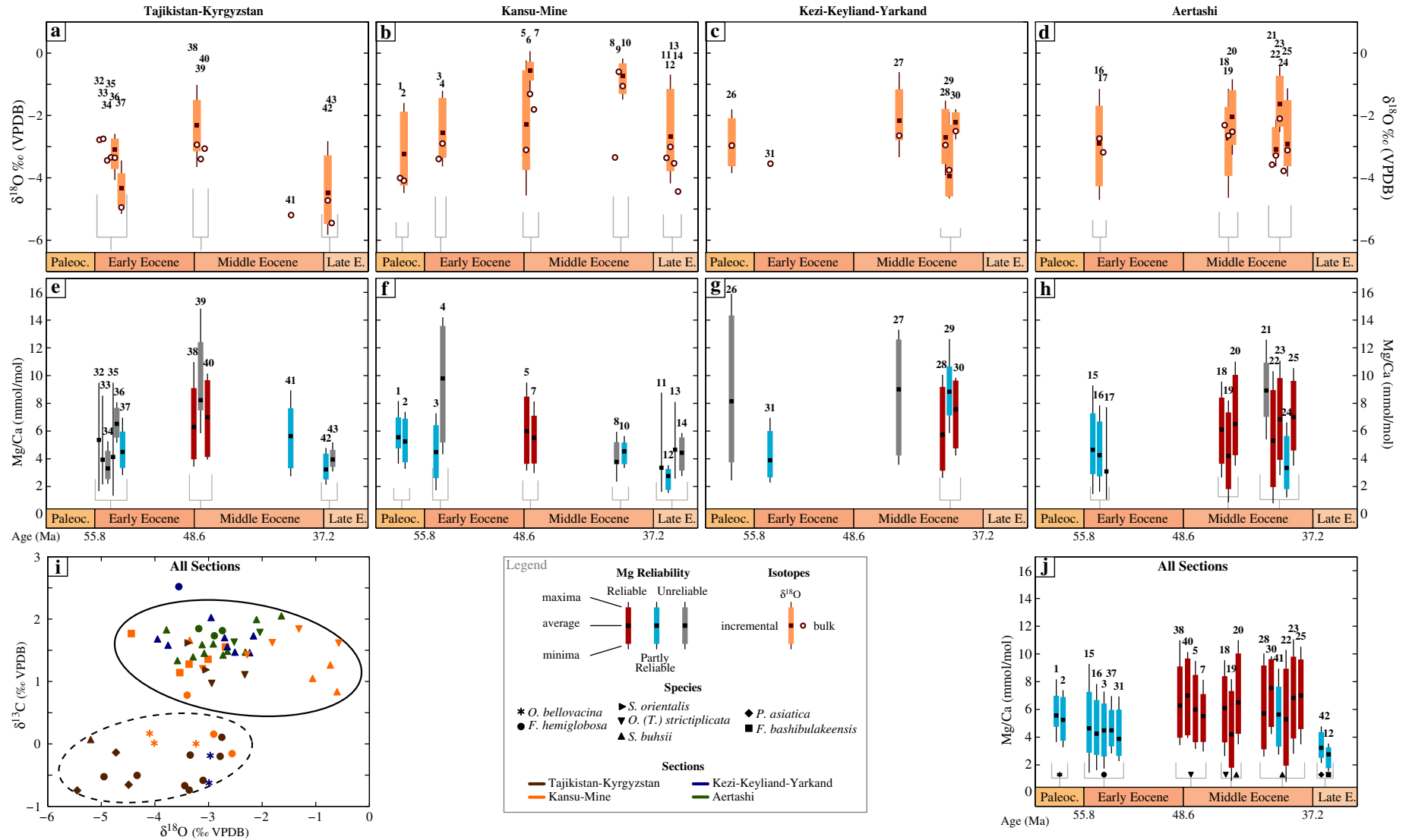
Fig. 9. a.–d. \delta^{18}\text{O} results from bulk and incremental analyses per stratigraphic section. e.–h. Mg/Ca results from incremental analyses per stratigraphic section. When the seasonal pattern could not be defined, we represented only the average (full black square) and a black line between the highest and lowest values. Red depicts suitable signal, blue partly suitable signal and grey unsuitable signal. When oysters are coming from the same bed, the estimated age is the same. However, to enhance visibility of the difference between them, we juxtaposed results next to each other. Numbers correspond to the Ref. N° in Table 2. i. \delta^{13}\text{C} vs \delta^{18}\text{O} for bulk and averaged incremental results. Two groups can be clearly distinguished between relatively high (full line) and low (dashed line) values of \delta^{18}\text{O} and \delta^{13}\text{C} . j. Compiled Mg/Ca results from the complete collection with suitable and partly suitable criteria.
