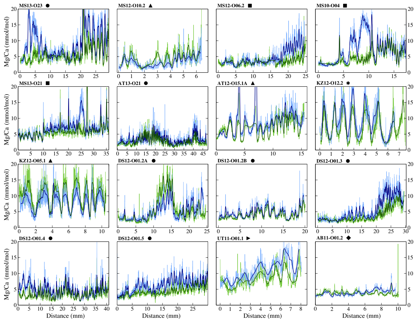
Fig. 8. Unsuitable Mg/Ca results across the oyster shell ligamental area showing poorly-expressed cyclicity and high intra-shell variability between parallel transects (Fig. 3) of oyster shells. Analyses were performed following the growth direction with 0 mm corresponding to the most juvenile part analysed.
