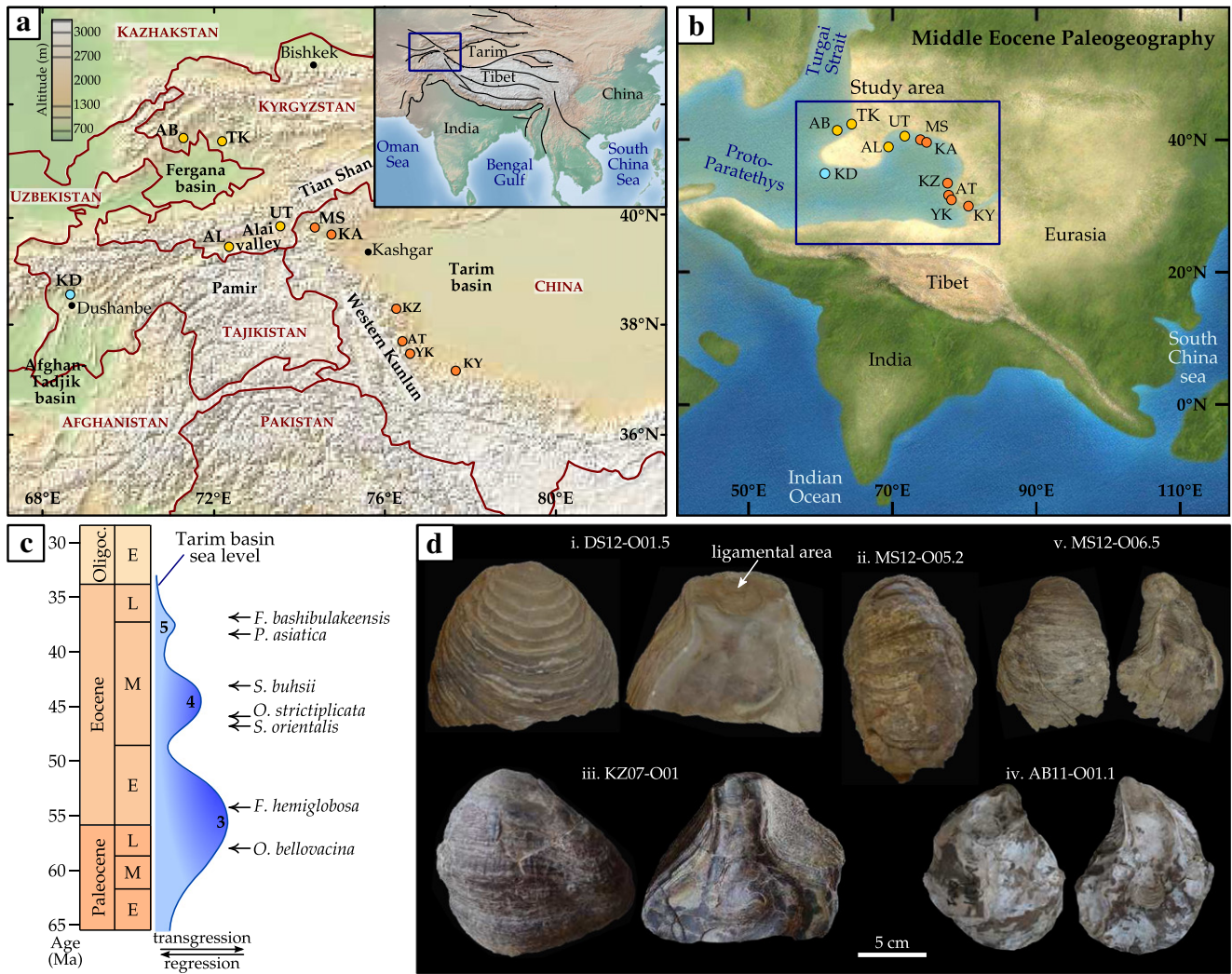
Fig. 1. a. Location of sampling area in Kyrgyzstan (yellow), Tajikistan (blue) and China (orange). b. Middle Eocene Palaeogeographical map showing Central Asia invaded by the Proto-Paratethys sea (map from Licht et al., 2014). c. Position of analysed species on schematic illustration of the third to fifth marine incursions into the Tarim Basin (Bosboom et al., 2014b). d. Examples of analysed fossil oyster left valves with well-developed ligamental area. (i.) F. hemiglobosa , (ii.) O. (T.) strictiplicata , (iii.) S. buhsii , (iv.) P. asiatica , (v.) F. bashibulakeensis . The first part of the specimen's name indicates the provenance with the code of the stratigraphic sections (see section codes below), and the year of sampling. The complete list of oysters from Central Asia analysed in this study is available in Supplementary data. Code for stratigraphic sections – MS: Mine-Bashibulake (39°51'N, 74°32'E), KA: Kansu (39°45'N, 74°58'E), KZ: Kezi (38°26'N, 76°24'E), AT: Aertashi (37°58'N, 76°33'E), YK: Yarkand (37.7°N, 76.6°E), KY: Keyliand (37°27'N, 77°86'E), AB: Ala Buka (41.4°N, 71.4°E), TK: Tash Kumyr (41.3°N, 72.2°E), AL: Alai Valley (39.6°N, 72.4°E), UT: Uch Tobo (39.9°N, 73.4°E), DS: Kuhdara-Dushanbe (38.7°N, 68.9°E).
