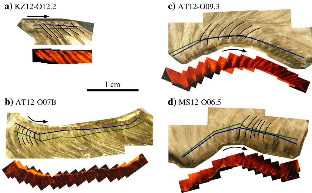
Fig. 3. Radial sections (top) of oyster ligamental areas showing light and dark alternations, each couplet corresponding to one growth year. Cathodoluminescence assemblages (bottom) for these specimens show alternation of areas with high and low luminescence corresponding to light and dark bands observed in natural light. Transects followed by laser ablation for trace element analyses are indicated in blue and green. Main paths followed by the Micromill for stable isotopes analyses are indicated in black. Black arrows indicate growth directions. (a.) O. bellovacina , (b.) F. hemiglobosa , (c.) S. buhsii and (d.) F. bashibulakeensis . Supplementary data provides the radial sections and CL images of complete collection.
