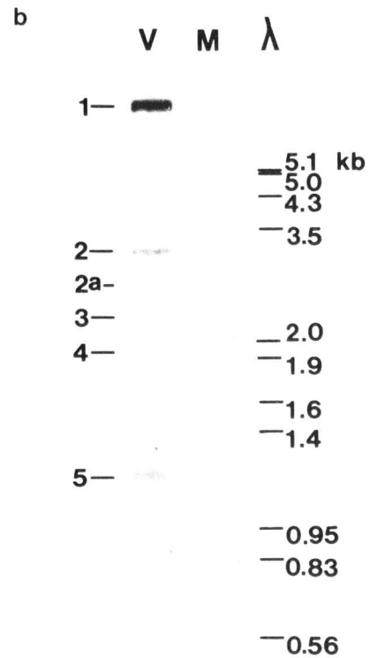
Figure 4. Determination of the 5'-end of RNA 6. (a) Primer extension on RNA from mock (M) and virus (V) infected BHK-21 cells. The elongation products were analyzed on a 8 M urea, 6% polyacrylamide gel. The primers used are pointed out below the gel. Samples from sequence reactions were included to yield the size ladder shown on the left. The extension products of RNA 5 and 6 are indicated separately. The extension products of RNA 5 were not within the separating range of the sequence gel. (b) Hybridization of oligonucleotide 32 to total cytoplasmic RNA from mock (M) and EAV (V) infected cells. The RNAs were resolved on a 1.5% agarose formaldehyde gel. A EcoRI/HindIII digest of bacteriophage lambda DNA, filled in with Klenow polymerase in the presence of [ \alpha - ^{32} P]dATP, was used as a size marker. The numbers at the right indicate the sizes and positions of the resulting fragments.
