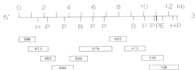
Figure 8. Physical map of the EAV genome. B, BamHI; E, EcoRI; H, HindIII; P, PstI. cDNA clones covering a continuous stretch of approximately 13 kb are aligned relative to the restriction map.
