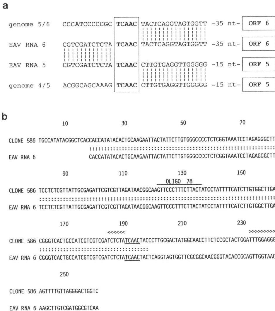
Figure 7. (a) Compilation of the sequences surrounding the divergence sites. The sequences entitled genome 4/5 and 5/6 represent the genomic sequences enclosing the junction sites of RNA 5 and 6 respectively. The position of ORF 5 and 6 relative to the junction sites of RNA 5 and 6 is indicated. A stretch of 5 nucleotides (5' TCAAC 3') is conserved at the junction sites of RNA 5 and 6. (b) Sequence of the 5'-terminus of the viral genome. The sequence of cDNA clones 586 is aligned with that of mRNA 6 specific cDNA clone 033. The part of the leader sequence that binds oligo 78 is indicated. The 5' TCAAC 3' motifs and the initiating codon of ORF 6 are underlined. <<<<<<< symbolizes a region with sequence homology to the 5'-splice site of the self-splicing pre-rRNA of Tetrahymena thermophila . >>>>>>> marks a possible internal guiding sequence.
