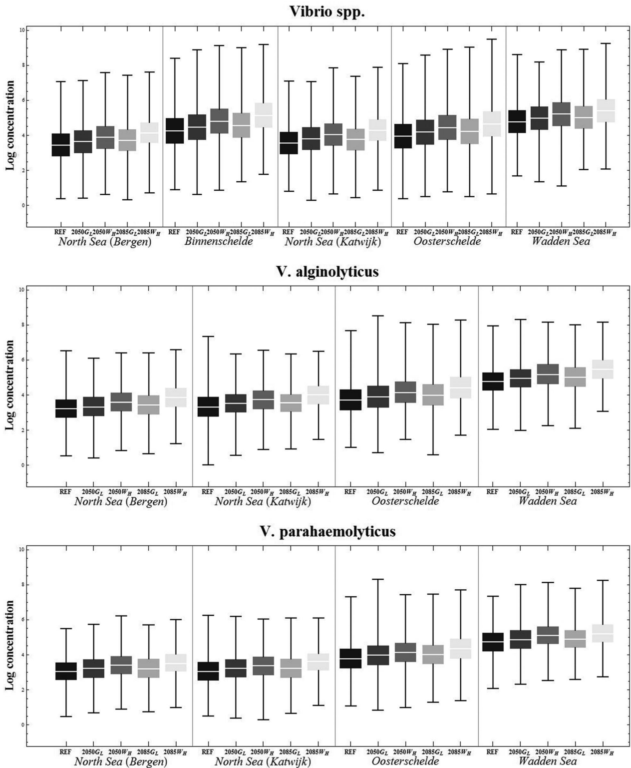
Fig. 3. Box whisker plots for predictions of future Vibrio LOG10 concentrations during summer under the different scenario's. The bottom of the box represents the 25th percentile and the top the 75th, the divider in the box shows the median and the whiskers extend to the highest and lowest observation. Variation includes both variation per season and uncertainty in the predictions.
