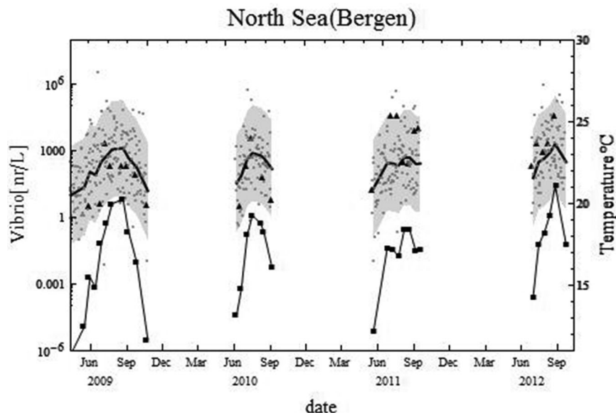
Fig. 2. Measured, predicted, and sampled concentrations for Vibrio spp. at the North Sea (Bergen), for enrichment at 36 °C for 6–8 (2009–2010) or 18–20 h (2011–2012). Black line shows mean prediction for Vibrio concentration; gray-shaded area encompasses the prediction interval for individual observations. Triangles represent the measured concentrations and dots represent random samples, as used for the calculations of illness risks. Squares represent temperature measurements.
