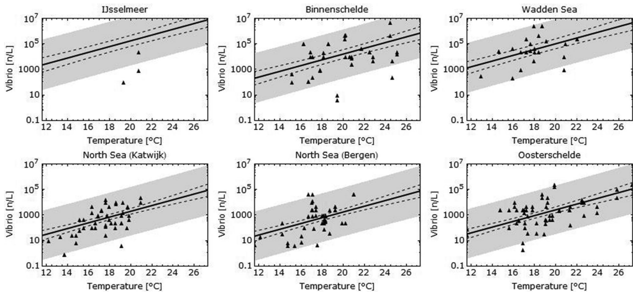
Fig. 1. Results of regression analysis for Vibrio spp., enrichment at 36 °C for 18–20 h. Triangles show measured concentrations, dashed lines encompass the 95% confidence bands for mean predictions; the gray-shaded area encompasses the prediction interval for individual observations.
