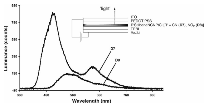
Figure 9. Electroluminescence spectra of D7 and D8 . Inset: schematic cross section of the fabricated OLEDs D7 and D8 , containing 7 ( R' = \text{CN} ) and 8 ( R' = \text{NO}_2 ) as the emissive layers, respectively.
