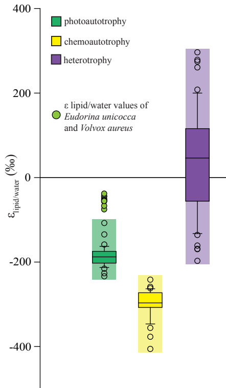
Figure 3: Box plots of D/H fractionations between the n C16:0 fatty acid and culture medium observed in different culture experiments. Cultures included from this study are Thiocapsa roseopersicina , Halochromatium glycolicum , Isochrysis galbana , Thiobacillus denitrificans and Pseudomonas str. LFY10. Additionally, published data for Isochrysis galbana , Ascophyllum sp., Alexandrium fundyense , Methylococcus capsulatus , Saragassum filicinum , Undararia pinnatifida , Binghamia californica , Gelidium japonica , Sporomusa sp., Botryococcus braunii , Eudorina unicocca , Volvox aureus , Desulfobacterium autotrophicum , Cupriavidus oxalaticus , Cupriavidus necator , Escherichia coli , Rhodospseudomonas palustris , Tetrahymena thermophile and Moritella japonica DSK 1 have been included (Sessions et al., 1999; Sessions et al., 2002; Chikaraishi et al., 2004; Valentine et al., 2004; Zhang and Sachs, 2007; Campbell et al., 2009; Zhang et al., 2009a; Dirghangi and Pagani, 2013b; Fang et al., 2014).
