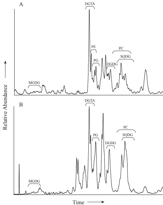
Figure 1: HPLC/ESI-MS base peak chromatogram of the Bligh Dyer extract of (A) the Schiermonnikoog microbial mat and (B) the Mokbaai sediment. monogalactosyldiacylglycerol (MGDG); digalactosyldiacylglycerol (DGDG); phosphatidylglycerol (PG); phosphatidylcholine (PC); phosphatidylethanolamine (PE); sulfoquinovosyldiacylglycerol (SQDG); G. diacylglyceryl-hydroxymethyl-trimethylalanine (DGTA). For structures of IPLs, see Figure 2.
