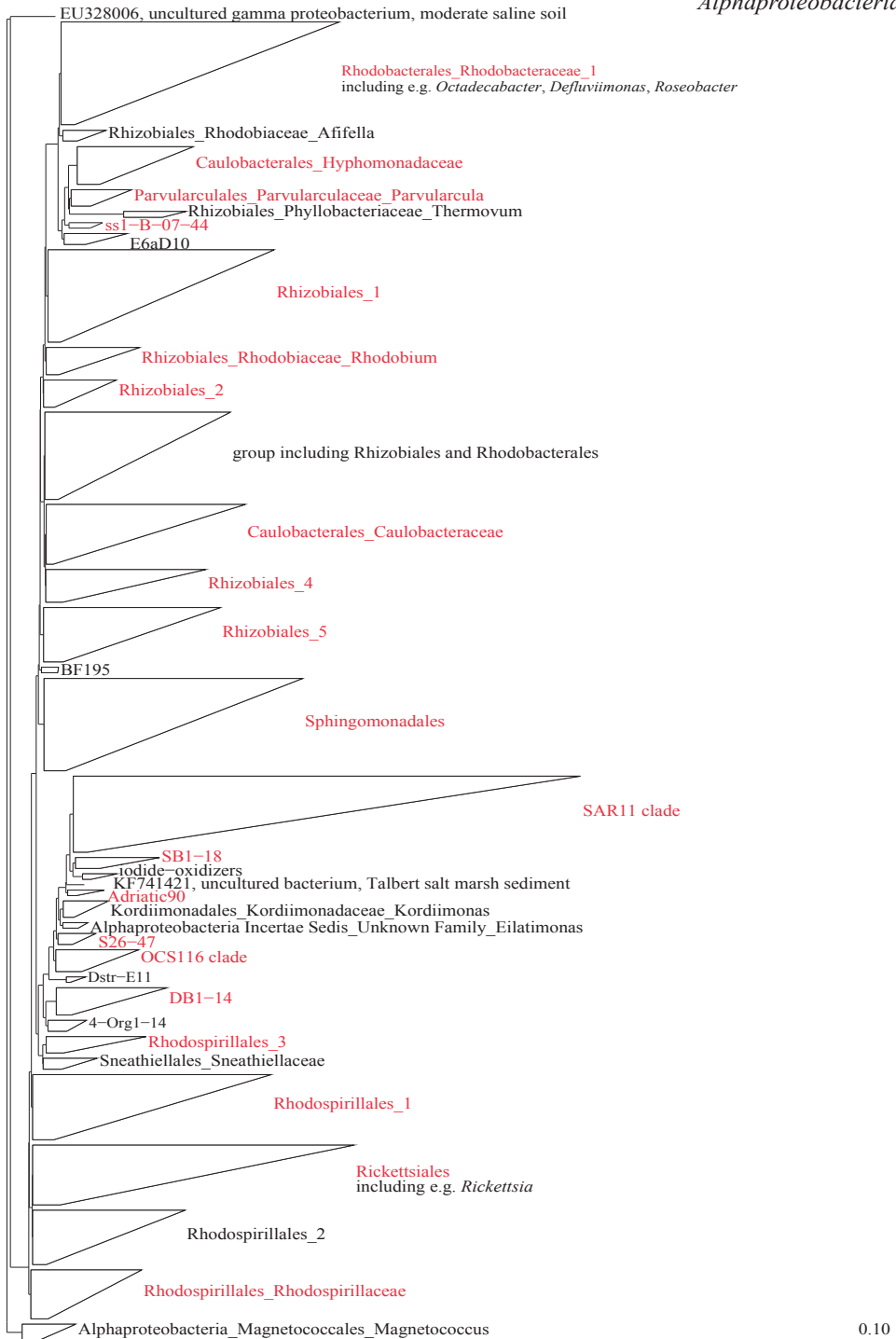
Figure S2: Phylogenetic tree of 16S rRNA gene sequence reads assigned to Alphaproteobacteria. Scale bar indicates 0.10 % estimated sequence divergence. Groups containing sequences are highlighted.
