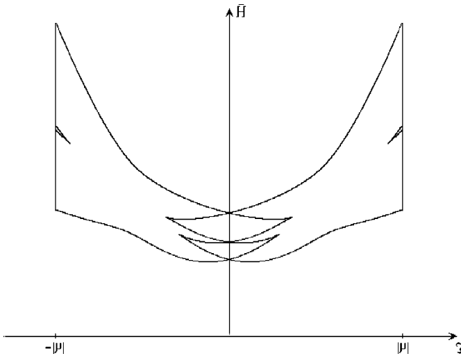
Fig. 2 A slice y_2 = |\mu| of the set of critical values of the energy-momentum mapping \mathcal{E}\mathcal{M} = (y, \bar{H}) with axes y_1 = \xi_3 and \bar{H} for the ‘middle’ case s_3 \cdot (\alpha, \beta, \gamma) \approx (a, b, c)
