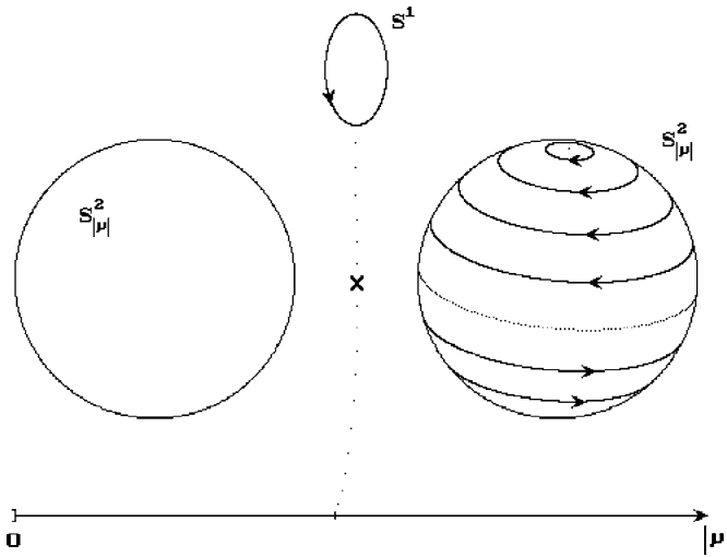
Fig. 1 Schematic representation of the bundle structure of the phase space \mathcal{P} = T^*SO(3) . The value y_2 = |\mu| = 0 is excluded from the picture, in this limit the product of the spheres with S^1 attached results in a fibre SO(3)
