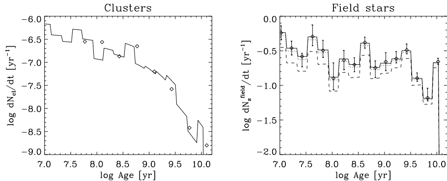
Figure 1. Age distributions of SMC clusters (left panel) and field stars (right panel). Diamonds denote observed values (left panel: Hodge 1987, right panel: Harris & Zaritsky 2004), while our model predictions are shown for infant mortality rates of f_{\text{IMR}} = \{0.6, 0.9, 0.995\} as dashed, dotted and solid lines, respectively. Error bars represent 2\sigma error margins.
