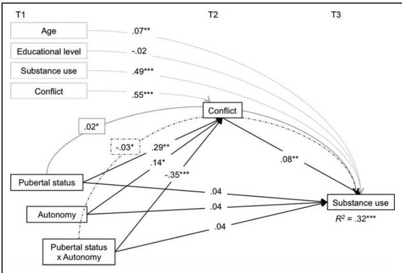
Figure 2. Standardized path coefficients for model with substance use (N = 1,844).
