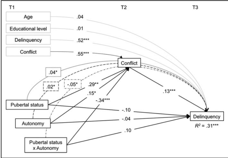
Figure 1. Standardized path coefficients for model with delinquency (N = 1,844).
