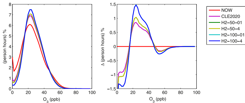
Fig. 9. Population exposed to different levels of O_3 for the whole LOTOS-EUROS domain. (left) Person hours versus O_3 level for the whole year, scaled by the total population in the domain and the total number of hours, and expressed in %. (right) Differences in person hours (%) between each scenario and the NOW scenario. Note that the y-values depend on the O_3 bin size; the O_3 bins used here are 2 ppb.
