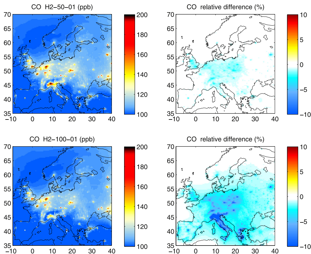
Fig. 3. CO mole fractions for the simulations with 50% (H2_50_01) and 100% (H2_100_01) H 2 cars (left panels), and the relative differences between these and the CLE2020 simulation (right panels). The figure shows annual means at ground level. Note that the color scales are different between left and right panels. (For interpretation of the references to colour in this figure legend, the reader is referred to the web version of this article.)
