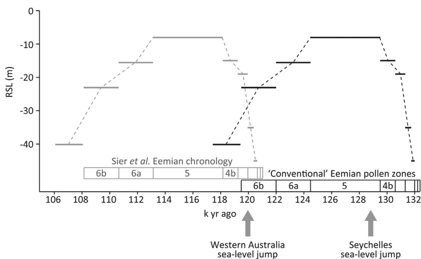
Fig. 7. The Zagwijn (1983) Netherlands sea level curve plotted against the established pollen zone chronology (in black) and Sier et al. (2015) chronology (in grey). The approximate timing of the Seychelles and Western Australia sea level jumps (as shown in Fig. 1 ) are marked.
