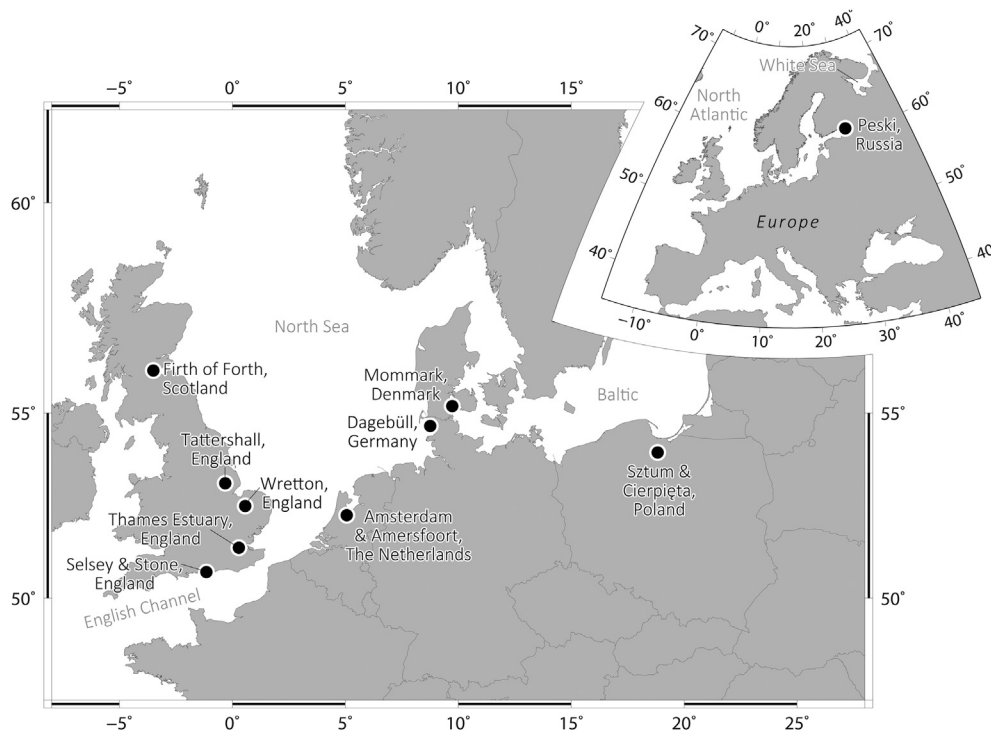
Fig. 3. Location map of Northwest Europe showing last interglacial site names referred to in the text.
