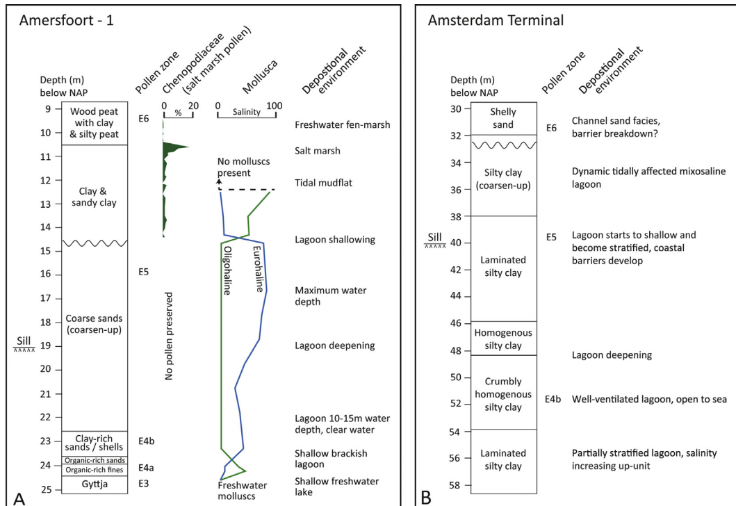
Fig. 6. Summary lithology and selected biostratigraphic data from the Amersfoort-1 and Amsterdam Terminal boreholes (modified from Van Leeuwen et al. (2000) and Cleveringa et al. (2000)).
