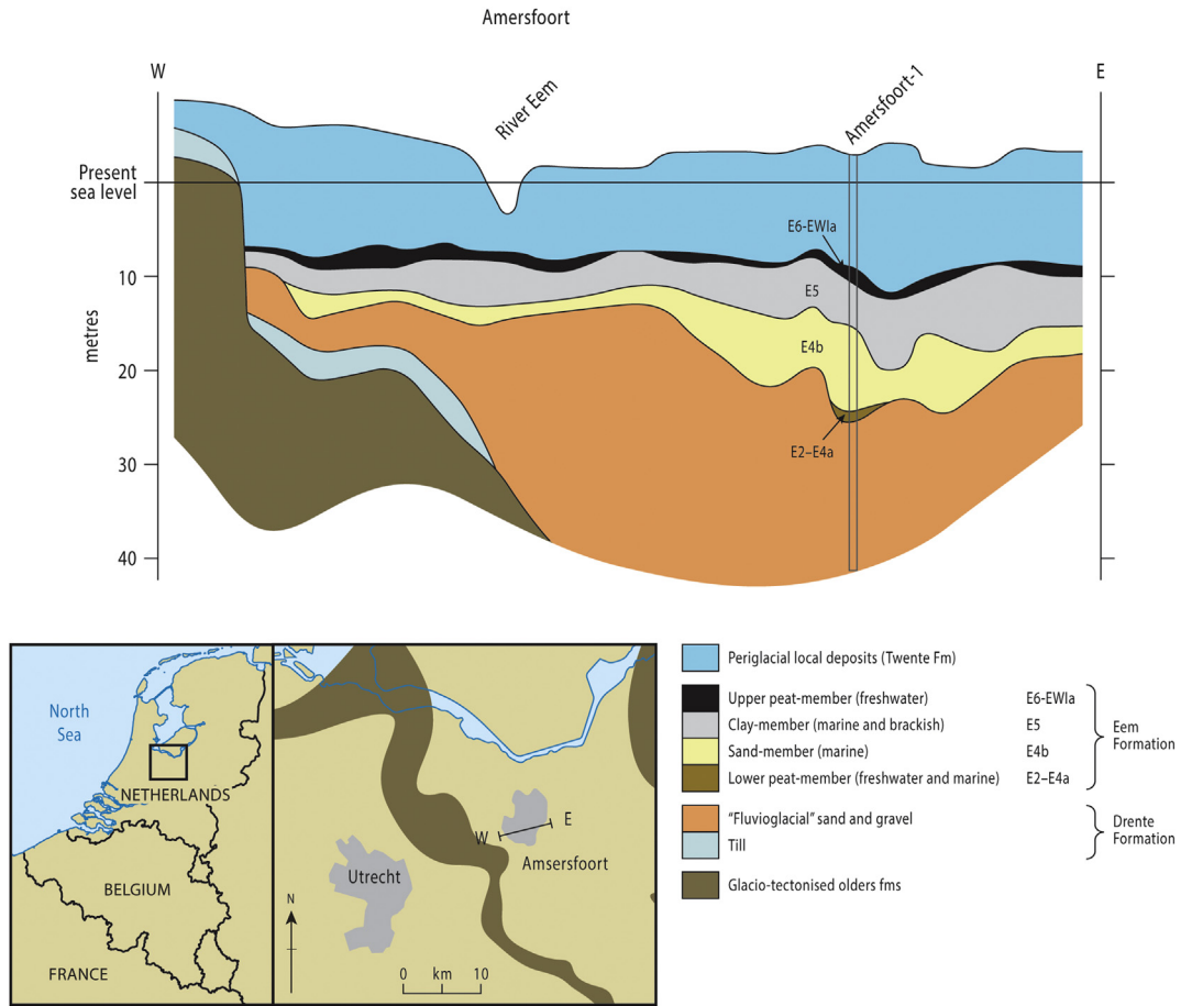
Fig. 5. Simplified lithostratigraphy in the Amersfoort Basin (modified from Zagwijn (1983)). Position of pollen zones are approximate, based upon Zagwijn (1983).
