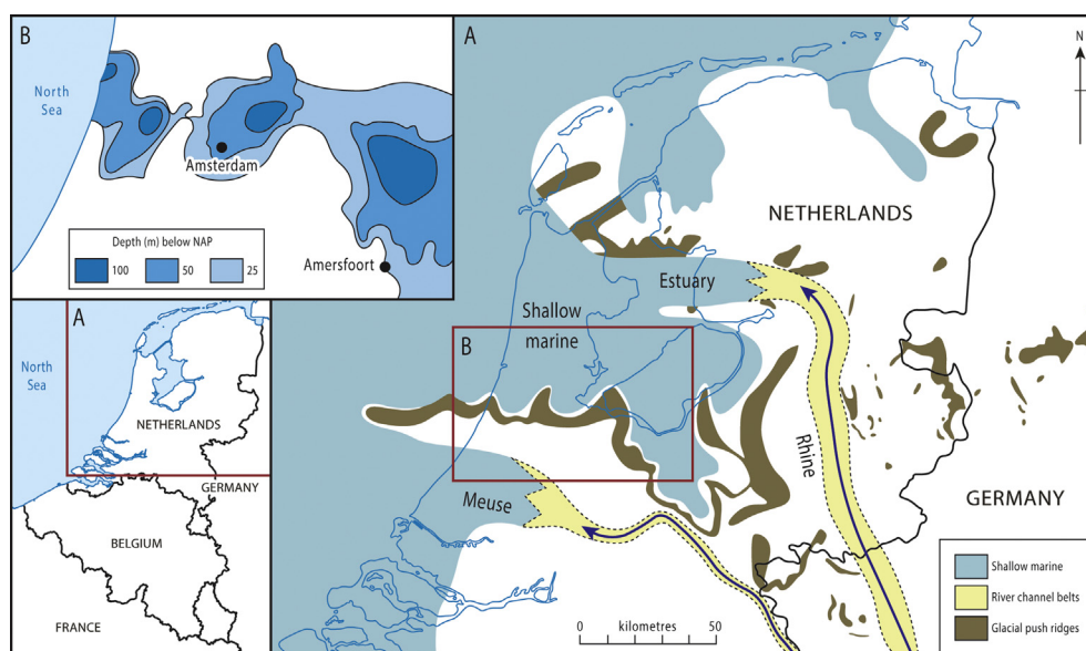
Fig. 4. Reconstruction depicting (A) the Last Interglacial coastal configuration in the Netherlands during the sea-level highstand (modified from Peeters et al. (2015)), (B) the glacial basins in the Netherlands (modified from Cleveringa et al. (2000)).
