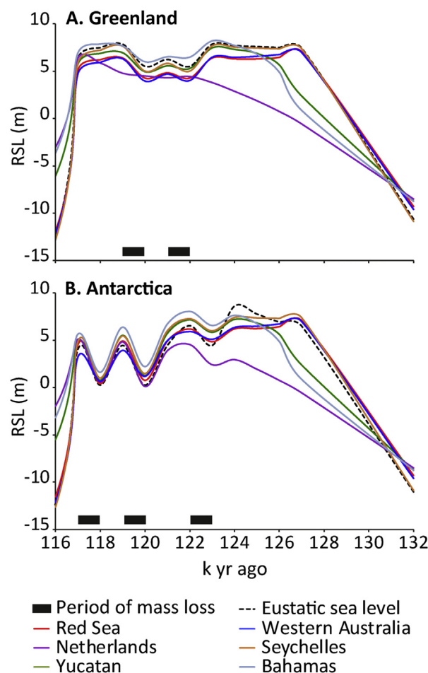
Fig. 8. Sea-level predictions associated with hypothetical collapse/regrowth cycles of the Greenland and Antarctic ice sheets. Experiments G1 and A1 assume that Greenland and Antarctica, respectively, are subjected to growth-collapse cycles with amplitudes that vary between c. \pm 2\text{--}3 and 5 m. A) Predictions assuming a Greenland-only origin for sea-level oscillations/jumps; B) Predictions assuming an Antarctic-only origin. Two periods of mass loss are shown for Greenland (122–121 k yr, 120–119 k yr) and three for Antarctica (123–122 k yr, 120–119 k yr, 118–117 k yr). Details of experimental set-up associated with each model are provided in Supplementary Information Table S1.
