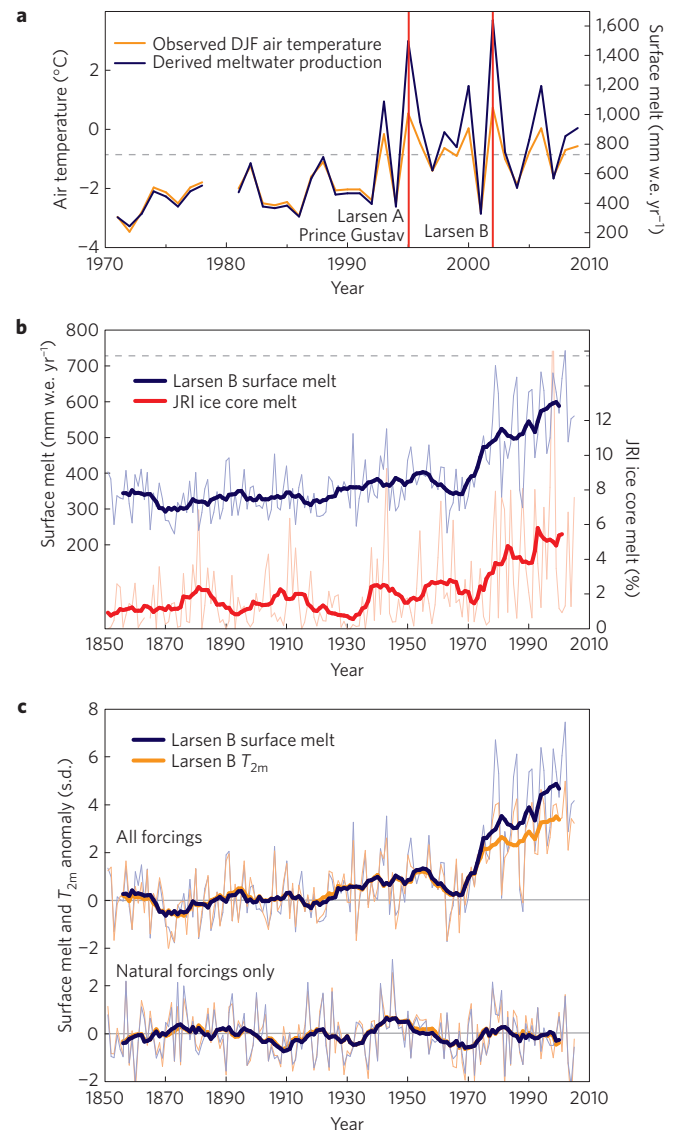
Figure 2 | Historical melt evolution before ice shelf collapse. a , Observed air temperatures at Marambio and derived melt levels. Vertical red lines show years of collapse for indicated ice shelves. b , Melt derived from GCM Ensemble simulations and an ice core record of past melt intensity from James Ross Island (JRI; melt as a percentage of annual accumulation) 11 . c , Anomalies (from 1851 to 1900) in melt and temperature from GCM Ensemble simulations including and excluding anthropogenic forcing. Bold lines (in b,c ) show 11-year centred moving averages. Dashed horizontal lines (in a,b ) show average pre-collapse melt on Larsen A and B simulated by RACMO2.
