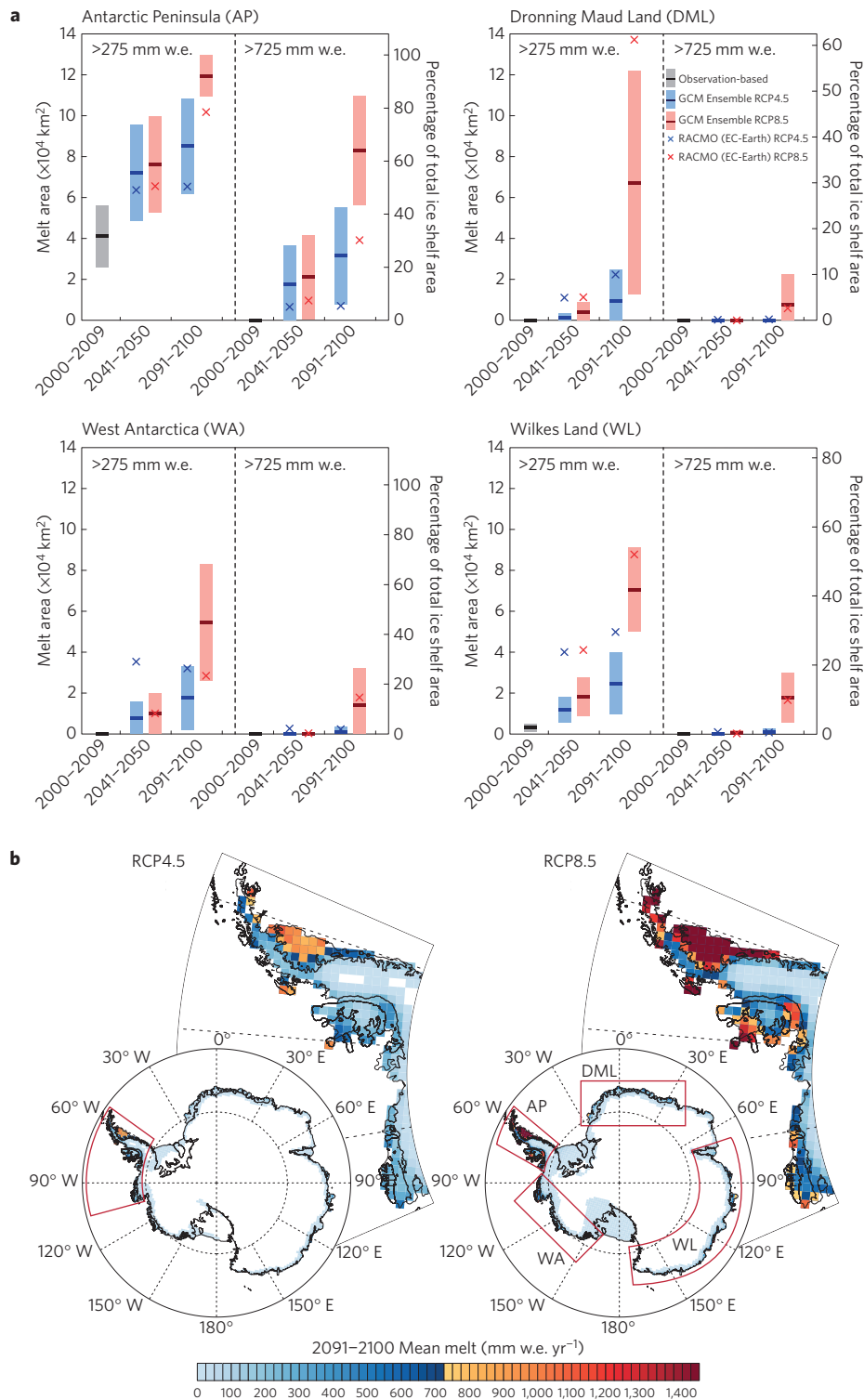
Figure 4 | Melt exceeding specific thresholds across time and space. a , Plots of regional ice shelf areas exceeding melt levels prevailing at present on high-melt AP ice shelves ( >275 mm w.e. \text{yr}^{-1} ) and associated with ice shelf collapses ( >725 mm w.e. \text{yr}^{-1} ). Regions indicated in b . b , Mean surface melting over 2091–2100 derived from the GCM Ensemble under RCP4.5 and RCP8.5. Enlarged maps show the AP and a portion of West Antarctica (map area indicated in red outline in the full RCP4.5 map). Boundary between blue and orange colours represents historical northeast AP collapse-associated melt level.
