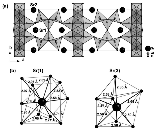
Fig. 10 (a) Unit cell of \text{Sr}_4\text{Al}_{14}\text{O}_{25} along the c -axis, (b) local coordination geometry environment of nonequivalent \text{Sr}^{2+} sites.
