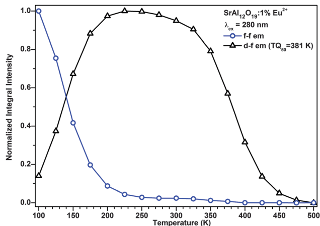
Fig. 4 The emission intensity dependence on temperature for the f–f and d–f emission in \text{SrAl}_{12}\text{O}_{19}:1\%\text{Eu}^{2+} .
