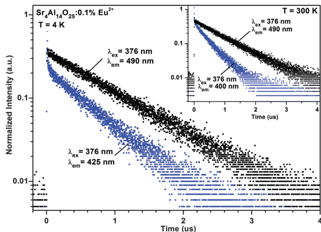
Fig. 15 Decay curve of \text{Sr}_4\text{Al}_{14}\text{O}_{25}:0.1\%\text{Eu}^{2+} at 4 K at emission wavelengths indicated in the figure. The inset shows decay curve of \text{Sr}_4\text{Al}_{14}\text{O}_{25}:0.1\%\text{Eu}^{2+} at 300 K.
