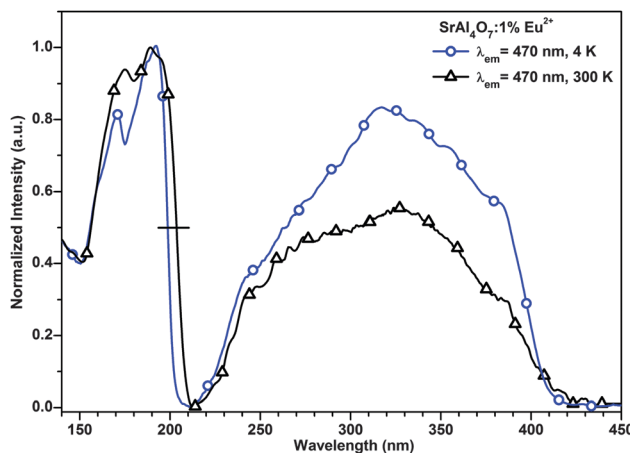
Fig. 7 Excitation spectra of \text{SrAl}_4\text{O}_7:1\%\text{Eu}^{2+} at 4 K and 300 K recorded at 470 nm.
