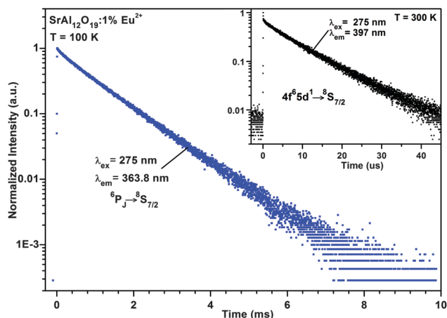
Fig. 5 Decay curve of the emission band originating from the {}^6\text{P}_J-{}^8\text{S}_{7/2} transition at 100 K. The inset shows the decay curve of the 4\text{f}^6 5\text{d}^1-{}^8\text{S}_{7/2} emission at 300 K.
