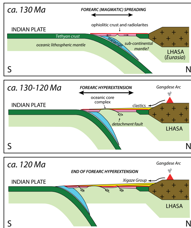
Figure 2. Schematic model (not to scale, not balanced) for forearc hyperextension in the south Tibetan ophiolites. The main extensional phase in the forearc occurred at 130–120 Ma, synchronous with the initial input of the Xigaze Group forearc sediments. This caused detachment faulting, crustal attenuation, and mantle uplift to the seafloor. Forearc hyperextension stopped ca. 120 Ma, and was followed by continuous sedimentation of the Xigaze Group, which unconformably covered the dismembered ophiolite. The dynamics of the subducting slab during forearc hyperextension did not affect the magmatic activity at the Gangdese arc, which persisted from the Early Cretaceous until the Eocene.
