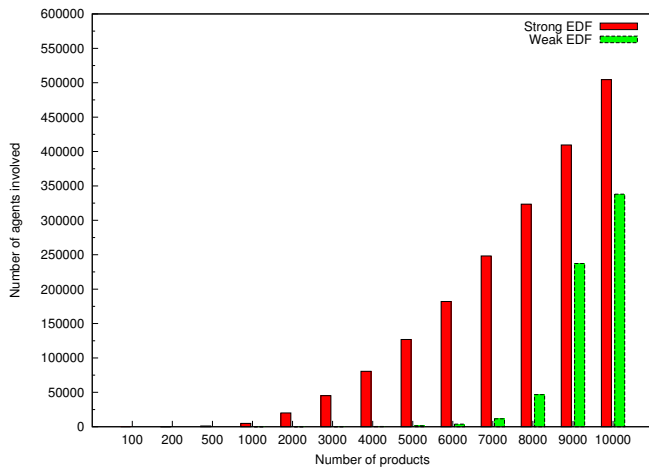
Figure 22: Number of agents involved for strong and weak EDF.
