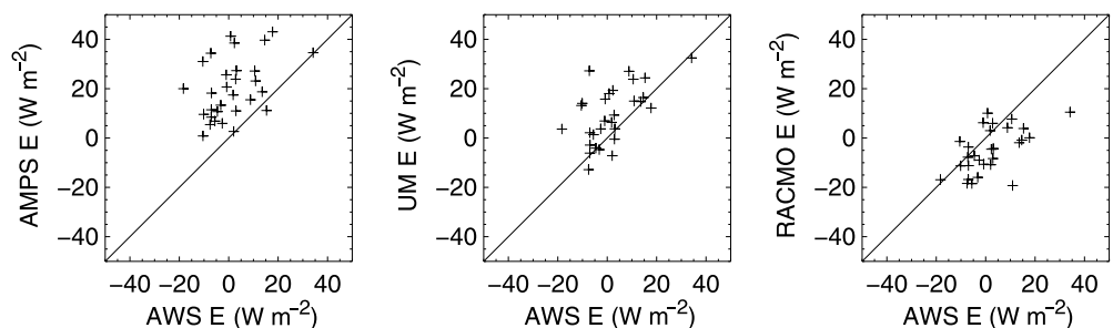
Figure 5. As in Figure 2 but for daily mean net surface energy flux, E .
