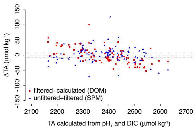
Figure A1. Differences in total alkalinity ( \Delta\text{TA} ; \mu\text{mol kg}^{-1} ) measured on unfiltered and filtered ( 0.45\ \mu\text{m} ) samples (blue triangles; representing the effect of particles) and between TA measured on filtered seawater and TA calculated from DIC and \text{pH}_T (red squares; representing potential organic alkalinity), plotted as a function of TA calculated from DIC and \text{pH}_T . The dotted lines indicate the typical standard deviation of the difference between two measurements.
