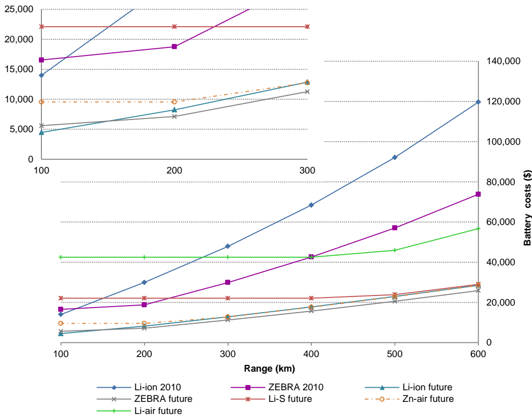
Figure 6: Battery cost as a function of the driving range.
