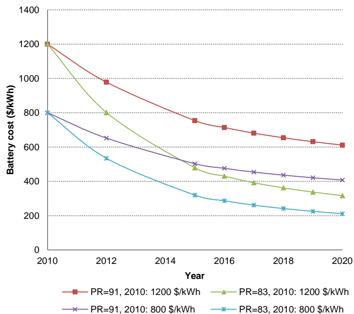
Figure 3: Li-ion cost scenarios based on market projections and assessment of progress ratios.
