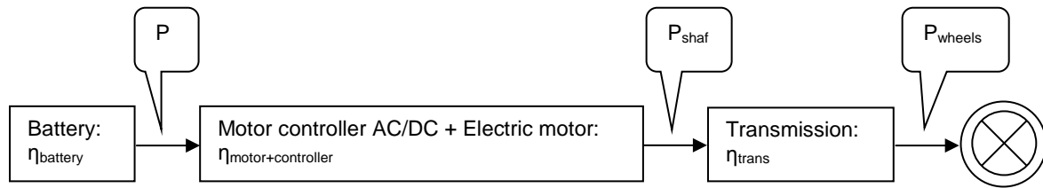
Figure 1: Main elements and power flow inside a battery electric vehicle, adapted from Campanari et al. [3]
