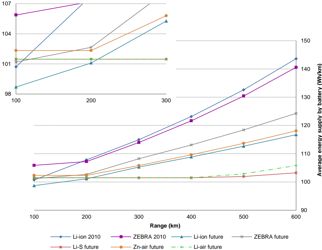
Figure 7: Energy consumption of the drive train (energy delivered by the battery) as a function of the driving range.
