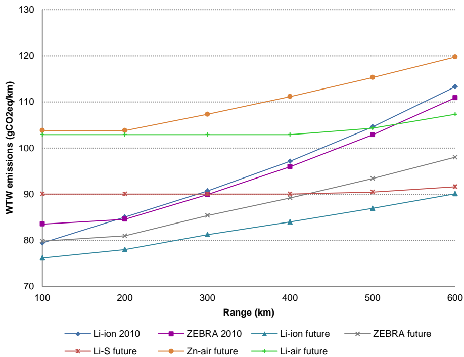
Figure 9: WTW emissions (European electricity mix) of the battery electric car as a function of the driving range. Energy consumption for heating of the ZEBRA batteries (when not in operation) is not included.
