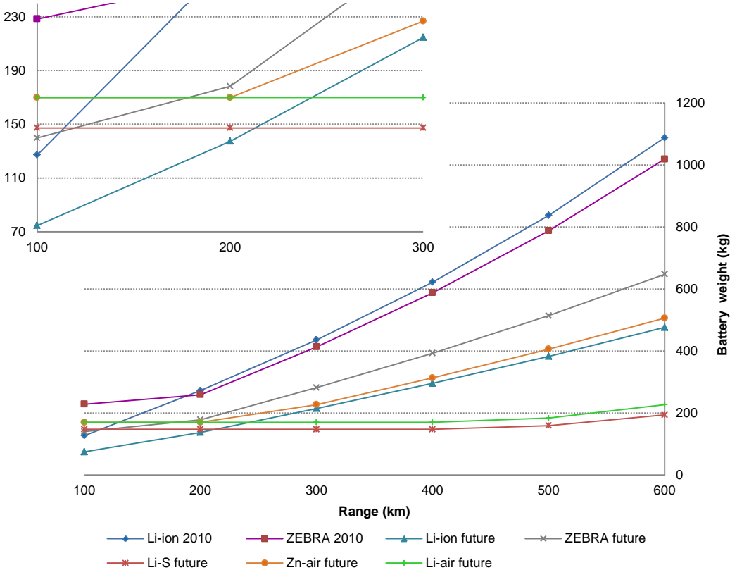
Figure 5: Battery weight as a function of the driving range.
