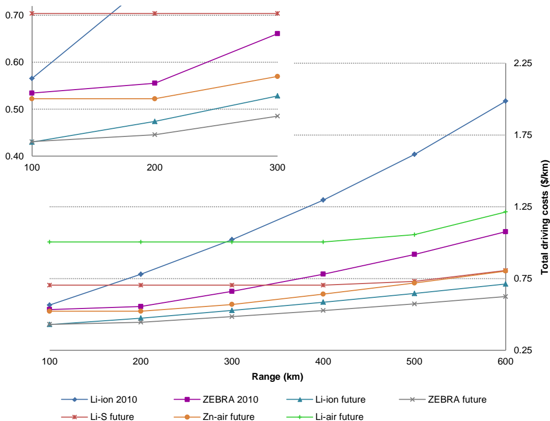
Figure 10: Total driving costs of the battery electric car, considering a number of present and future battery technologies (at an electricity price 0.15-0.30 $/kWh, including taxes [96])
