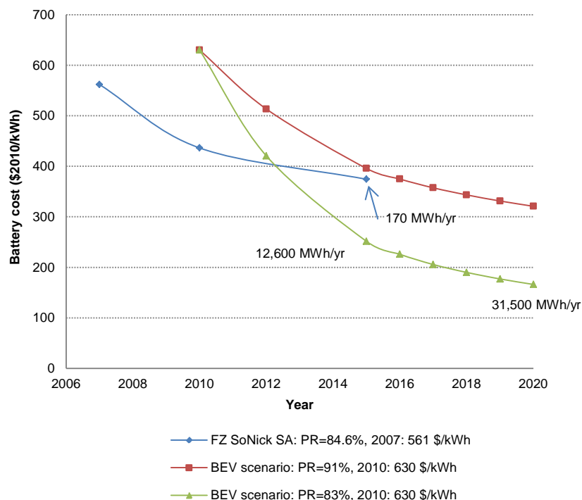
Figure 4: ZEBRA battery cost scenarios, based on cost data from Kalhammer et al. [8]. Blue line: based on production capacity goals of FZSoNick [76]; red and green line: based on cumulative production volume of 7.1 million batteries in 2020. Annual production capacities in 2015 and 2020 are given for FZSoNick and BEV scenarios.
