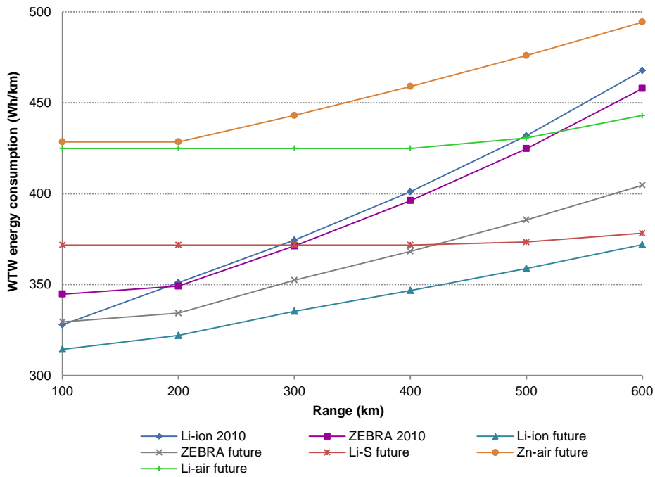
Figure 8: WTW energy consumption of battery electric car as a function of the driving range. Energy consumption for heating of the ZEBRA batteries (when not in operation) is not included.
