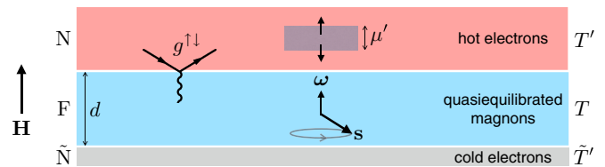
FIG. 1. (Color online) Schematic of the proposed heterostructure. On the top, the normal metal N, with electron temperature T' , provides spin torque through spin accumulation \mu' = \mu'z at the interface with the ferromagnet (F). The F is assumed to be sufficiently thin such that its magnon temperature T is uniform throughout. Collective spin density \mathbf{s} in the F precesses with frequency \omega , which is controlled by the applied field \mathbf{H} , both pointing in the z direction. Electron-magnon interaction at the N|F interface is parametrized by the spin-mixing conductance g^{\uparrow\downarrow} . The normal metal \tilde{N} is a poor spin sink, which can, nevertheless, drain energy from magnons and phonons in the ferromagnet.
