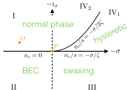
FIG. 3. (Color online) Phase diagram for the solutions of Eqs. (27) and (28) for n_c in the abstract (\sigma, \iota_x) space. O stands for the unperturbed (i.e., thermal-equilibrium) point, while P is the critical point for a driven system. The solid lines, \iota_x = 0 and \iota_x = -\sigma^2/4\zeta , trace out phase transitions between distinct dynamic states: second-order transition between the NP and BEC (I/II boundary) and hysteretic first-order transitions at the IV 2 /IV 1 and IV 1 /III boundaries, where the normalized condensate density, n_c/s , jumps by -\sigma/2\zeta and -\sigma/\zeta relative to 0, respectively. The condensate associated with these first-order transitions is interpreted to be “swasing” [12].
