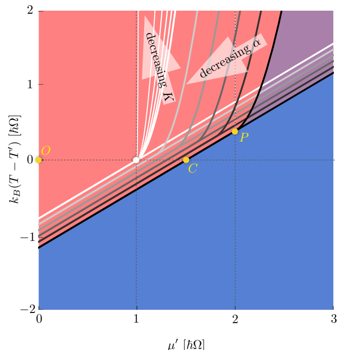
FIG. 5. (Color online) Effects of intrinsic damping \alpha/\alpha' (starting at 1 and decreasing to 0 in increments of 0.2) and nonlinearity K/\hbar\Omega (going from 1 to 0 in increments of 0.2), while keeping \hbar\Omega fixed, on the phase-diagram structure, using Eqs. (37) and (38). Decreasing Gilbert damping \alpha [which lowers the swasing threshold (35)] increases the size of the condensate regions, while decreasing anisotropy K increases the size of the hysteretic region [as is evident from Eq. (38)].
