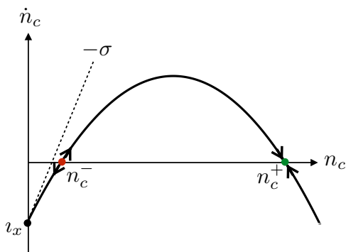
FIG. 2. (Color online) Graphical representation for obtaining solutions (36) to the equation \hbar \dot{n}_c = i with i given by Eq. (28). Here, \sigma < 0 and \iota_x < 0 (corresponding to region IV 1 , as described in the text), resulting in two fixed points: unstable at n_c^- and stable at n_c^+ .
