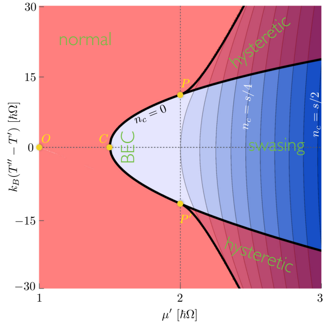
FIG. 6. (Color online) Phase diagram with a floating magnon temperature T and density determined by the conditions i = 0 and j = 0 . Here, \alpha/\alpha' = 1 , K = \hbar\Omega , s(A/\hbar\Omega)^{3/2} = 10^4 , and k_B T'' = 10^2 \hbar\Omega , similarly to the other plots.
