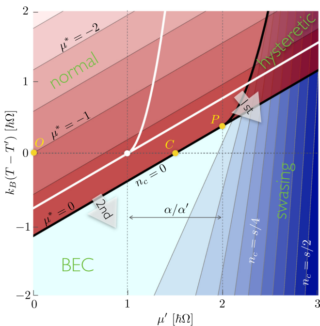
FIG. 4. (Color online) Physical phase diagram in the presence of anisotropy K = \hbar\Omega at k_B T = k_B T'' = 10^2 \hbar\Omega , s(A/\hbar\Omega)^{3/2} = 10^4 , and \alpha/\alpha' = 1 (black curves), calculated using the linearized current i_x in Eq. (28) [see discussion preceding Eq. (37)]. The white curves show the idealized \alpha/\alpha' = 0 case. The analytically evaluated diagram shown here is essentially indistinguishable from the numerical diagram (not shown) produced by the exact expression for i in Eq. (28). The phase-transition lines and crossovers that delineate different dynamic regimes can be inferred from Fig. 3.
