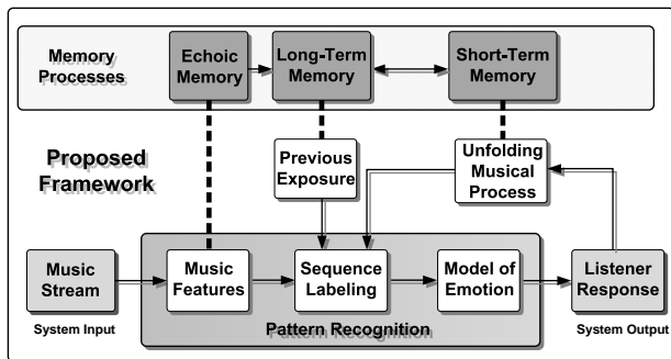
Figure 2: The proposed framework for MER. The blocks are system components and the arrows indicate the flow of information. In the shaded area is pattern recognition, and outside are the proposed processes, namely, the “unfolding musical process” and the listener’s “previous exposure”. The figure also illustrates how the organization of auditory memory is related to system blocks.
