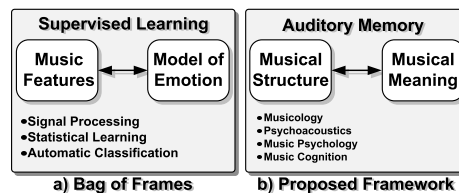
Figure 1: Approaches to MER. Part a) illustrates the BOF approach, which uses machine learning to map music features to a region of a model of emotion. Part b) illustrates the proposed approach, which relies on the organization of auditory memory to estimate musical emotions as a form of musical meaning emerging from musical structure.
