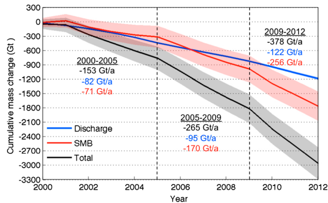
Figure 3. (black) Cumulative mass change due to (blue) discharge change with respect to 1996 and (red) surface mass balance change with respect to the 1961–1990 mean. Shading indicates uncertainty. Discharge uncertainty is shown but is visually indistinguishable. Text indicates the trend in the (black) total mass loss rate, (blue) discharge, and (red) surface mass balance during the 2000–2005, 2005–2009, and 2009–2012 periods.
