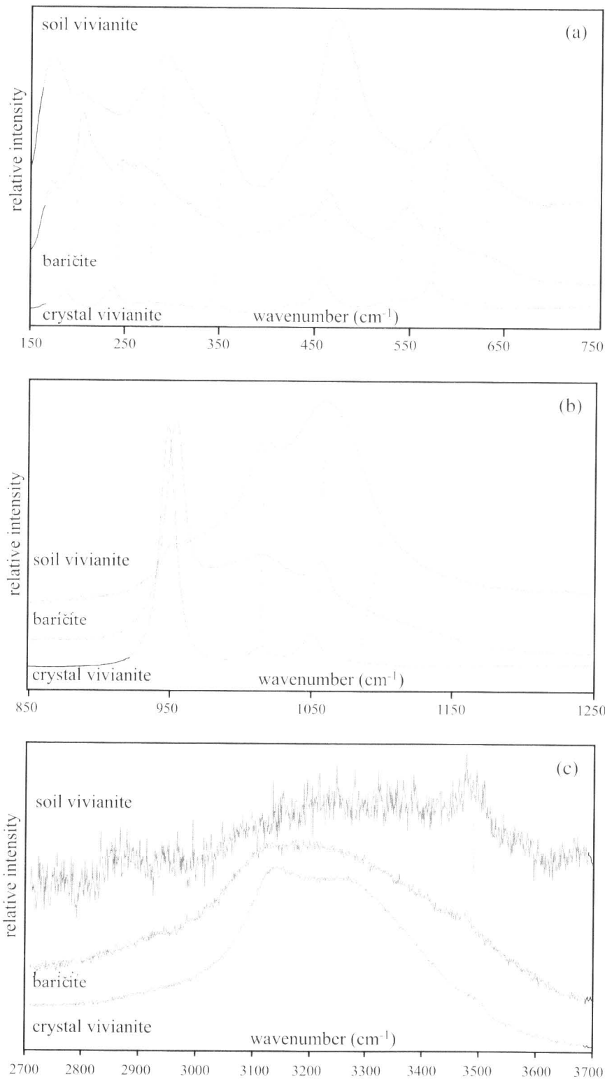
Fig 2. Raman spectra of soil vivianite, single crystal of pure vivianite and baričite in the regions (a) 150-750 cm -1 , (b) 850-1250 cm -1 and (c) 2700-3700 cm -1 .
