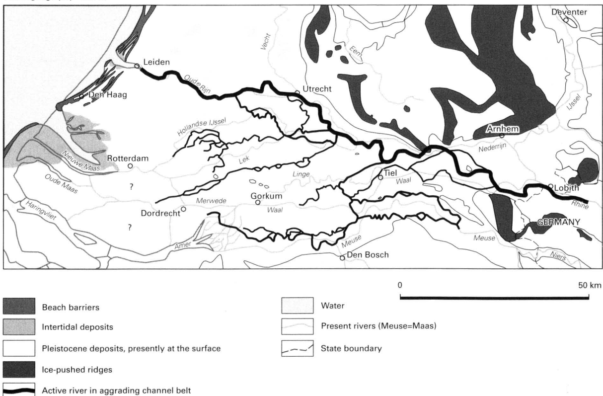
Fig. 9. Palaeogeography around 4000 yr BP: main discharge of the Rhine followed the Utrecht river system. There were some smaller channels branching off to the SW. The River Meuse (=Maas) closely followed the southern margin of the Late Weichselian valley. The exact location of river courses south of Rotterdam is unknown, partly because of later erosion.
