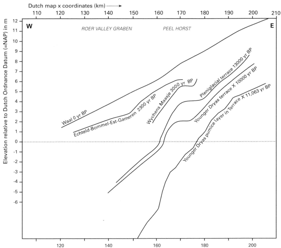
Fig. 4. Gradient lines of the Younger Dryas pumice layer (after Verbraeck 1990), the top of Late Weichselian terraces, and the top of Holocene channel belts crossing the Peel Horst, plotted along an E-W axis (after Stouthamer and Berendsen 2000). The influence of differential tectonic movements of the Peel Horst and Roer Valley Graben on gradient lines is evident.
