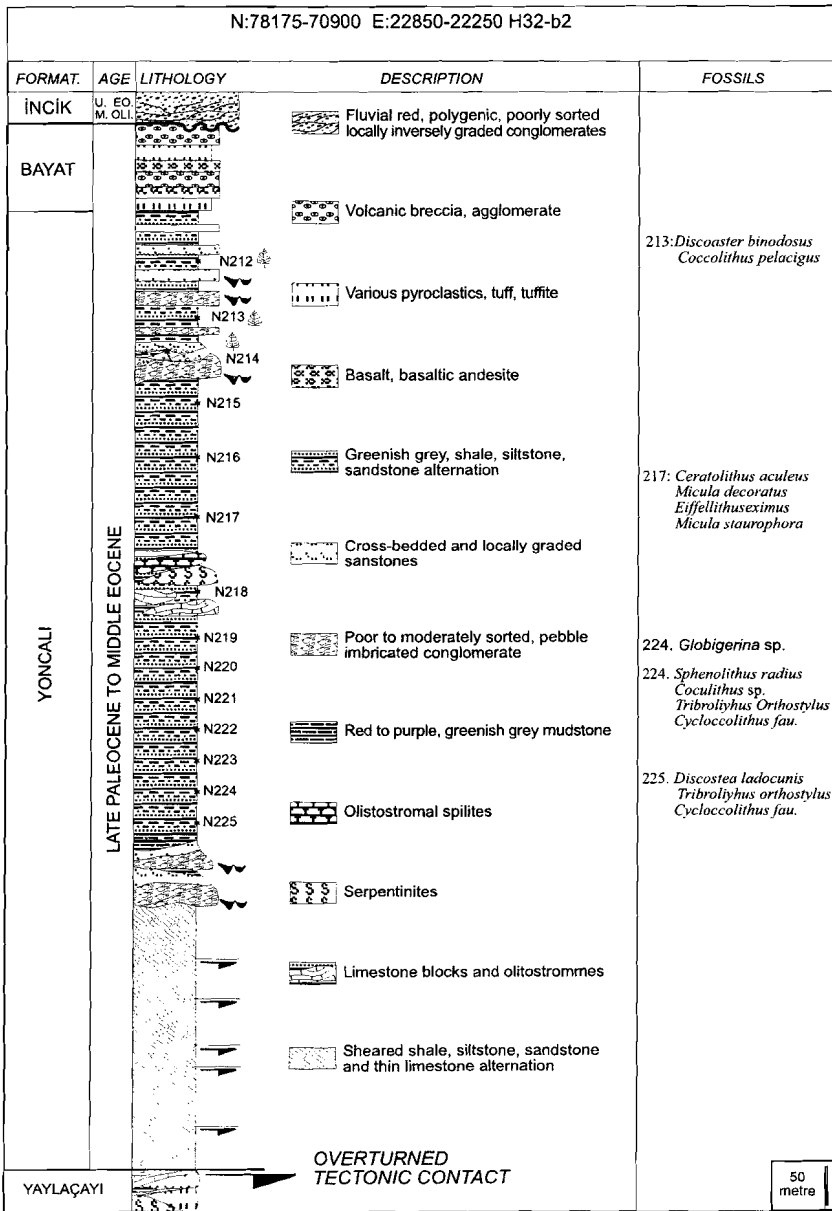
Figure 3.14 Measured stratigraphical section for the Yoncali and the Bayat formations. The coordinates at the top of the figure are the beginning and ending northing (N) and easting (E) for the stratigraphic section (UTM based Turkish Grid).
