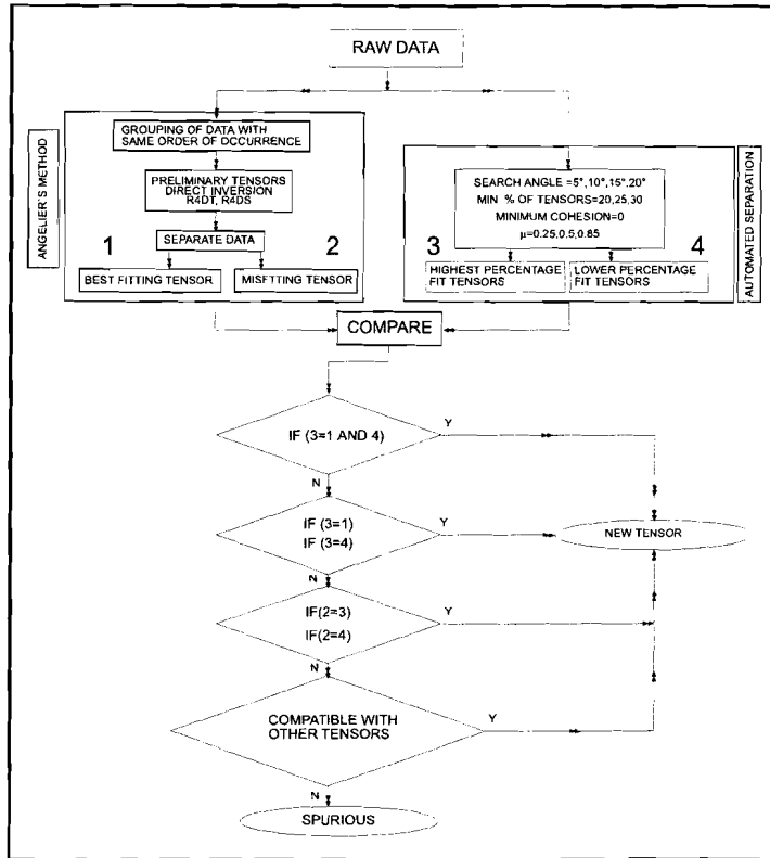
Figure 5.05 A flowchart of steps followed during the analysis of the data. The data was analyzed independently using two different methods then they were compared. After determination of the tensors and separation of the data into best fitting and tensor of miss-fitting faults, the results were compared with the automated method. If best-fitting and miss-fitting tensors of Angelier's method fall within the highest percent fit tensors of automated method, each subset is ascribed into two separate acceptable tensors. If not, and if they fall within the lower percentage fit tensors, then further analysis was carried out until reasonable and acceptable tensors were obtained (lowest miss-fit angles that was less than 15^\circ was obtained for all the groups. Only faults with more than 45^\circ were accepted spurious (less than 2% of whole data). This process is repeated for each class of structures (number of relative chronology) for each phase and for determining mean regional (sub-area based) stress tensor configurations.
