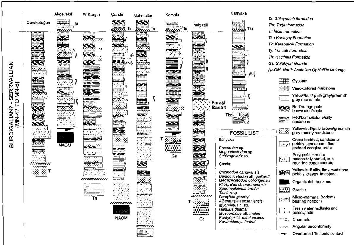
Figure 4.10 Correlation chart for the measured sections of the Çandır Formation. The relative position of the Faraşlı Basalt is extrapolated in the Inelgazlı section (see Figures 4.04, 4.11, 4.12, and 4.13 for the locations of the sections).
