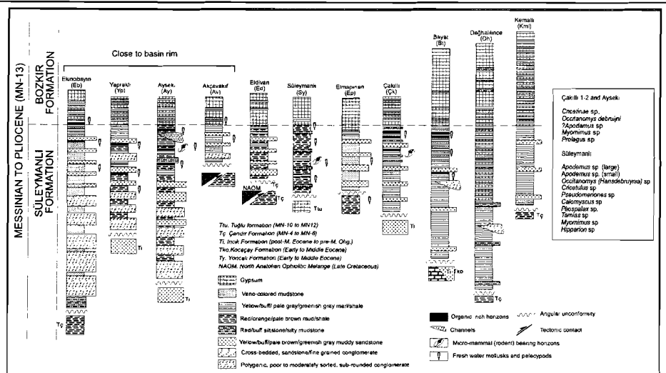
Figure 4.16 Correlation chart of the measured sections of the Süleymanlı and Bozkır formations (see Figures 4.05,4.12,4.13 and 4.14 for the location of the sections).
