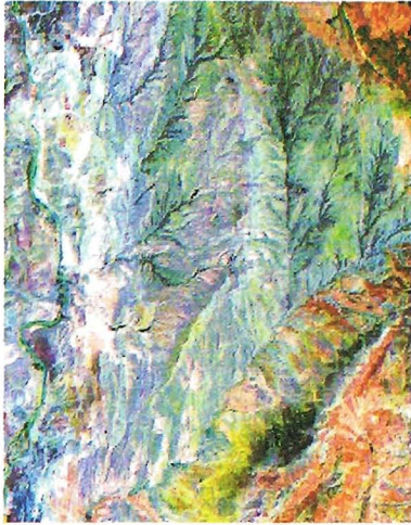
Decorrelation stretch R:7, G:4, B:1
