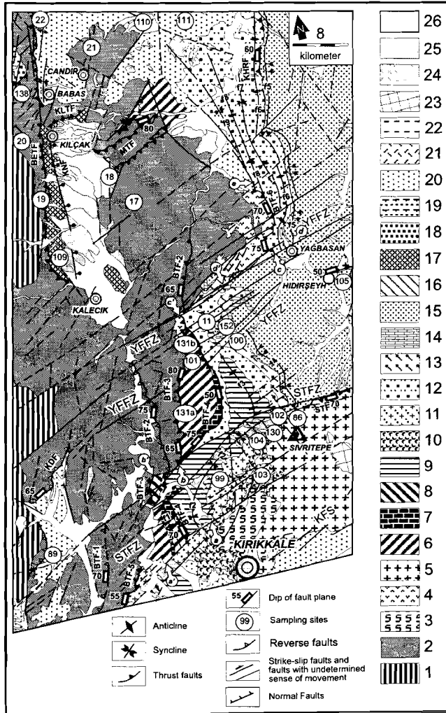
Figure 6.04 Geological map and sample locations for the sub-area 5. 1.Karakaya Complex, 2. North Anatolian Ophiolitic melange (NAOM), 3. ophiolitic units of the Kırşehir Block, 4. quartz-lalite member of the NAOM, 5. Sulakyurt Granitoids, 6. Dizilitaşlar Formation, 7. D3-member of the Dizilitaşlar Formation, 8. Dizilitaşlar and Hacıhalil formations (undifferentiated), 9.Yoncalı Formation, 10. Karagüney Formation, 11. Mahmatlar Formation, 12. Karabalçık Formation, 13. Osmankahya Formation, 14. Kocaçay Formation, 15. Incik Formation, 16. Güvendik formation, 17. Kılçak Formation, 18. Aslantaş Formation, 19. Hancılı Formation, 20. Çandır Formation, 21. Faraşlı Basalt, 22. Tuğlu formation, 23. Süleymanlı formation, 24. Bozkır Formation, 25. Deyim Formation, 26. Alluvium (see Figure 6.03 for the ages of these units).
