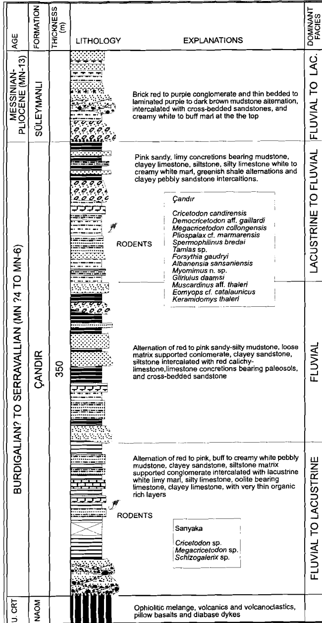
Figure 4.09 Generalized section of the Çandır Formation (fossil lists are from Çandır and Sanyaka locations, see Figures 4.05 and 4.13 for the sample locations).
