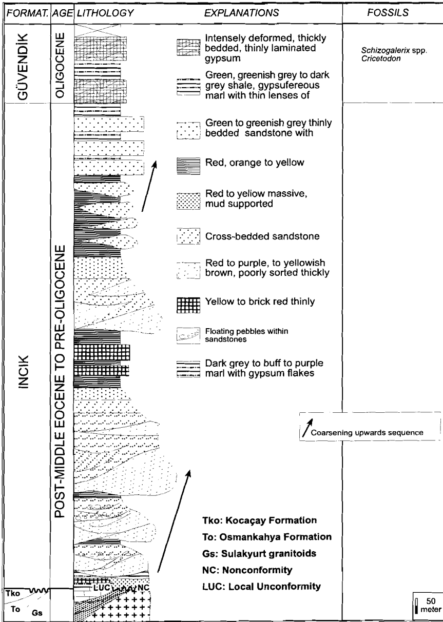
Figure 3.20 Generalized stratigraphical section for the Incik and Guvendik formations (Incik formation is partly modified after Dellaloğlu et al. 1992)
