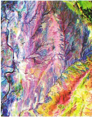
Figure 2.05 Various band combinations of the decorrelation stretch enhancement technique for a part of the Çankırı Basin (see Figure 2.03a for the location).
