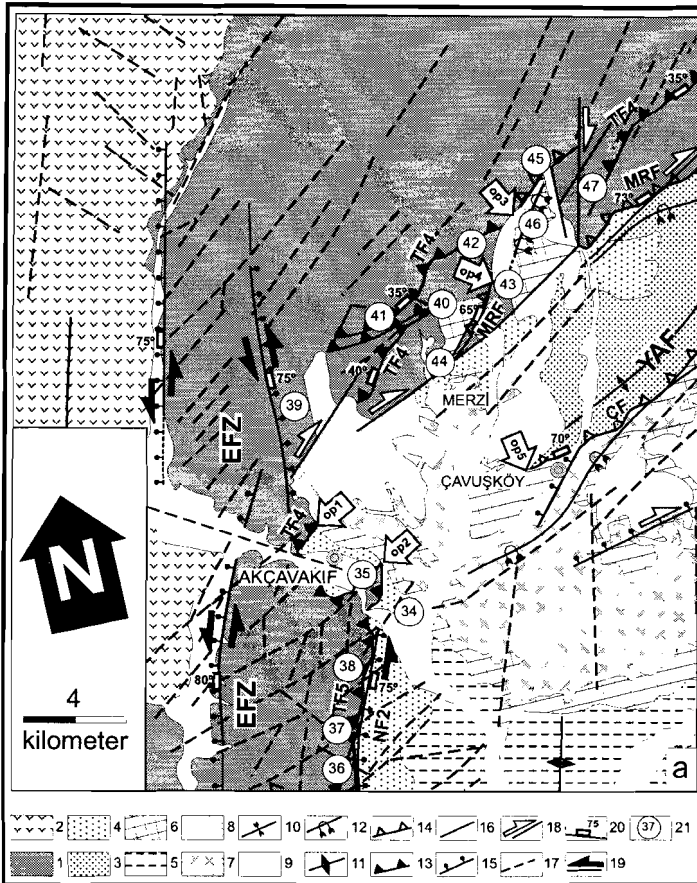
Figure 5.08 a) Geological map and sample location for the sub-area 3. EFZ: Eldivan Fault Zone, O.P. observation point (see text) 1. NAOM, 2. Galatean Volcanic Province (see Tankut et al 1995 and Toprak et al. 1996), 3. İncik Formation, 4. Çandır Formation, 5. Tuğlu formation, 6. Süleymanlı formation, 7. Bozkır Formation, 8. Deyim Formation, 9. Alluvium, 10. syncline, 11. anticline, 12. overturned syncline, 13. thrust faults, 14. reverse faults, 15. faults with normal sense of movement, 16. strike-slip or faults with unknown sense of movement, 17. photo-lineaments, 18. faults with dextral strike-slip sense of movement, 19. faults with sinistral strike-slip sense of movement, 20. Dip of faults where they are best observed in the field, 21. sample site locations. Plots of fault planes, slickenlines and stress orientations for each site (b-e) and whole data in a particular phase and sub-area (f-i) (lower hemisphere equal area projection).
