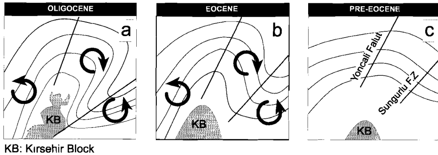
Figure 7.06 Back rotation of rim of the Çankırı Basin. Note northwards convex outline of the basin in pre-Eocene. Note pre-Eocene curved outline of the Çankırı Basin after back rotation of its margins
