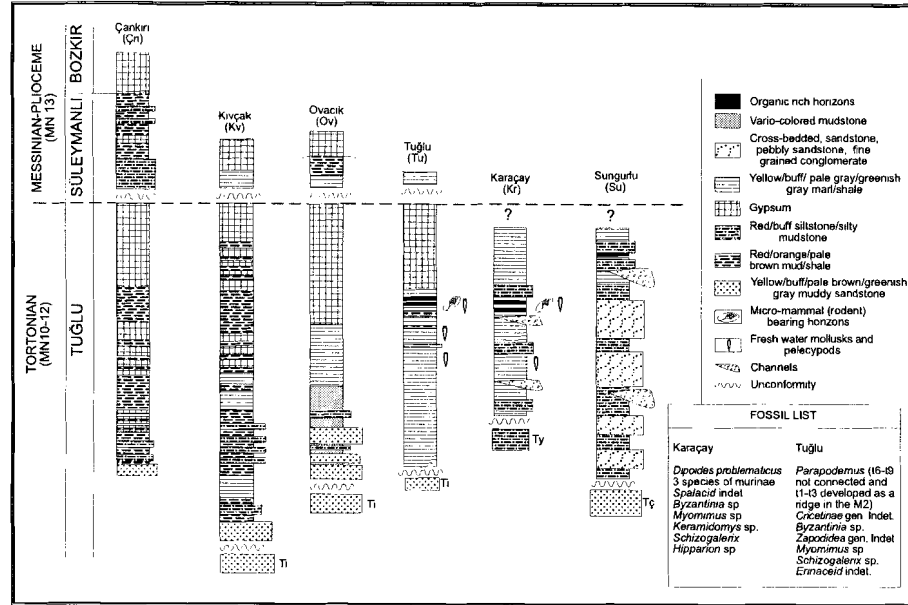
Figure 4.15 Correlation chart for the measured sections of the Tuğlu formation (see Figures 4.12, 4.13 and 4.14 for the location of the sections).
