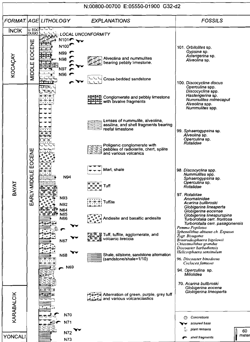
Figure 3.18 Measured stratigraphical section for the Karbalçık, Bayat and the Kocaçay formations (compare the stratigraphical positions of Bayat and other units with the Figures 3.13 and 3.14). The coordinates at the top of the figure are the beginning and ending northing (N) and easting (E) for the stratigraphic section (UTM based Turkish Grid).
