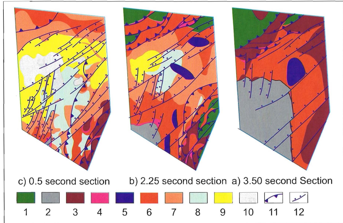
Figure 2.14 Time sections produced from the volume model. 1. Late Cretaceous units, 2. Basement (Kırşehir Block), 3. Tertiary clastics, 4. Kocaçay Formation, 5. Salt bodies, 6. lower part of the Incik Formation, 7. upper part of the Incik Formation, 8. Oligocene evaporites (Güvendik Formation), 9. Middle Miocene to Tortonian units, 10. Late Miocene units, 11. Thrust faults 12. normal faults.
