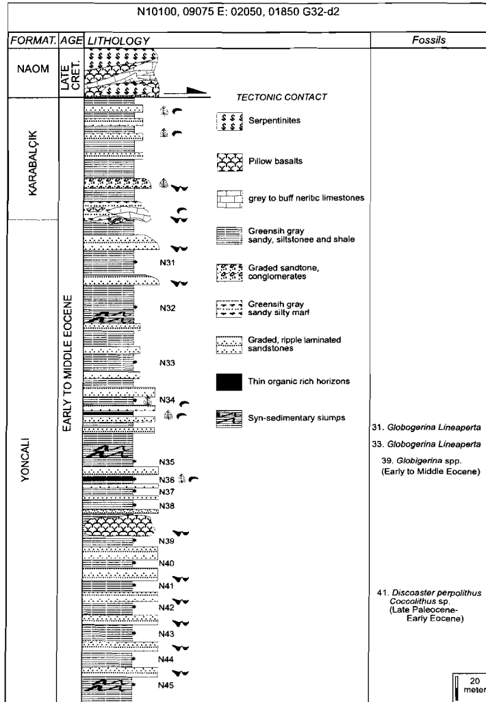
Figure 3.13 Measured stratigraphical section for the Yoncalı and Karabalçık formations. The coordinates at the top of the figure are the beginning and ending northing (N) and easting (E) for the stratigraphic section (UTM based Turkish Grid).
