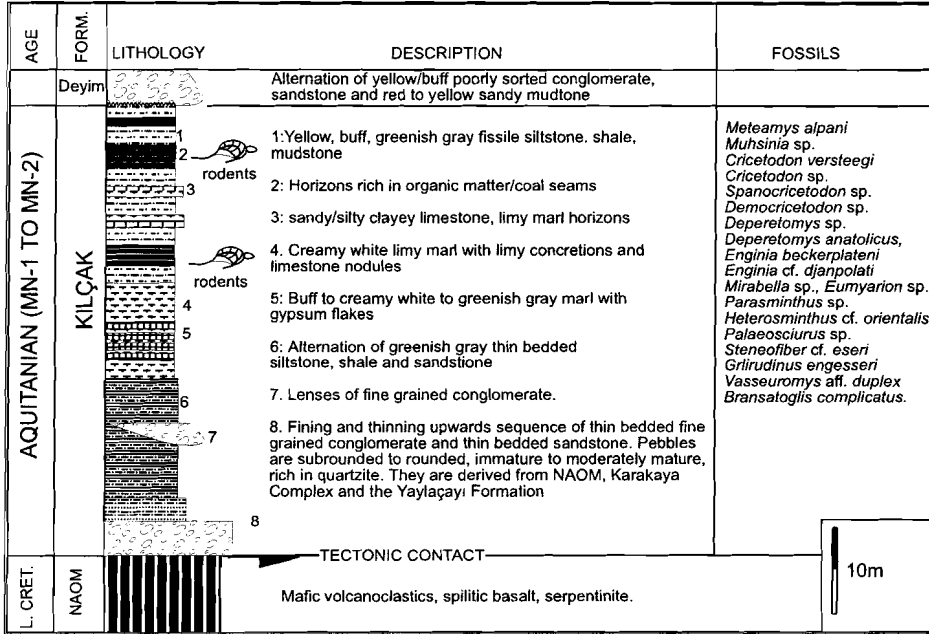
Figure 4.06 Generalized section of the Kılçak Formation (partly modified from Koçyiğit et al. 1995)
