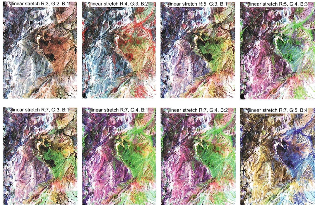
Figure 2.04 Simple linear stretch enhancement technique applied to various band combinations of the Landsat TM image for a part of the Çankır Basin (see Figure 2.03a for the location).
