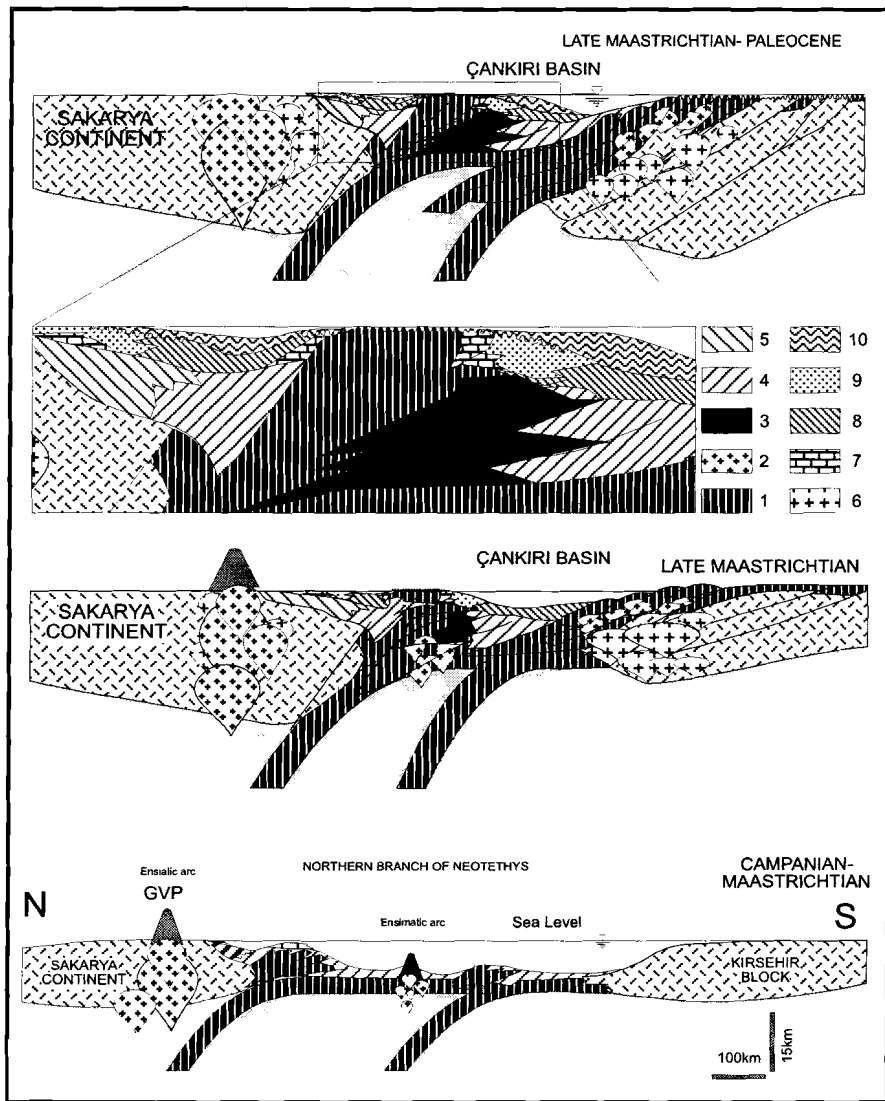
Figure 3.27 Conceptual, scenarios for the Late Cretaceous to Paleocene evolution of the northern branch of the Neotethys. 1. oceanic crust and ophiolites, 2: arc granites, 3: Island arc, 4. Yaylaçayı Formation, 5. Yapraklı Formation, 6. Collision granites, 7. Maliboğazı Formation, 8. Bağın formation, 9: Kavak formation, 10. Diziltaşlar Formation (modified after references cited in the text).
