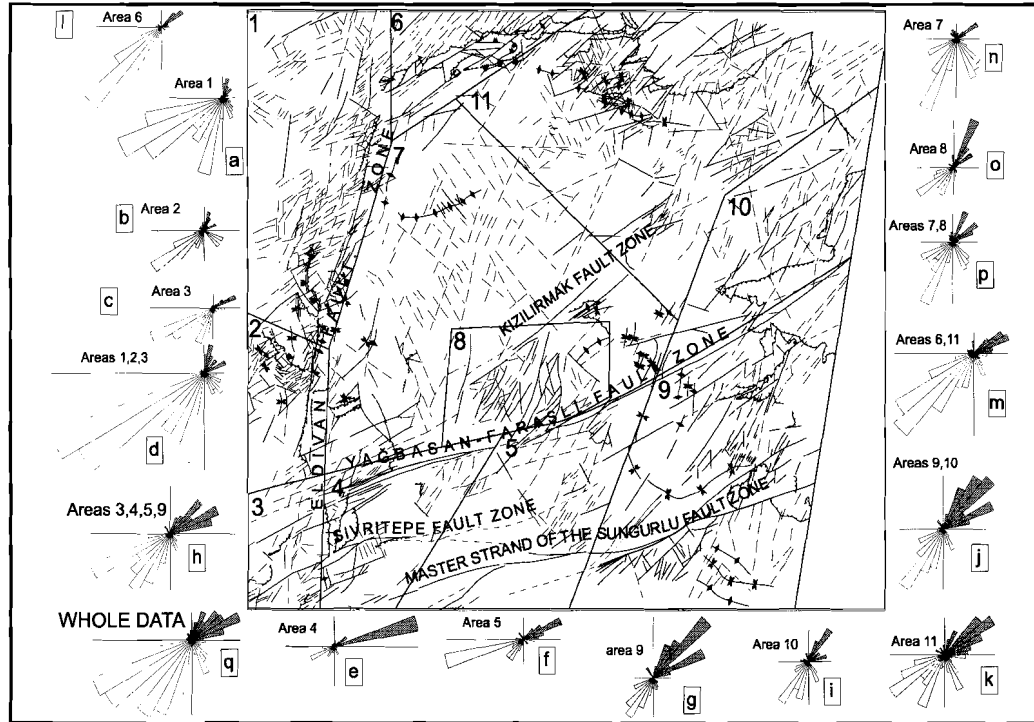
Figure 2.08 Lineament map of the Çankırı Basin. a-q) rose diagrams for each selected sub area and combinations of some sub areas. The upper quadrants of the rose diagrams display the fault classes and lower quadrants display the photo-lineament classes (see Tables 2.02 and 2.03 for the details of frequencies).
