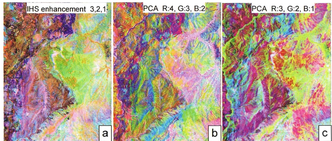
Figure 2.06 a) Image produced from the Hue-Intensity-Saturation(HIS) enhancement technique applied to the bands 1,2 and 3. B and c) Various band combinations of the Principal Component Analysis (PCA) applied to a part of the Çankırı Basin (see Figure 2.03a for the location).
