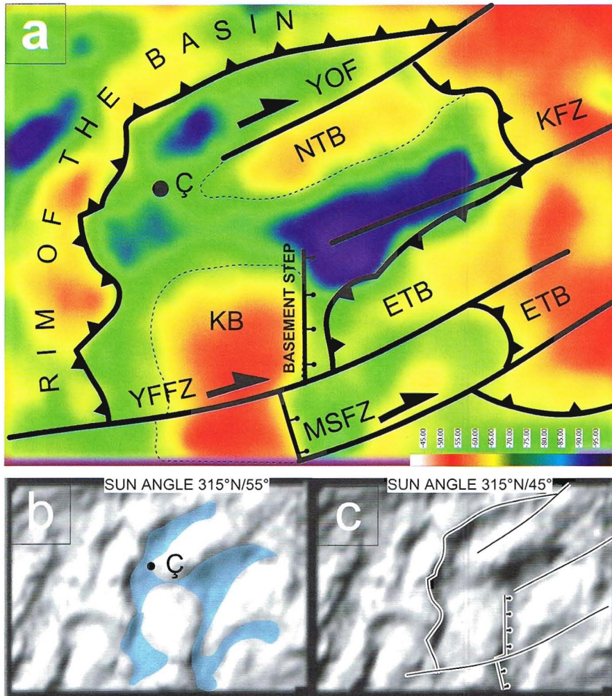
Figure 2.10 a) Gravity image of the Çankırı Basin obtained from gridding using Krigging of 2*2 km gravity data. Ç: Çankırı, ETB: eastern thrust belt, KB: Kırşehir Block, KFZ: Kızılırmak Fault Zone, MSFZ: Master Strand of the Sungurlu Fault Zone, NTB: Northern Thrust Belt, YFFZ: Yağbasan-Faraşlı Fault Zone, YOF: Yoncalı Fault Zone. b-c) pseudo-stereo pair of the shaded relief images of the gravity data (scale is 50% of a). The blue areas indicate where the basin in-fill is the thickest.
