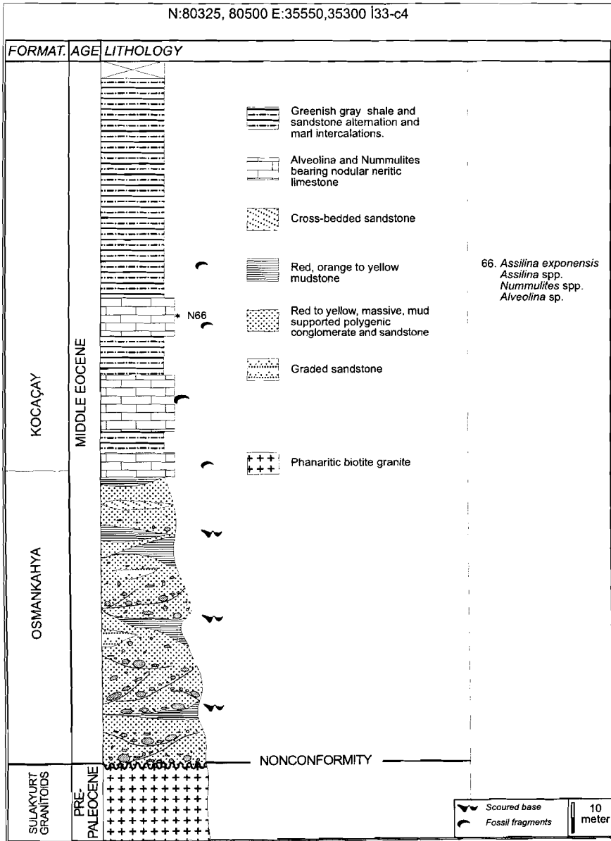
Figure 3.19 Measured stratigraphical section for the Osmankahya and the Kocaçay formations. The coordinates at the top of the figure are the beginning and ending northing (N) and easting (E) for the stratigraphic section (UTM based Turkish Grid).
