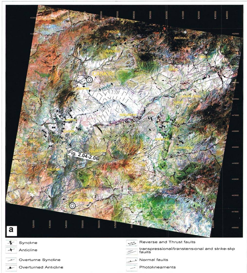
Figure 2.03 a) Landsat TM Image of the study area, major faults, folds and photo-lineaments are overlaid on the image b) resultant geological map of the study area GVP: Galatean Volcanic Province
