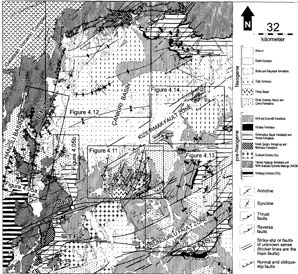
Figure 4.02 Geological map of the Çankırı Basin. EFZ: Eldivan Fault Zone, KFS: Kırıkkale Fault Set, SFMS: Master Strand of the Sungurlu fault Zone, STFZ: Sivritepe Fault Zone, YFFZ: Yağbasan-Faraçlı Fault Zone.
