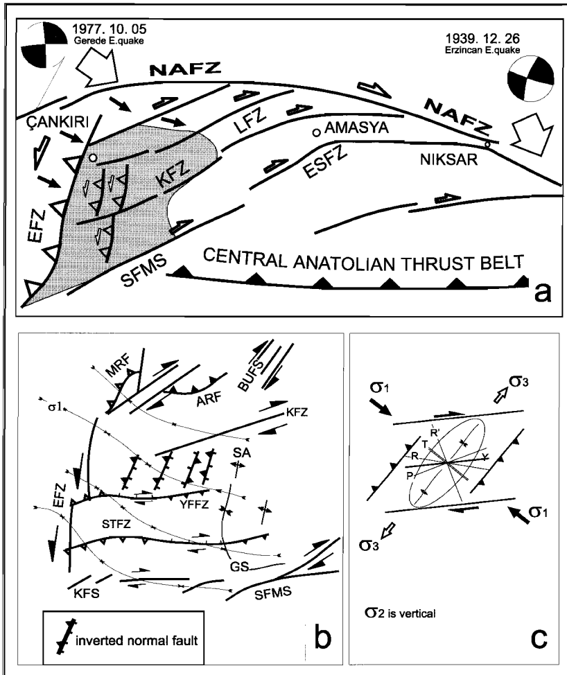
Figure 4.24 Simplified tectonic map of the active faults in the north central Turkey. ESFZ: Ezinepazarı-Sungurlu Fault Zone, KFZ: Kızılırmak Fault Zone, LFZ: Laçın Fault Zone, NAFZ: North Anatolian Fault Zone, SFMS: Master Strand of the Sungurlu Fault Zone. Large arrows are the horizontal components of the compression directions obtained from fault plane solutions of the Gerede and Erzincan Earthquakes (partly modified after Barka and Hancock 1984, Özçelik 1994, Kaymakci and Koçyiğit 1995, fault plane solutions are after Jackson and McKenzie 1984). b) Simplified structural map of the Çankırı Basin area. ARF: Ayseki reverse fault, BUFS: Bürtü Fault Set, EFZ: Eldivan fault Zone, GS: Güvendik Syncline, KFS: Kırıkkale Fault Set, MRF: Merzi Reverse Fault, STF: Sivritepe Fault Zone, YFFZ: Yağbasan-Faraşlı Fault Zone. Note transpressional and transtensional segments of the STFZ and YFFZ as the faults change their strike. c) Riedel pattern of deformation proposed for the structures developed in the latest phase of deformation (Tortonian to Recent) in the Çankırı Basin area.
