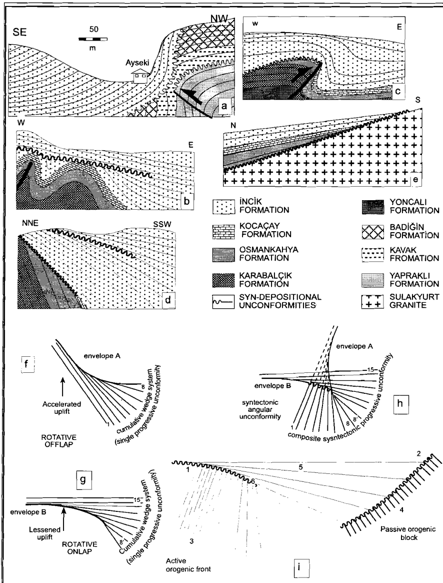
Figure 3.25 a-e) Sketch cross-sections illustrating the various types of syn-depositional (=syntectonic) unconformities observed during the field studies. f-i) Conceptual development of syn-depositional unconformities in areas where deformation and deposition are coupled. The numbers 1-5 are the time lines (adopted from Riba 1976 and Anadón (1986). See text for the discussion.
