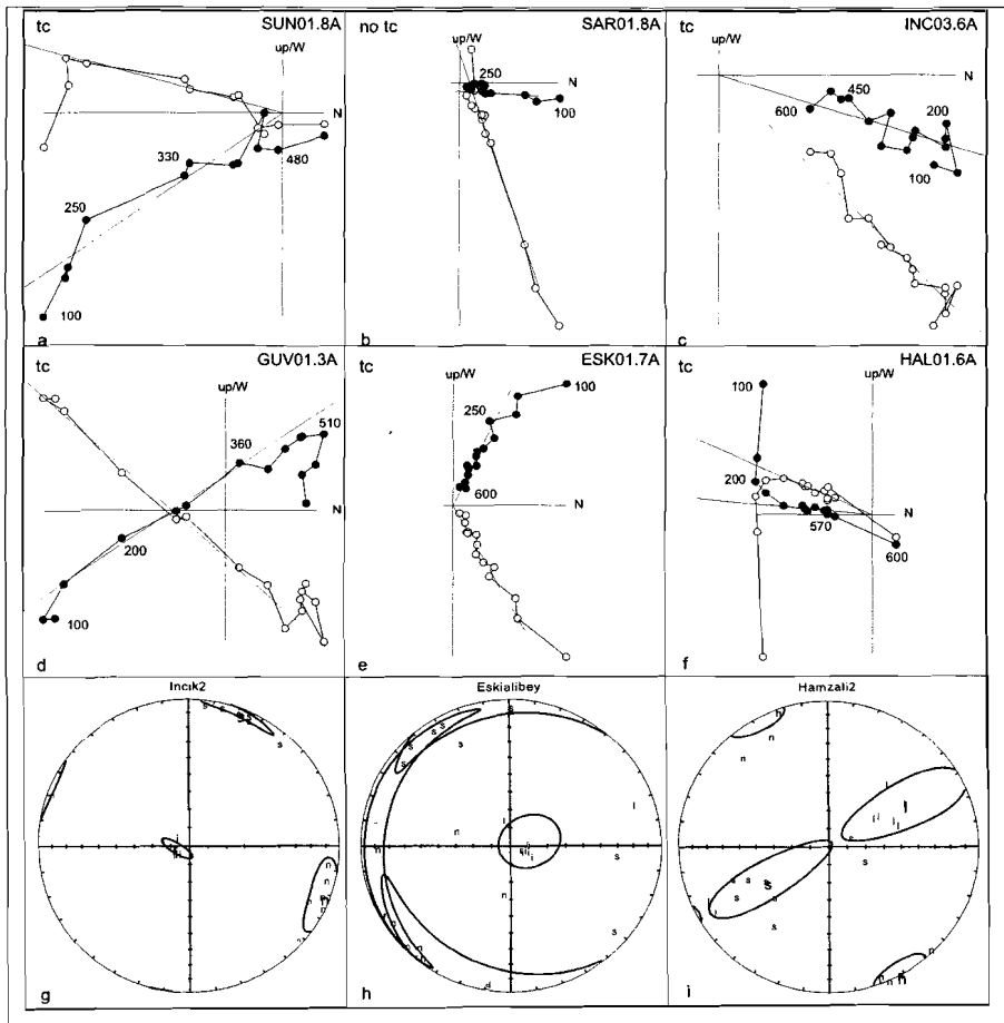
Figure 7.03 Orthogonal projections of stepwise thermal demagnetisation of selected samples from Eocene (a,b), Oligocene (c,d) and Miocene (e,f) sediments. Closed (open) circles represent the projection of the ChRM vector endpoint on the horizontal (vertical) plane. Numbers denoting temperatures in °C and tc/no tc indicates after/before bedding plane correction. g-i shows equal area projection of anisotropy of the magnetic susceptibility with circles/squares/triangles as k_{min}/k_{max}/k_{int} after bedding plane correction.
