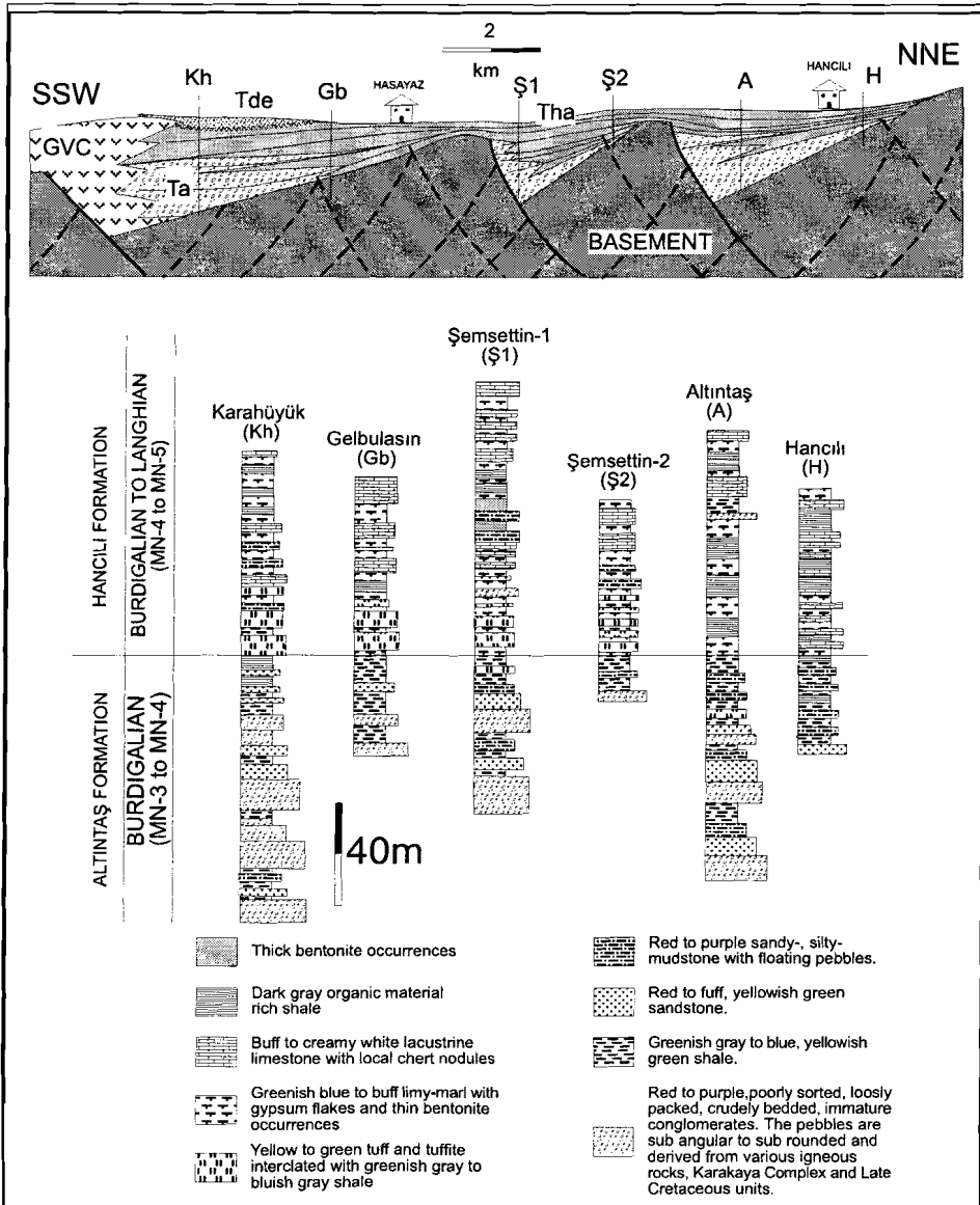
Figure 4.08 Correlation chart of the measured sections of the Altıntaş and the Hancılı formations and an interpreted sketch cross-section along an imaginary NNE-SSW line illustrating the relative positions of the measured sections (see Figure 4.05 for the locations of the measured sections). Vertical scale is 2 times exaggerated.
