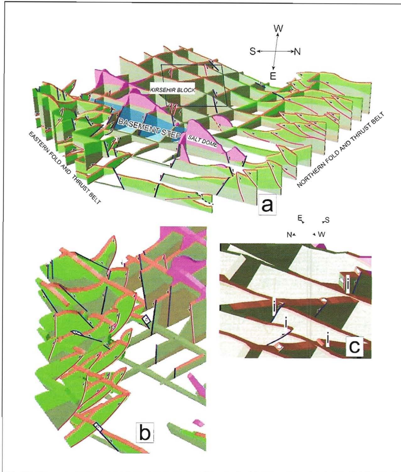
Figure 2.15 Fence diagrams of the volume model area. The units above the Kocaçay Formation are stripped-off. Note two thrust belts: one in the north and the other one in the east. Note also the basement step, which is a normal fault in the eastern part of the Kirsehir Block (a). Note also that the thrust faults (b) are displaced by a number of faults with normal off-set. These faults, in the seismic sections, appeared to be normal in nature. However, this does not exclude lateral movements which are actually observed on the surface. c) Normal and reverse faults observed in the Basement. Most of these reverse faults are inverted growth faults. Examples are indicated with "i" (see also Figure 2.16). c) blow-up image of the faults developed on the basement (looking to the NE)..
