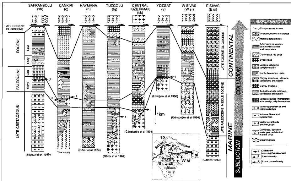
Figure 8.08 Correlation chart for the major Tertiary basins located within and around the Kırşehir Block. Note relatively younging of unconformable bottom contacts of Early Tertiary units in the Safranbolu and Çankırı Basins indicated with U and LU. Note also the Late Cretaceous to Tertiary continuous sedimentation in all of the Basins (with local unconformities) except in the Tuz Gölü, Central Kızılırmak, Çankırı and Yozgat basins, which have unconformable relations with the Kırşehir Block (indicated with 1).
