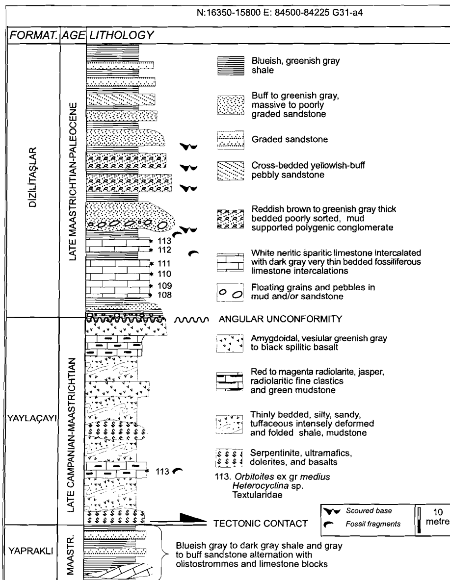
Figure 3.06 Measured stratigraphical section for the Yaylaçayı and Dizilitaşlar formations. The coordinates at the top of the figure are the beginning and ending northing (N) and easting (E) for the stratigraphic section (UTM based Turkish Grid).
