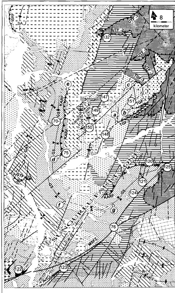
Figure 6.11 Geological and sample location (site) map of the sub-area 7 (see Figure 6.04 for the description of the units).
