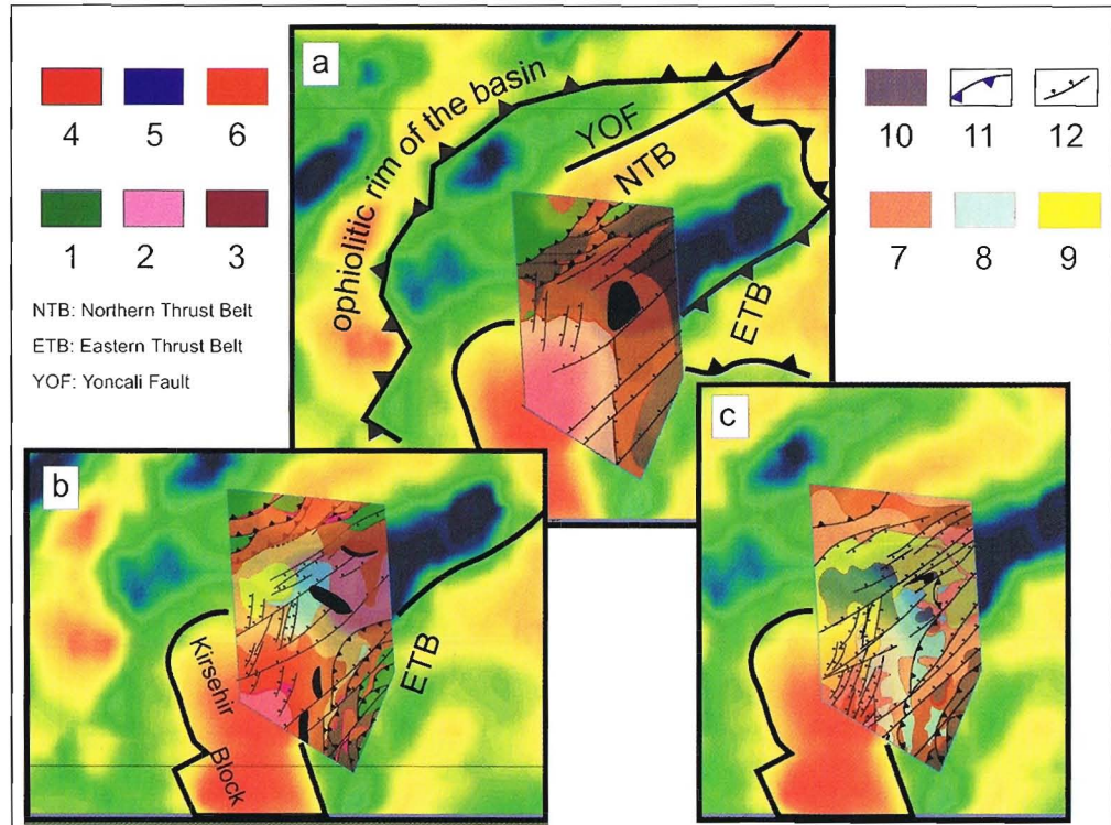
Figure 2.17 Overlay maps of gravity anomaly image and the time section maps (semi transparent). Note the coincidence of outline of the Kırşehir Block in the gravity image and the 3.50s map (a). Note also, alignment and positions of the salt bodies (a and b). 1. Late Cretaceous units, 2. Kırşehir Block, 3. Tertiary clastics, 4. Kocaçay Formation, 5. Salt bodies, 6. lower part of the Incik Formation, 7. upper part of the Incik Formation, 8. Oligocene Güvendik formation, 9. Middle Miocene to Tortonian units, 10. Late Miocene units, 11. thrust faults, 12. normal faults.
