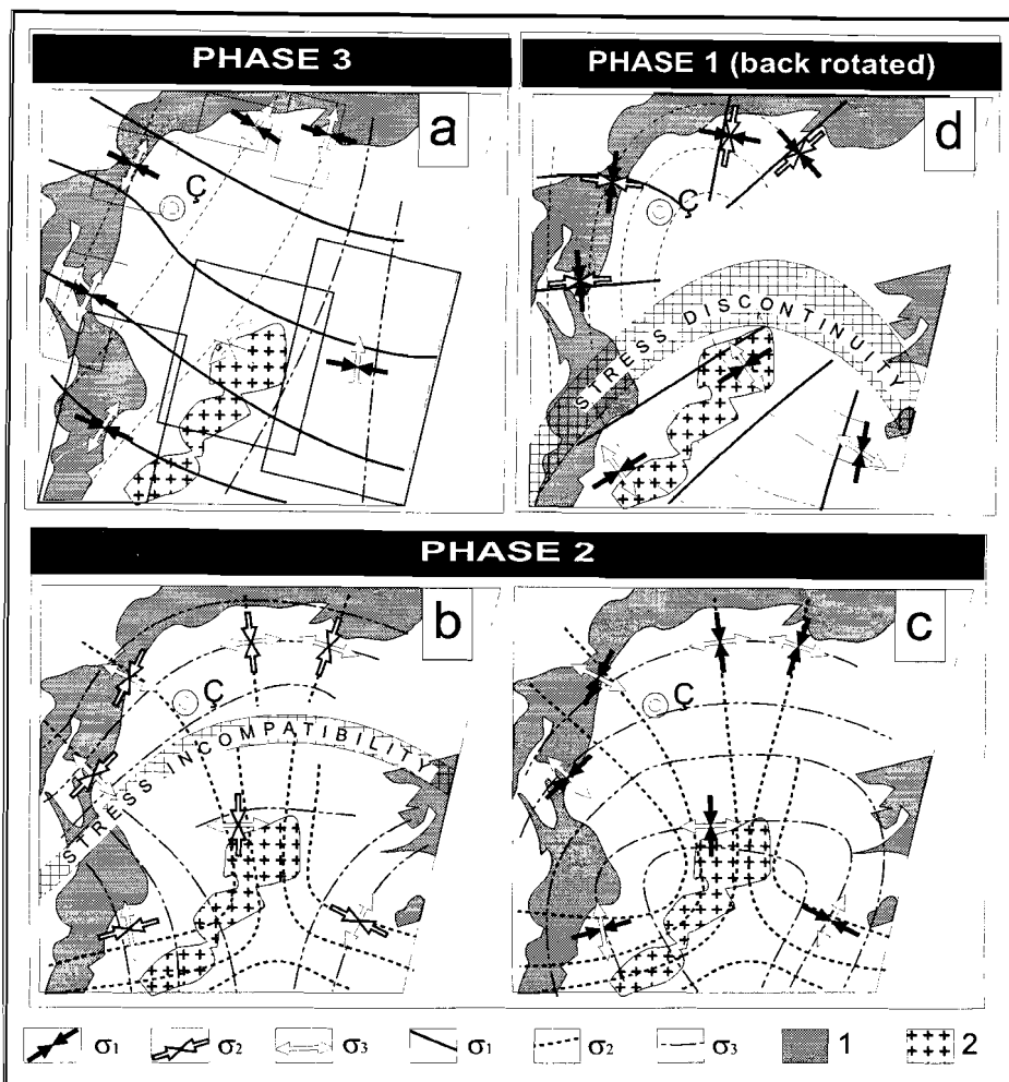
Figure 6.17 Integrated smoothed trajectories of horizontal components of principal stress for each deformation phase. Note that only concentric pattern of \sigma_3 (c) for the deformation phase 2 is compatible with the northern area (i.e. sub-areas 1-4). 1: ophiolitic rim of the Çankırın Basin, 2: granitoids of the Kırşehir Block. Ç: Çankırın.
