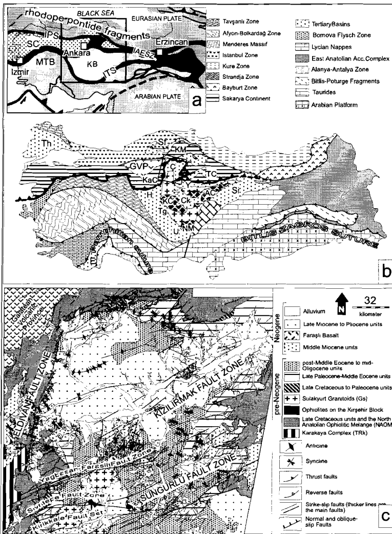
Figure 8.02 a) Main tectonic units of Turkey (after Şengör et al. 1984). Black areas are the oceanic domains. IAESZ: Izmir-Ankara-Erzincan Suture Zone, IPS: Intra-Pontide Suture, ITS: Inner-Tauride Suture, KB: Kırşehir Block, SC: Sakarya Continent, b) Isopic zones and main Tertiary basins of Turkey (modified after Şengör and Yılmaz 1981, Şengör et al. 1984, Okay et al. 1996). Th: Thrace Basin, Sf: Safranbolu Basin, Ç: Çankırı Basin, GVP: Galatean Volcanic Province, Ck: Central Kızılırmak Basin, H: Haymana Basin, Tg: Tuzgözü Basin, U: Ulukışla Basin, Si: Sivas Basin, E: Elmalı Basin, KaC: Karakaya Complex, KM: Kargı Massif, TC: Tokat Complex. AC: Akdağmadeni Massif, KC: Kırşehir Metamorphics, NM: Niğde Massif. c) Simplified Geological map of the Çankırı Basin.
