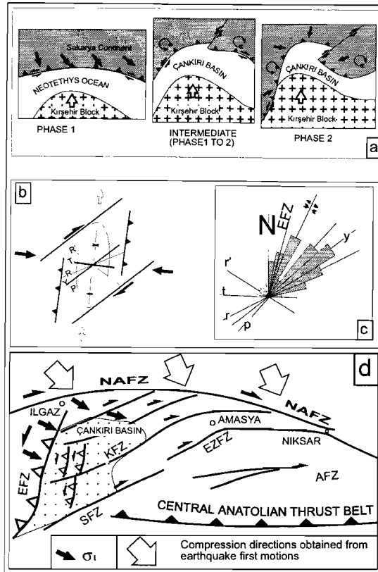
Figure 5.13 a) Cartoons illustrating the possible development of the Çankırı Basin through deformation phase 1 to 2. Note block rotations and response of principal stress orientations as the Kirşehir block drives northwards. b) Riedel pattern of deformation (after Biddle and Christie-Blick 1985) and plot of horizontal components of the \sigma_1 (convergent large arrows) proposed to explain the structures developed in the deformation phase-4. c) Length weighted rose diagram prepared from the structures proposed to have been developed in this phase and corresponding Riedel shears. r , synthetic-shear, r' , antithetic-shear, p , secondary synthetic-shear, y , principal displacement zone, t , extension fractures. Note that the orientation of the Eldivan Fault Zone (EFZ) with respect to the riedel shears. d) Schematic illustration of the structures in north-central Turkey plotted to explain the structural development of the Çankırı Basin during the deformation phase 4. AFZ: Almus Fault Zone, EFZ: Eldivan Fault Zone (which is the WBCB-western boundary fault of the Çankırı Basin), EZFZ: Ezinepazarı Fault Zone, KZF: Kızılırmak Fault Zone, NAFZ: North Anatolian Fault Zone (modified after Barka and Hancock 1984, Şengör et al. 1985).
