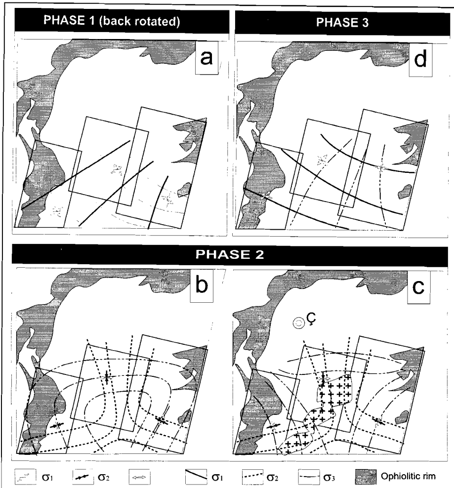
Figure 6.16 Smoothed trajectories of horizontal components of principal stresses for the southern part of the Çankırı Basin. Note that for the deformation phase 2 \sigma_3 has two possible patterns while keeping the \sigma_2 pattern fixed (see text for the discussion).
