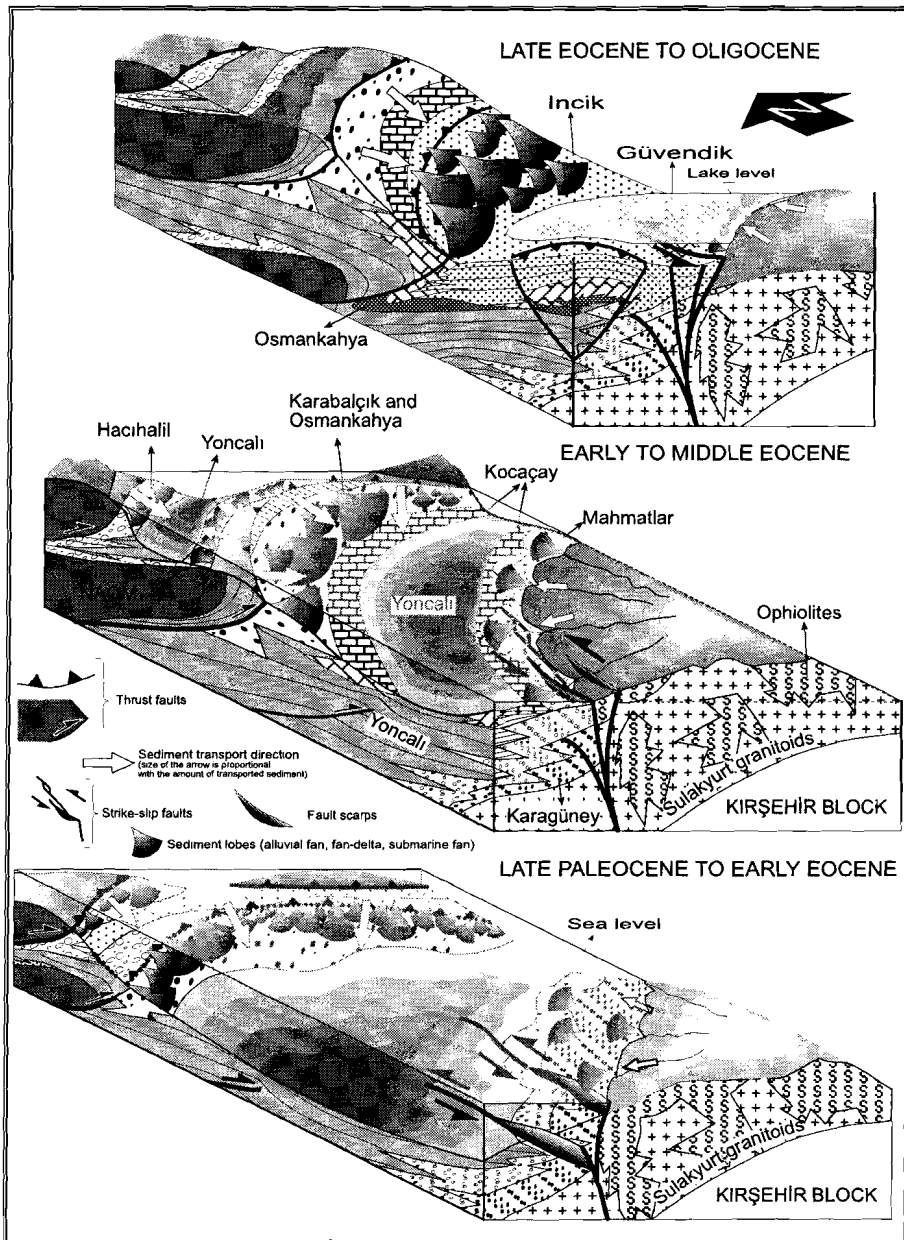
Figure 3.28 Block diagrams illustrating the Late Paleocene to Oligocene evolution of the Çankırı Basin. See text for the explanations.
