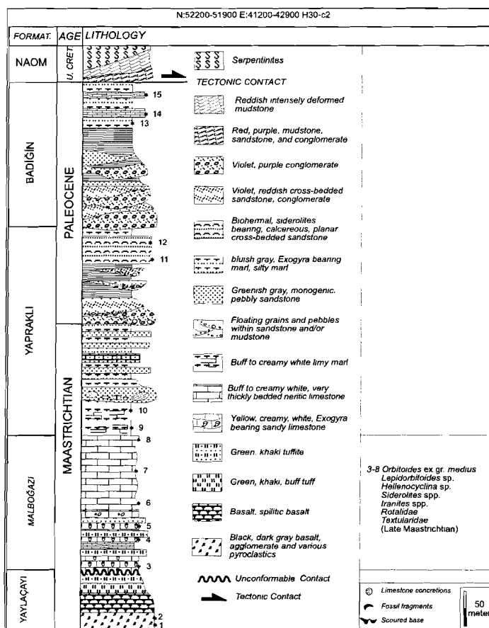
Figure 3.09 Measured stratigraphical section for the Malboğazi, Yapraklı and Badiğın formations. The coordinates at the top of the figure are the beginning and ending northing (N) and easting (E) for the stratigraphic section (UTM based Turkish Grid).
