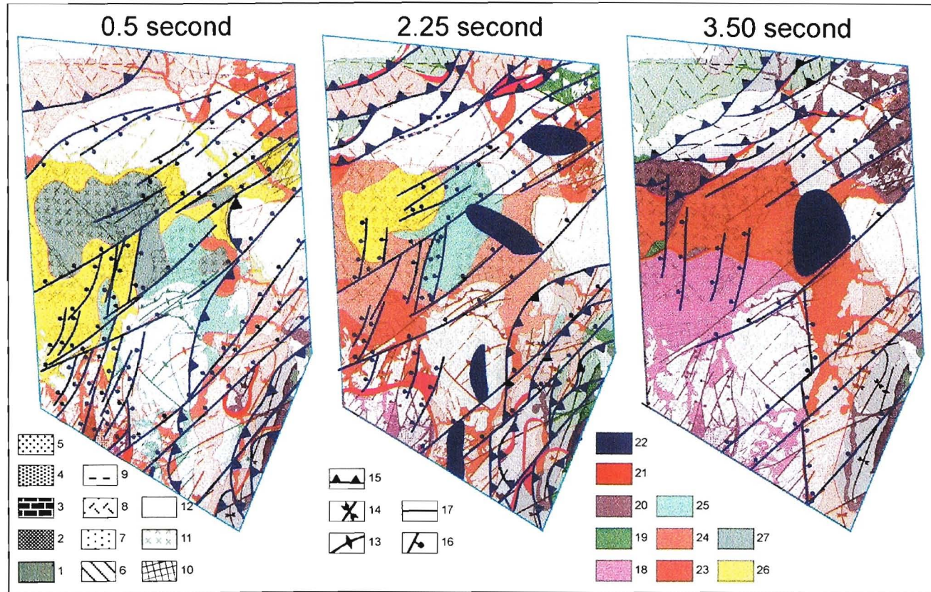
Figure 2.18 Overlay maps of the surface geology and time section maps. KFZ: Kızılırmak Fault Zone, YFFZ: Yağbasan-Faraşlı Fault Zone. 1-12 are the units recognized on the surface geologic map indicated with patterns. 1. NAOM, 2. Late Paleocene to Middle Eocene units, 3. Kocaçay Formation, 4. lower part of the Incik Formation, 5. upper part of the Incik Formation, 6. Oligocene Güvendik formation, 7. Early to Middle Miocene Çandır Formation, 8. Middle Miocene (?) Faraşlı Basalt, 9. Tortonian Tuğlu formation, 10. Late Miocene Suleymanlı formation, 11. Late Miocene Bozkır Formation, 12. Quaternary Alluvium, 13. anticline, 14. syncline, 15. thrust/reverse faults, 16. normal faults, 17. strike-slip faults and faults with undetermined sense of movement. 18-27 are the units recognized on the seismic sections indicated with colors. 18. Kırşehir Block, 19. Late Cretaceous units, 20. Tertiary clastics, 21. Kocaçay Formation, 22. salt bodies, 23. lower part of the Incik Formation, 24. upper part of the Incik Formation, 25. Oligocene Güvendik formation, 26. Middle Miocene to Tortonian units, 27. Late Miocene and younger units.
