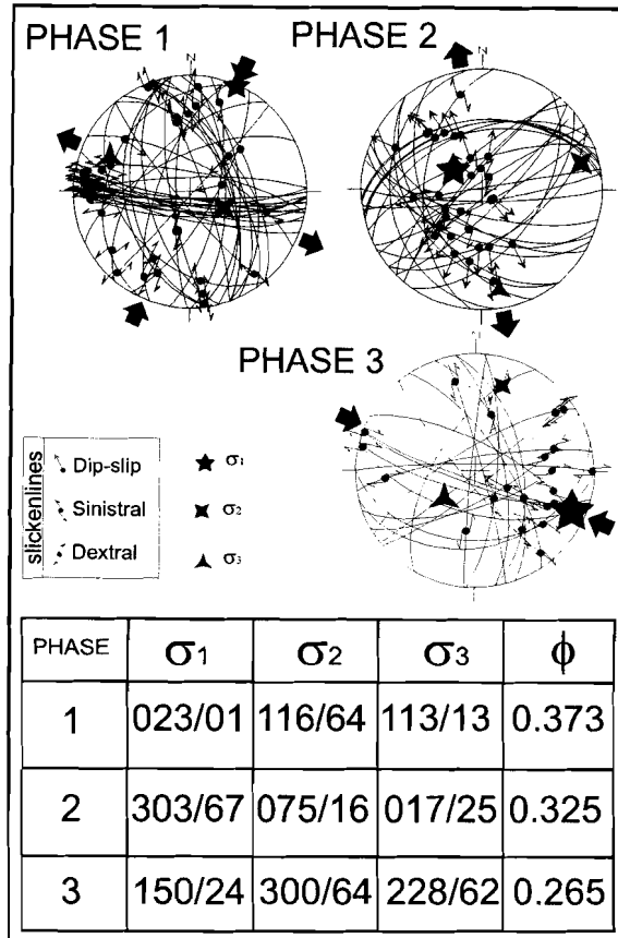
Figure 6.07 Plots of fault planes, slickenlines and stress orientations for the whole data, in sub-area 5, for each deformation phase.
