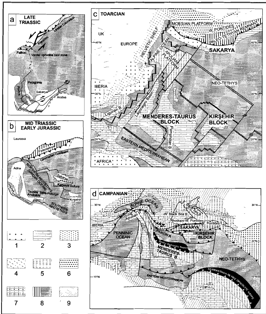
Figure 8.01 Some selected published paleogeographic reconstructions of the Eastern Mediterranean Tethys after: a) Robertson and Dixon (1984), b) Şengör et al. (1984), c-d) Channel et al. (1996). Apart from the paleogeographic positions of the continental fragments, the main difference between these models is the polarity of the subduction of the Permo-Triassic Tethys oceanic crust (Paleotethys). Note the locations of the Sakarya Continent and of the Kirşehir Block. 1. exposed continental basement, 2. carbonate platform, 3. continental deposits, 4. mixed shelf environment, 5. deep shelf, 6. marginal marine, 7. restricted carbonate platform, 8. deep sea, 9. continental crust (in a and b).
