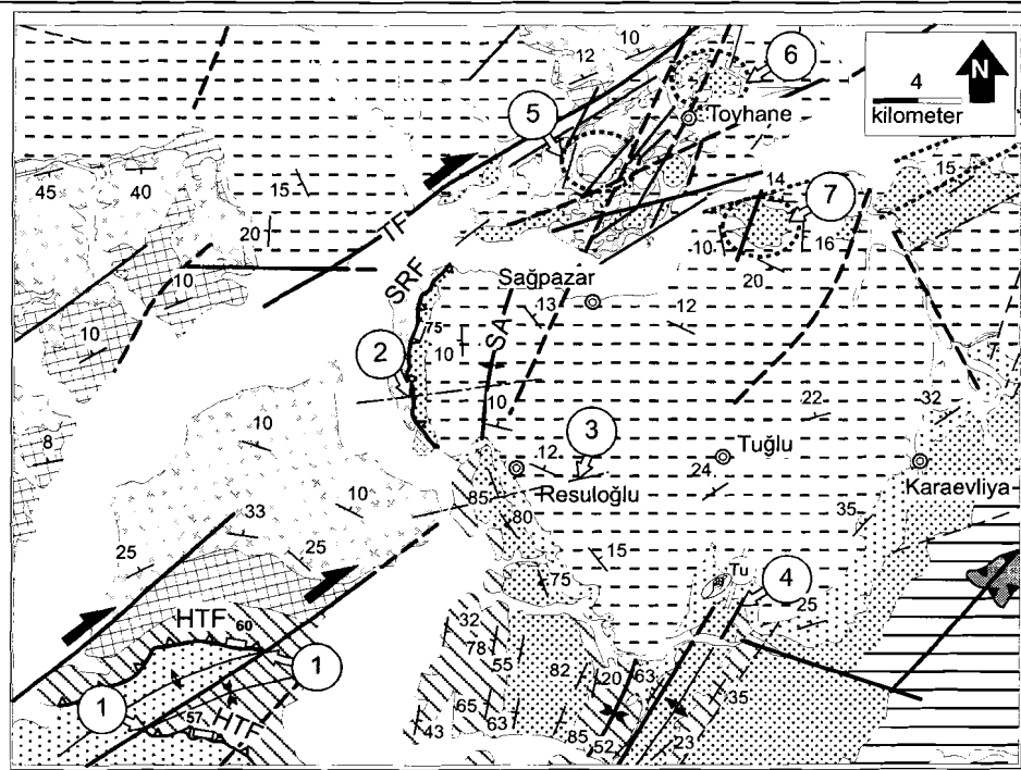
Figure 4.14 Geological map of the north-eastern margin of the Çankırı Basin ( see Figure 4.05 for the explanation of the symbols).
