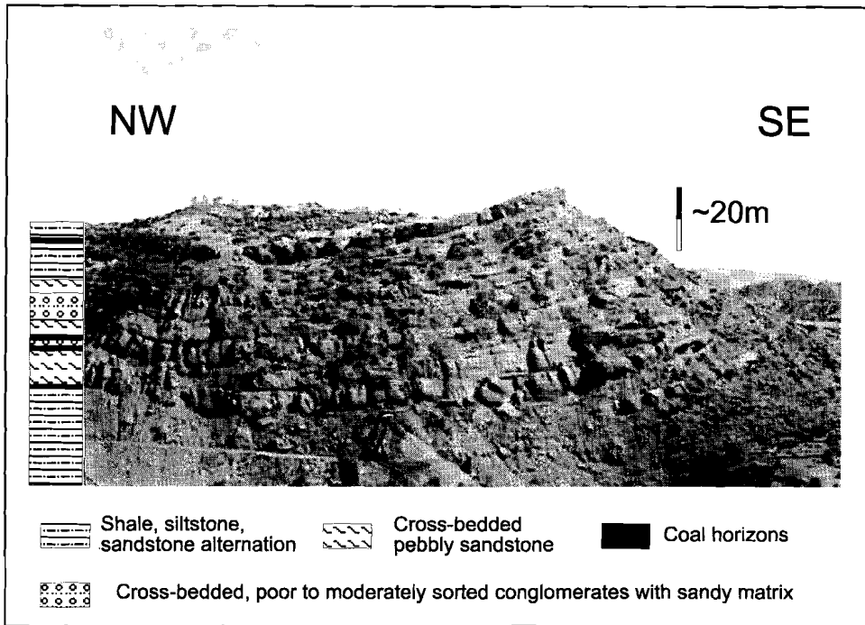
Figure 3.16 Photograph of upper coal bearing parts of the Karabağlık Formation in the northern part of the Çankırı Basin (Location is around N:07065, E:95300 G32-d2 quadrangle, view to NE).
