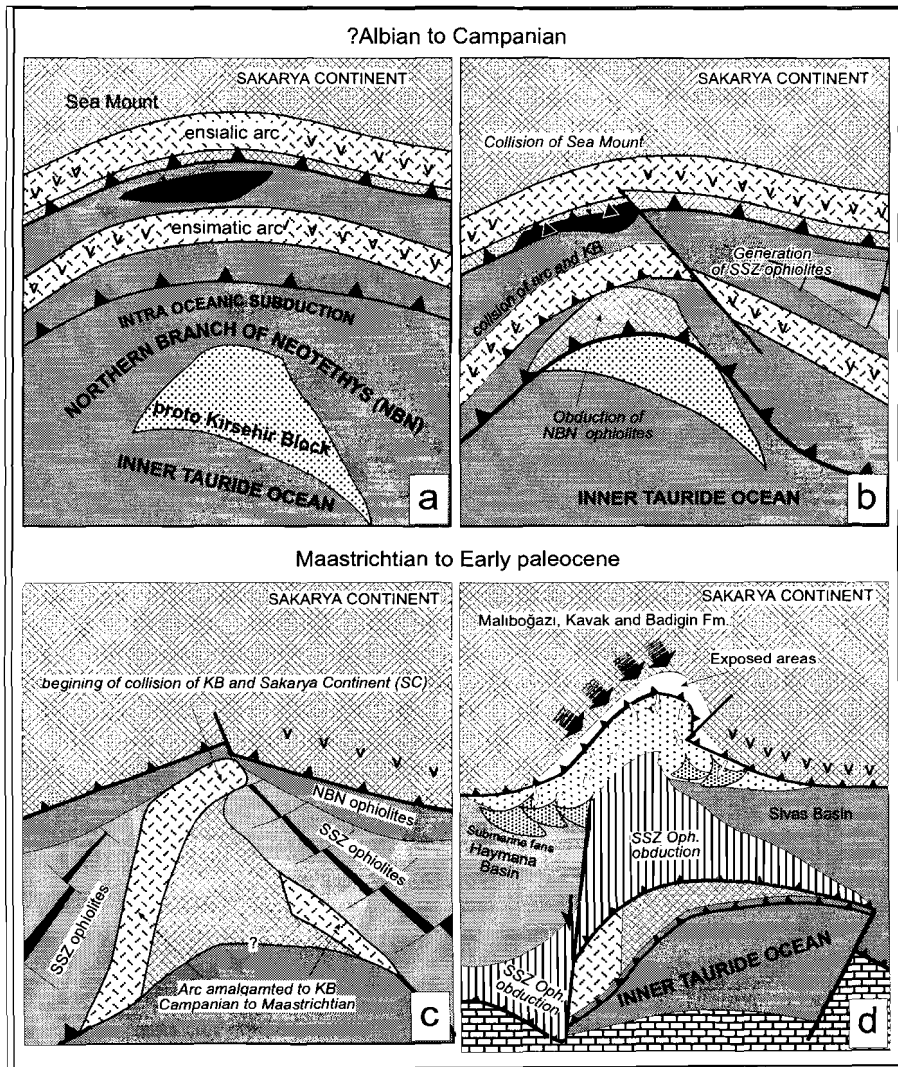
Figure 8.07 Paleogeographic reconstructions for the evolution of the Sakarya Continent and the Kırşehir Block together with the intervening areas. (a-b) based on Gökten (1983), Görür et al. (1984), Okay (1984, 1992), Gönçüoğlu et al. (1991, 1992, 1993, 1994), Özcelik (1994), Tüysüz et al. (1995), Yalınız et al. (1996). Anticlockwise rotation of the Kırşehir Block is based on Sanver and Ponat (1980). Collision of the ensimatic arc and the Kırşehir Block, and supra subduction zone ophiolite (SSZ) generation and their obduction is based on Yalınız et al. (1996), Yalınız (1997) and Gönçüoğlu et al. (2000). The areas in the south, south-east and south-west of the Kırşehir Block are after Görür et al. (1984) and Okay (1984, 1992). See text for the discussion.
