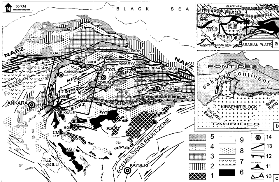
Figure 3.01 a) Inset map showing the geological outline of the Eastern Mediterranean area (Modified after Şengör et al. 1984). BSZ: Bitlis-Zagros Suture, IAESZ: Izmir-Ankara-Erzincan Suture Zone, ITS: Intra-Tauride Suture, KB: Kırşehir Block, MTB: Menderes-Taurus Block, SC: Sakarya Continent. b) Tectonic setting of the Çankırı Basin. c) Tectono-stratigraphical map of Central Anatolia. Box shows the location of the Çankırı Basin. AFZ: Almus Fault Zone, ESFZ: Ezinepazari-Sungurlu Fault Zone, KFZ: Kızılırmak Fault Zone, LFZ: Laçın Fault Zone, NAFZ: North Anatolian Fault Zone, YFFZ: Yağbasan-Faraşlı Fault Zone. AG: Ağaçören granitoids, BM: Baranadağ Monzonite, CM: Cefalıkdağ Quartz-Monzonite, SG: Sulakyurt Granitoids, YG: Yozgat Granitoids. 1. Pre-Late Cretaceous metamorphic basement of the Kırşehir Block, 2. Pre-Jurassic metamorphic basement of the Sakarya Continent, 3. Triassic Karakaya Complex, 4. Jurassic-Cretaceous platform carbonates on the Sakarya Continent, 5. Late Cretaceous (?) ophiolites and ophiolitic melanges, 6. Pre-Paleocene granitoids of the Kırşehir Block, 7. Galatean Volcanic Province (GVP, Toprak et al. 1996), 8. Paleogene units (mainly marine), 9. Neogene and Quaternary cover, 10. reverse faults, 11. thrust faults, 12. normal faults, 13. strike-slip faults and faults with unknown sense of movement, 14. major towns (modified after Barka and Hancock 1984, Görür et al. 1984, Özçelik 1994, Kaymakci and Koçyiğit 1995).
