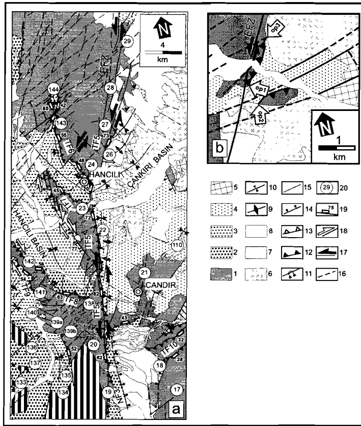
Figure 5.09 a) Geological map and sample location for the sub-area 4. EFZ: Eldivan Fault Zone, O.P. observation point (see text). 1. NAOM, 2. Altıntaş and Kılçak formations, 3. Hancılı Formation, 4. Candır Formation. 5. Süleymanlı formation, 6.Bozkır Formation, 7.Deyim Formation, 8. Alluvium, 9. anticline, 10. syncline, 11.overtumed syncline, 12. thrust faults, 13. reverse faults, 14. faults with normal sense of movement , 15. strike-slip or faults with unknown sense of movement, 16. photo-lineaments, 17. faults with sinistral strike-slip sense of movement, 18. faults with dextral strike-slip sense of movement, 19. dip amount of faults where they are best observed in the field. 20. sample site locations. b) Map showing the relation between thrusting of NAOM onto the Candır Formation and covering of the fault contact by the Bozkır Formation (see Figure 5.02 for the location of the map). Plots of fault planes, slickenlines and stress orientations for each site (c-f) and whole data in a particular phase and sub-area (g-j) (lower hemisphere equal area projection).
