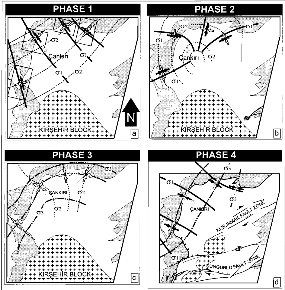
Figure 5.12 Interpreted and smoothed stress trajectories for each deformation phase.
