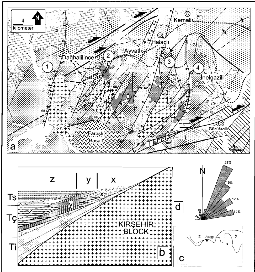
Figure 4.11 a) Geological map of the central part of the Çankırı Basin (see Figure 4.02 for its location). b) Schematic illustration of the interpreted cross-section of the facies (x,y,z) of the Çandır Formation, in which grain size decreases from x to z (x: conglomerate dominated, y: sand dominated and z: shale dominated), c) Simplified map of facies (x,y,z) distribution of the Çandır Formation. d) Length weighted rose diagram of the faults that displace the granitic basement and the Çandır Formation, percentages indicate the length frequency of the faults (see Figure 4.05 for the explanation of the symbols).
