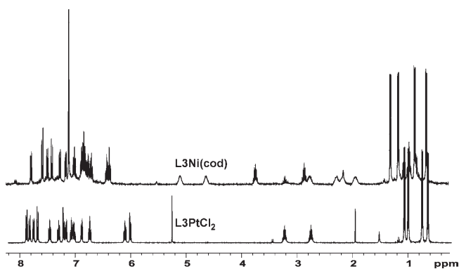
Figure 3. 1 H NMR spectra of L3PtCl 2 ( \text{CDCl}_3 ) and L3Ni(cod) ( \text{C}_6\text{D}_6 ).
