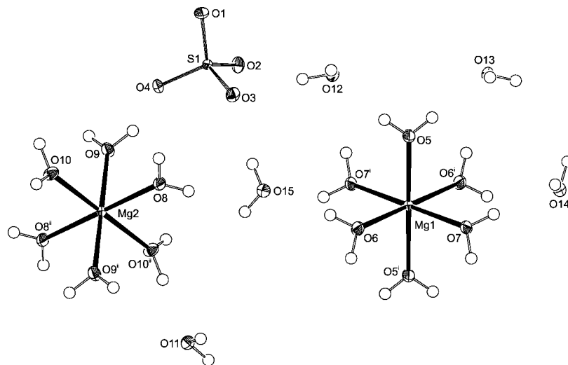
Figure 4. Displacement ellipsoid plot of [\text{Mg}(\text{H}_2\text{O})_6](\text{SO}_4)\cdot 5\text{H}_2\text{O} , drawn at the 50% probability level. Symmetry operations i: 1-x, 1-y, 1-z ; ii: 1-x, 1-y, -z .
