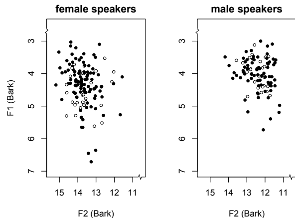
Figure 1: Formant frequencies of F_2 and F_1 in Bark units, in /i/ vowel tokens, broken down by speaker sex and by semantic category (filled symbols: smile-related, open symbols: control).
