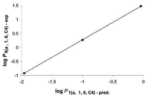
Figure 6. Prediction of \log P_{6(a, 1, 6, C4)}^{4g} in FC-72/MeOH at room temperature from \log P_{1(a, 1, 6, C4)}^{\text{pred}} in PFMCH/toluene at 0 °C.
